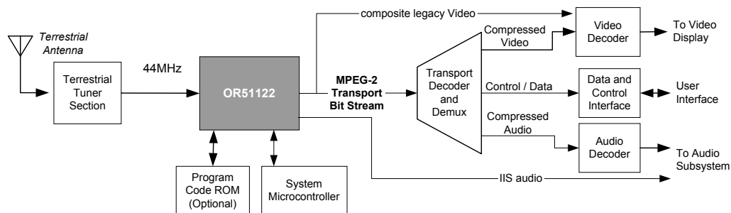
Figure 1: Application of the OR51122 in Typical Legacy/Digital TV Receiver
