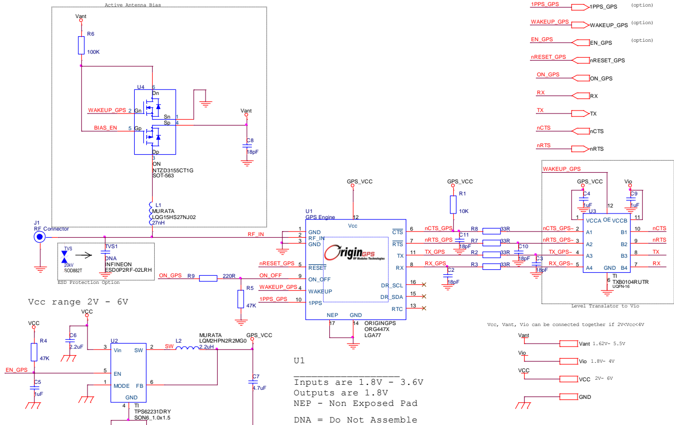
Figure 7-10: Active Antenna and UART interface circuit
