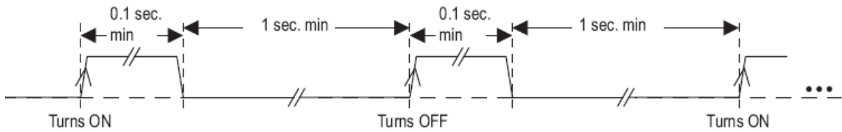
Figure 7-1: ON_OFF timing
