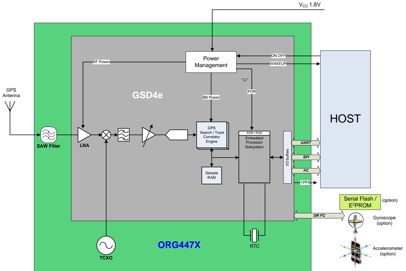
Figure 2-1: ORG447X architecture
