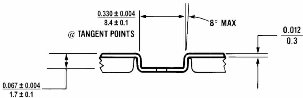
Figure 11-1: Carrier \frac{\text{inch}}{\text{millimeter}}
