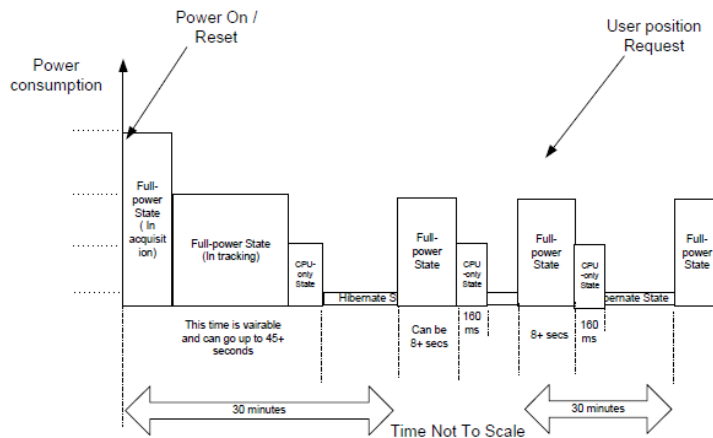
Figure 5-2: PTF™ timing
