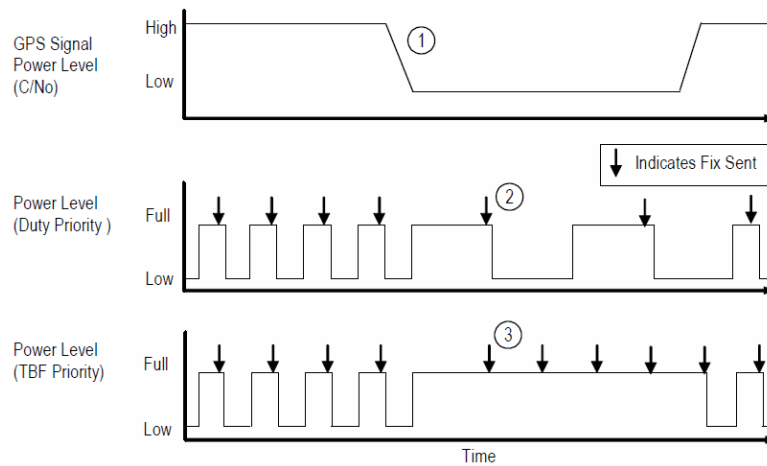
Figure 5-2: APM™ timing
