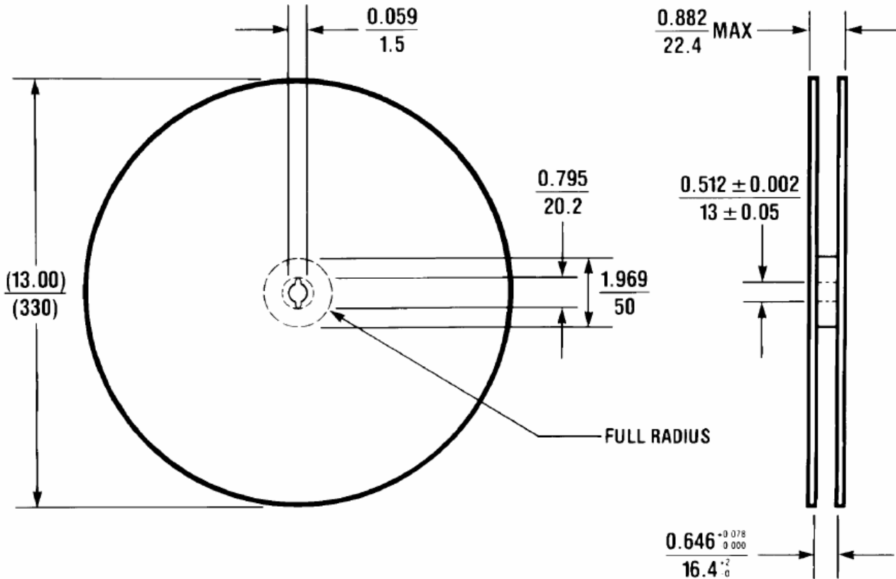
Figure 11-3: Reel \frac{\text{inch}}{\text{millimeter}}
