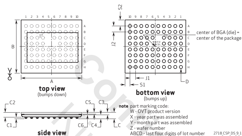
figure 9-1 package specifications
