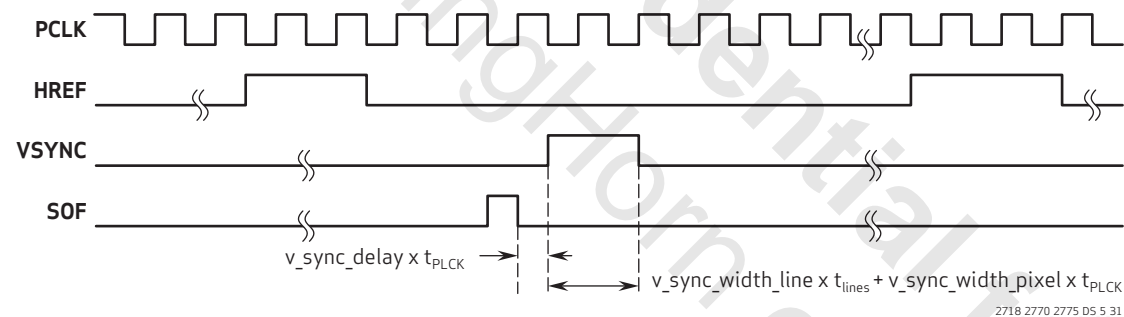
figure 5-16 DVP diagram
