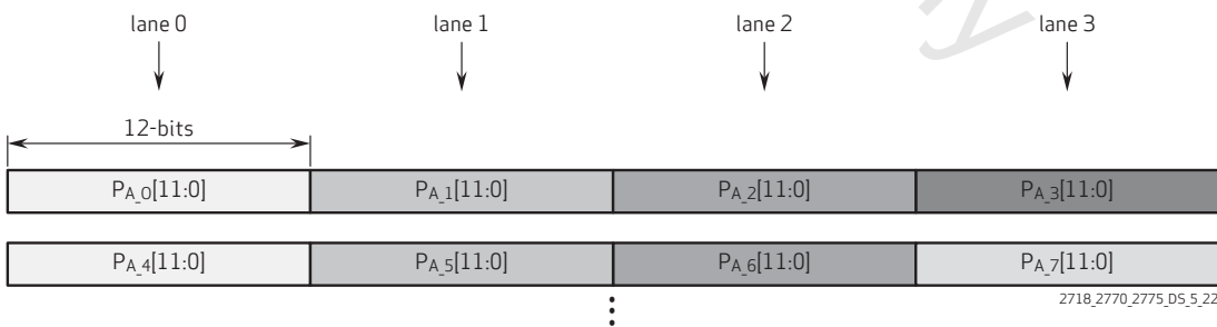
figure 5-12 12 bits linear mode diagram
