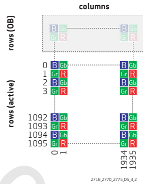
figure 3-2 pixel array region color filter layout
