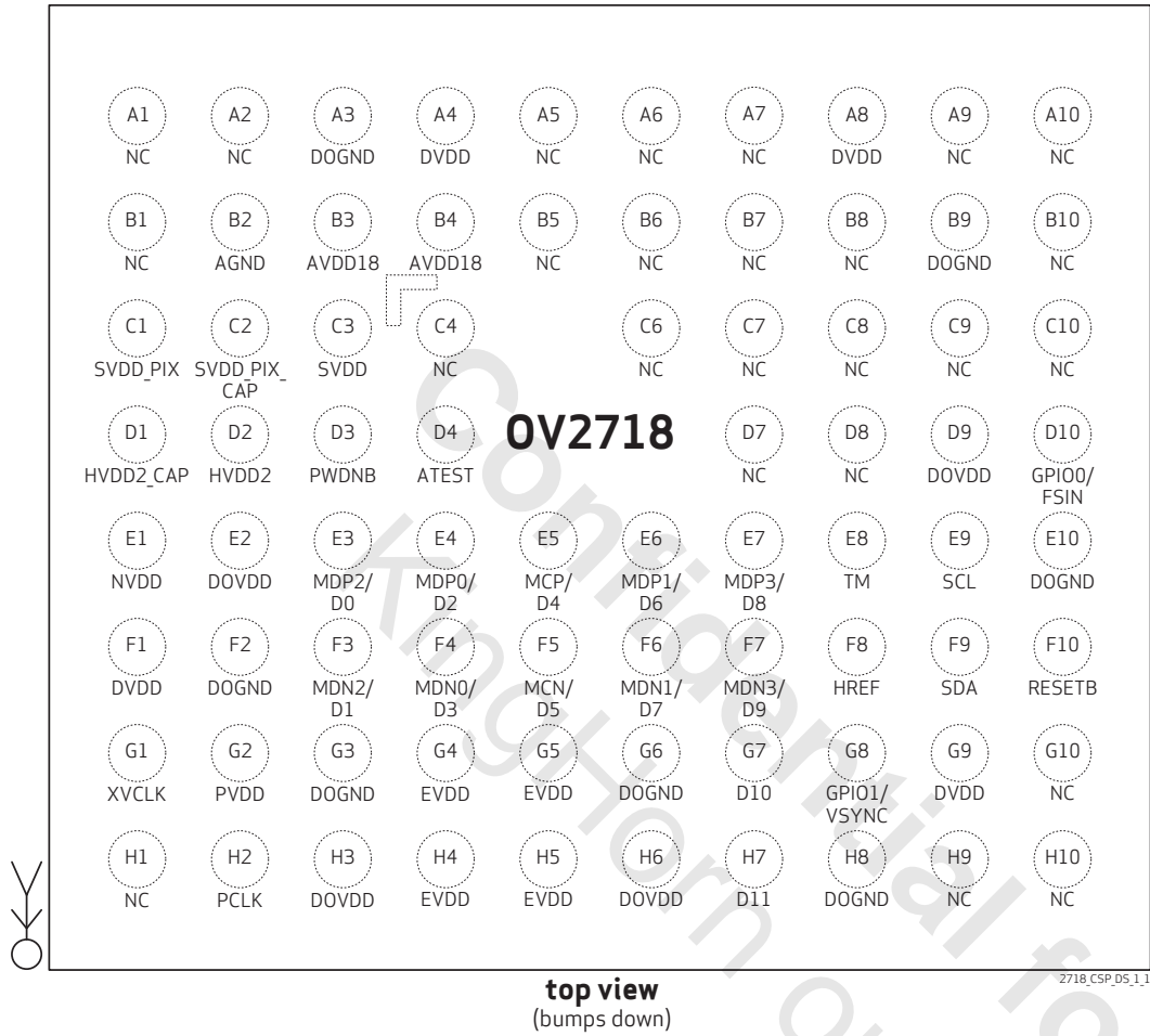
figure 1-1 pin diagram
