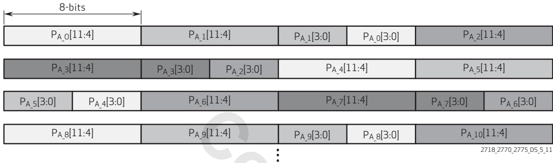
figure 5-6 12b linear mode diagram
