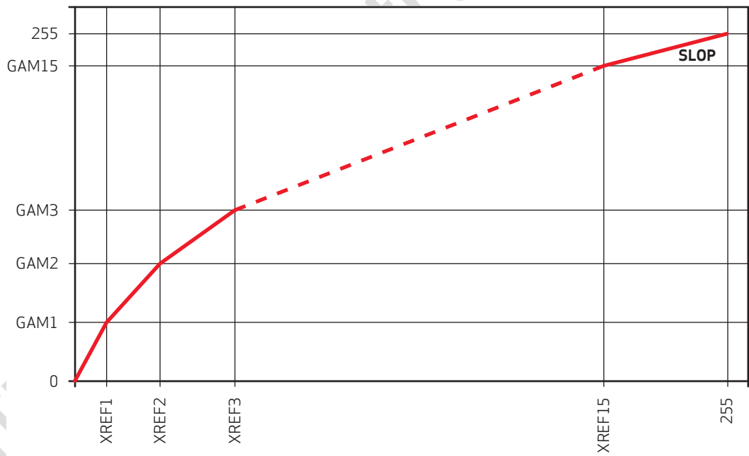
figure 5-1 gamma curve
