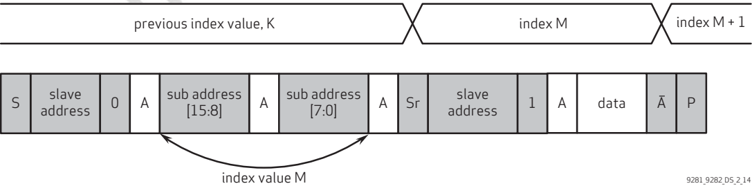
figure 2-14 SCCB single read from random location
