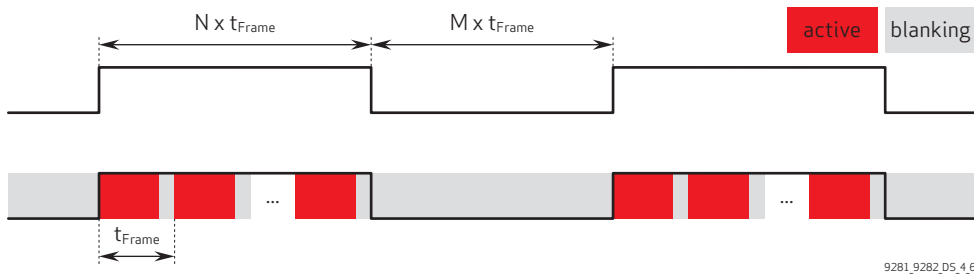
figure 4-6 low frame rate mode timing
