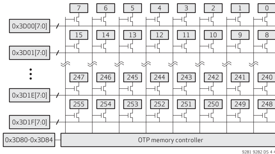
figure 4-4 OTP access
