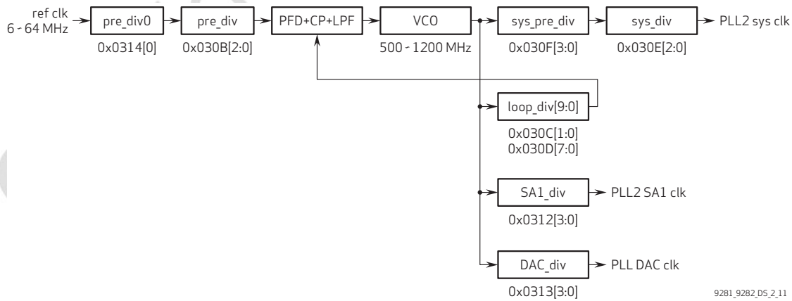
figure 2-11 PLL2 clock diagram
