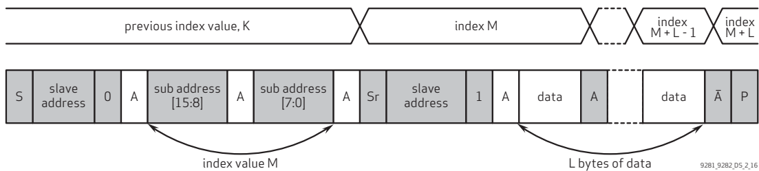
figure 2-16 SCCB sequential read from random location
