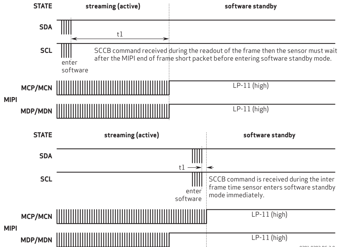
figure 2-9 standby sequence
