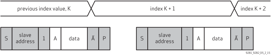
figure 2-15 SCCB single read from current location
