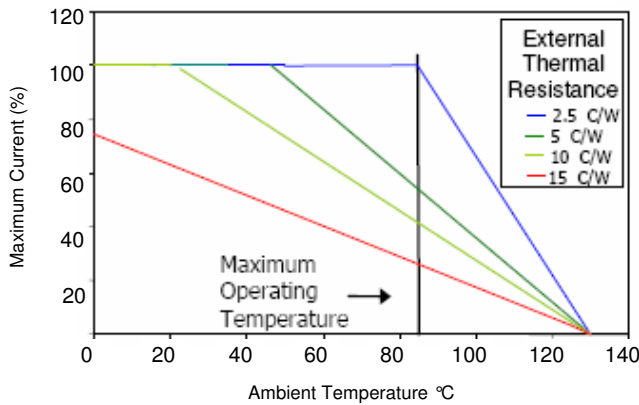
Derating Curves - Blue, Green and White LEDs
