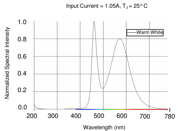
Wavelength Characteristics
