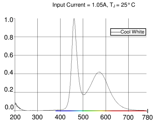
Wavelength Characteristics
