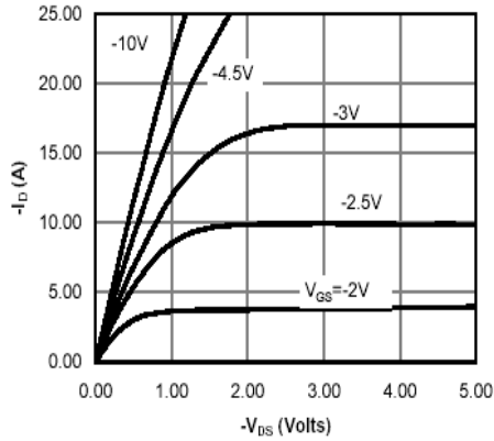
Fig 1: On-Region Characteristics
