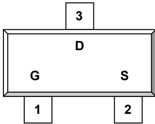
1.Gate 2.Source 3.Drain
