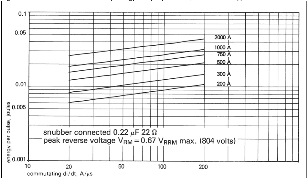
Figure 15 - Maximum reverse recovery energy loss per pulse at T j = 125°C and V rrm = 804 volts
