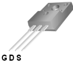
TO-220F
