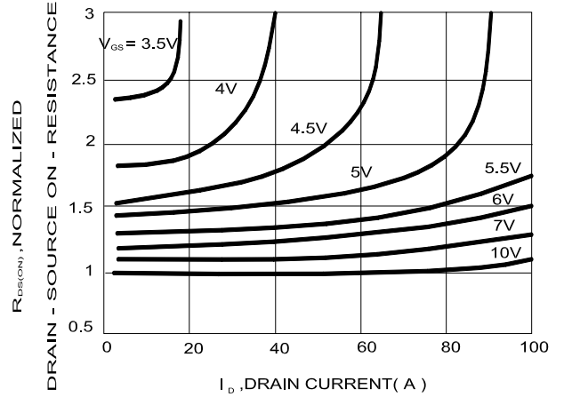
ON-RESISTANCE VARIATION WITH GATE-TO-SOYRCE VOLTAGE
