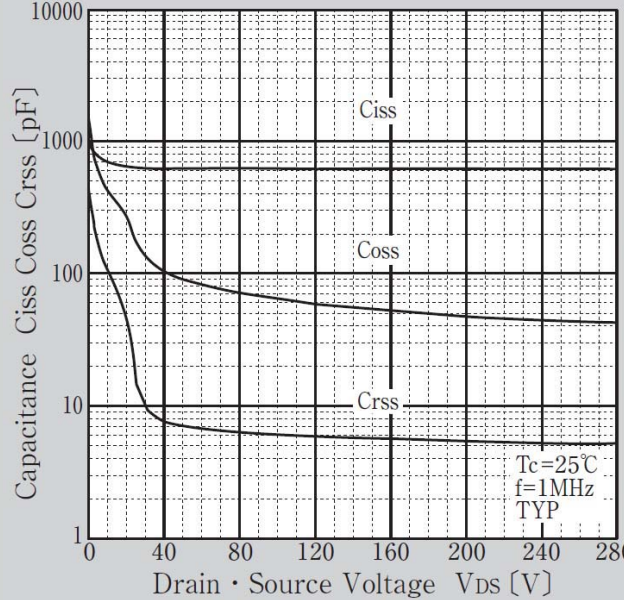
Capacitance Characteristics
