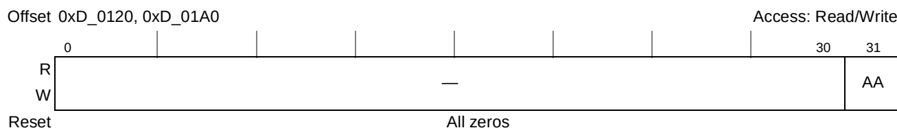
Figure 15-45. Port n Pass-Through/Accept-All Configuration Register (PnPTAACR)
