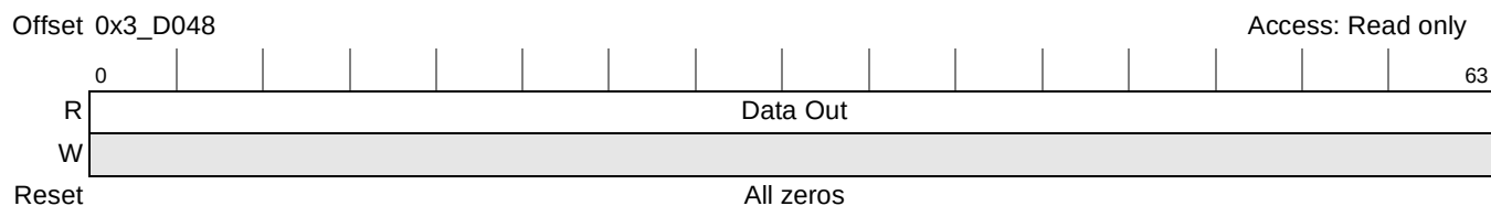
Figure 20-114. STEU Data Out Register (f9 MAC)
