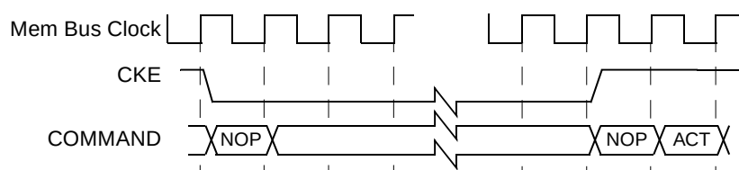
Figure 8-59. DDR SDRAM Power-Down Mode
