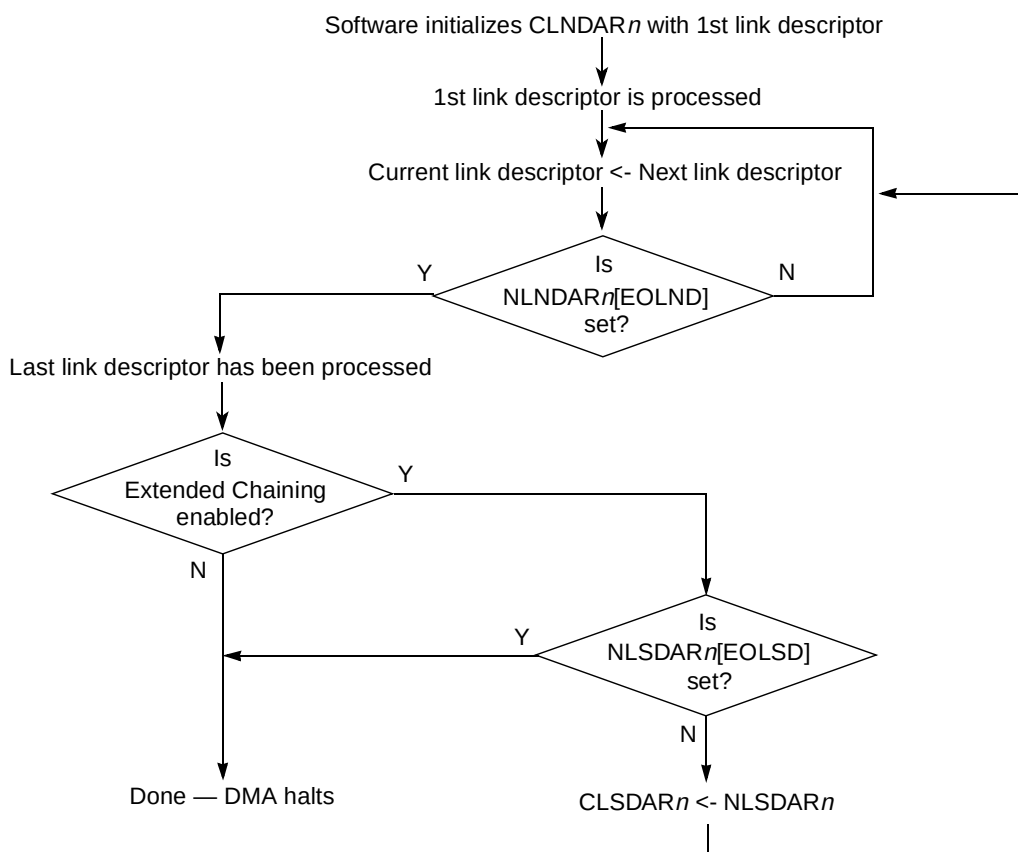
Figure 13-6. Basic Chaining Mode Flow Chart
