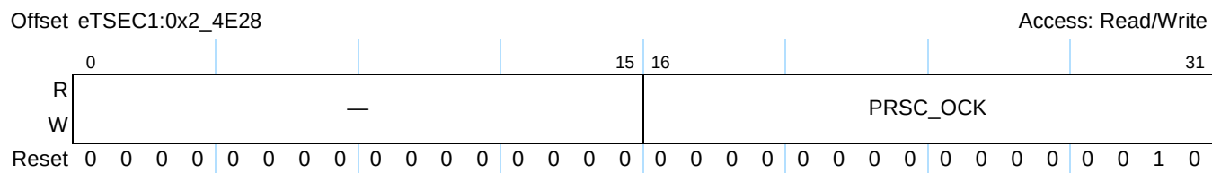
Figure 14-117. TMR_PRSC Register Definition
