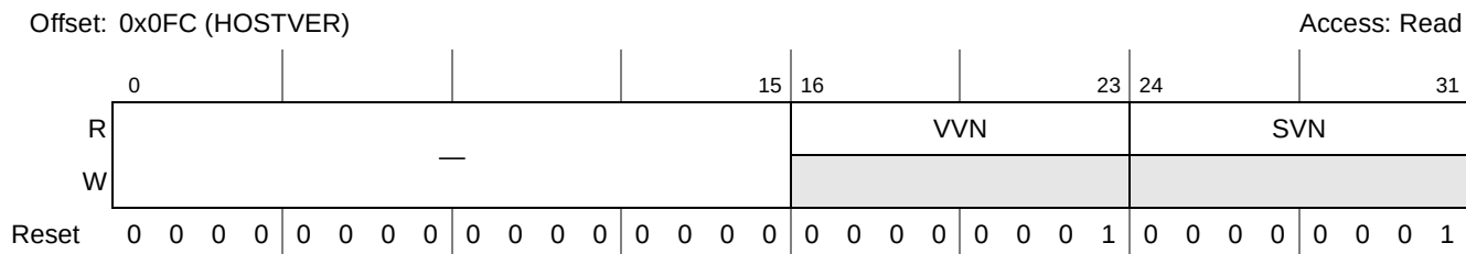
Figure 17-19. Host Controller Version Register (HOSTVER)
