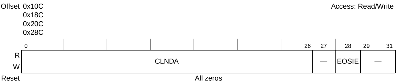
Figure 13-8. Current Link Descriptor Address Registers (CLNDAR n )
