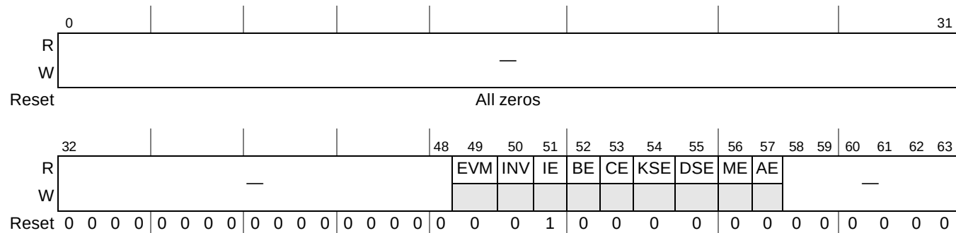
Figure 20-98. PKEU Interrupt Mask Register
