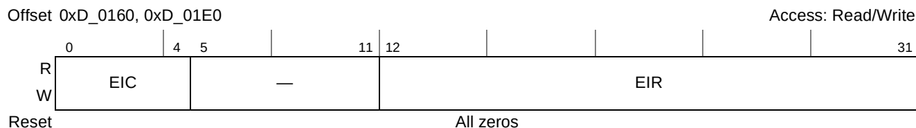
Figure 15-50. Port n Serial Link Error Injection Configuration Register (PnSLEICR)
