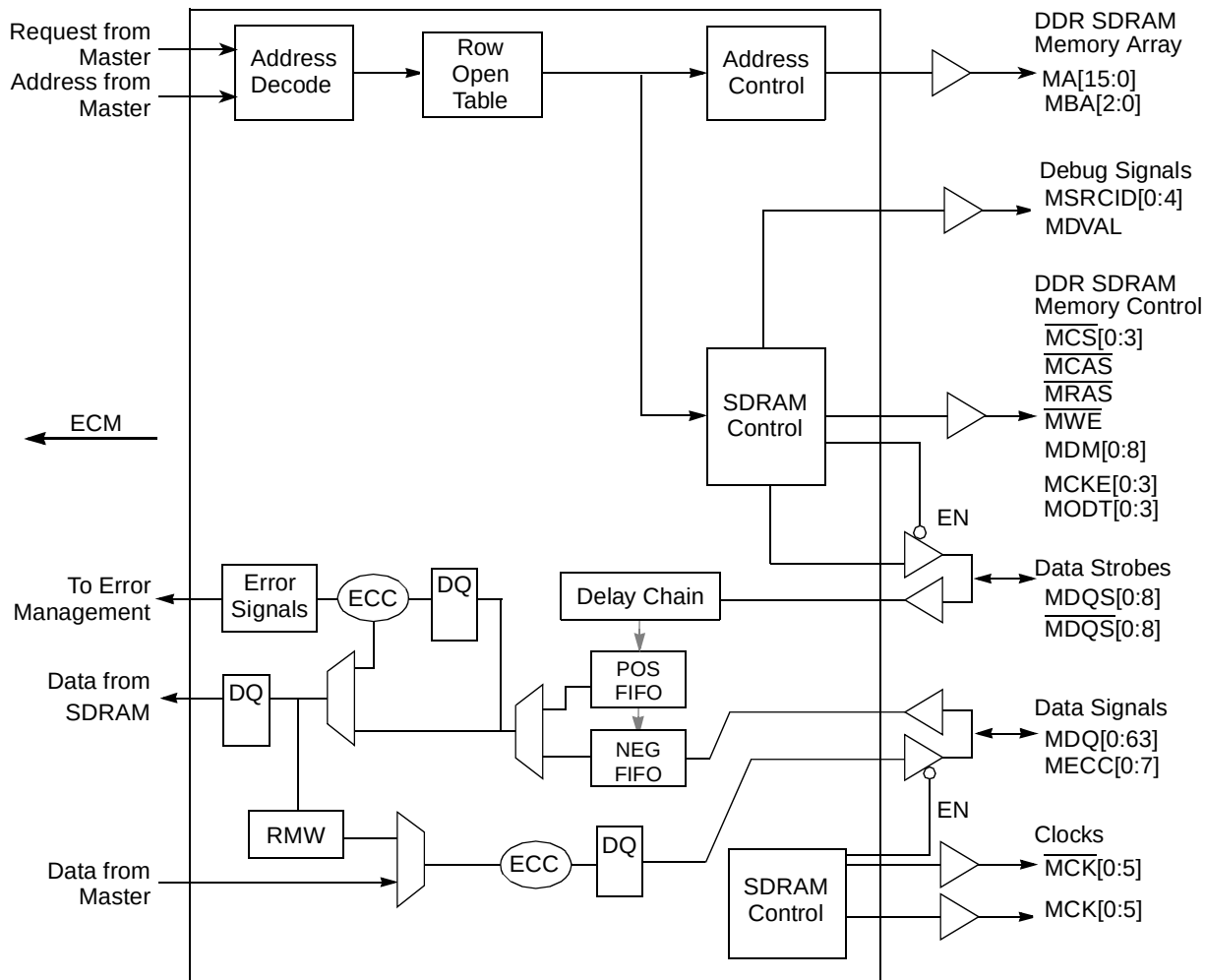
Figure 8-47. DDR Memory Controller Block Diagram
