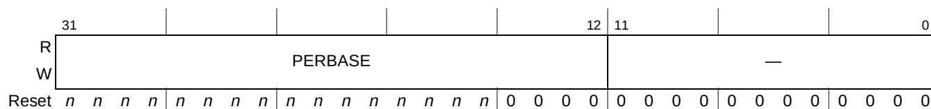
Figure 18-12. Periodic Frame List Base Address (PERIODICLISTBASE)
