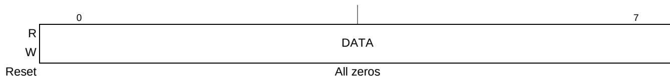
Figure 10-6. I 2 C Data Register (I2CDR)
