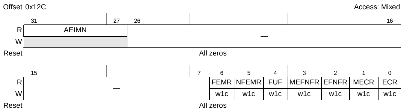
Figure 16-112. PCI Express Root Error Status Register
