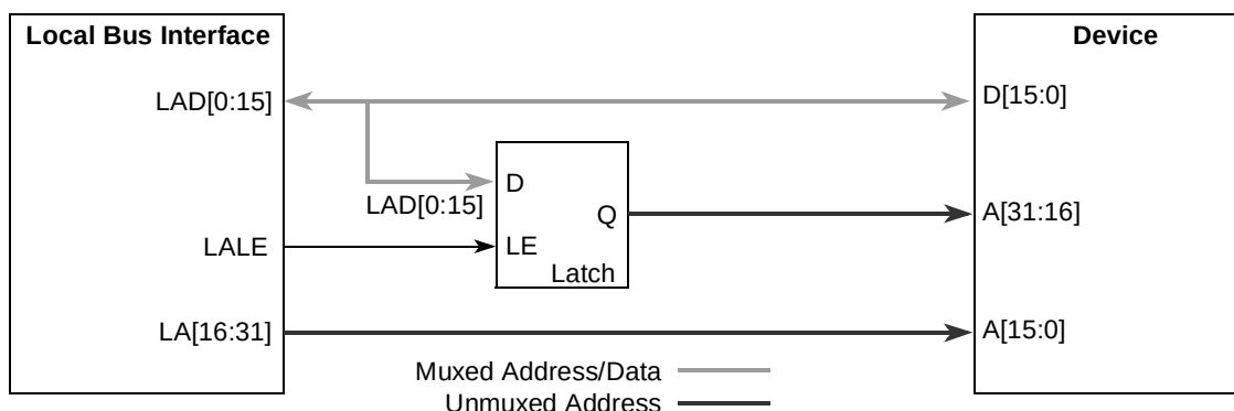
Figure 12-71. Multiplexed Address/Data Bus for 32-Bit Addressing and 16-Bit Data Bus
