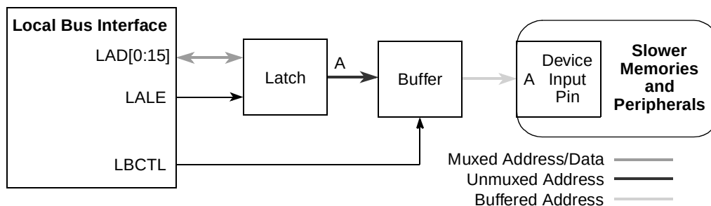
Figure 12-74. GPCM Address Timings
