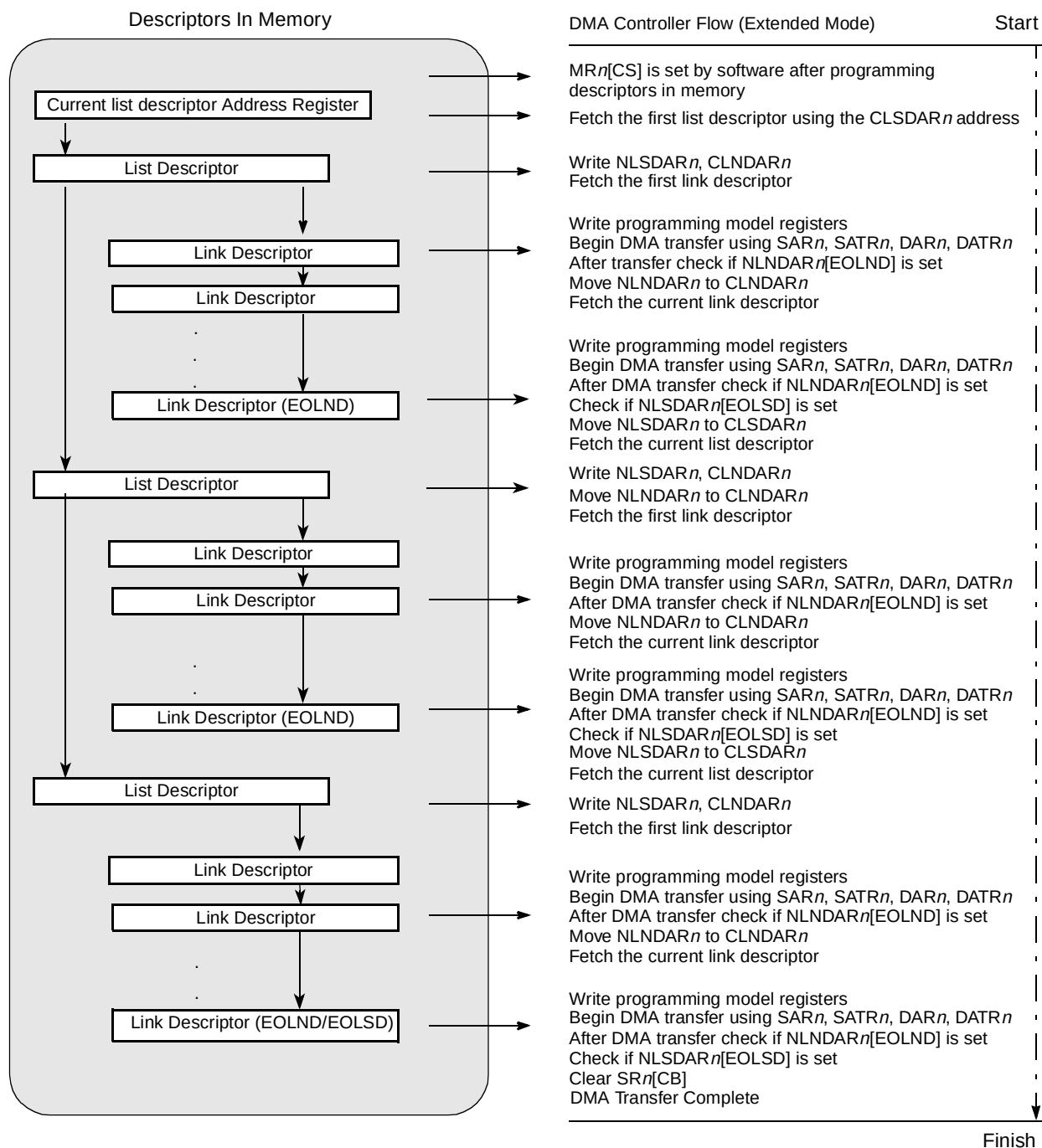
Figure 13-27. DMA Transaction Flow with DMA Descriptors
