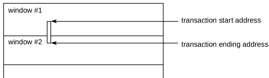
Figure 15-101. Translation Window as Hit Window
