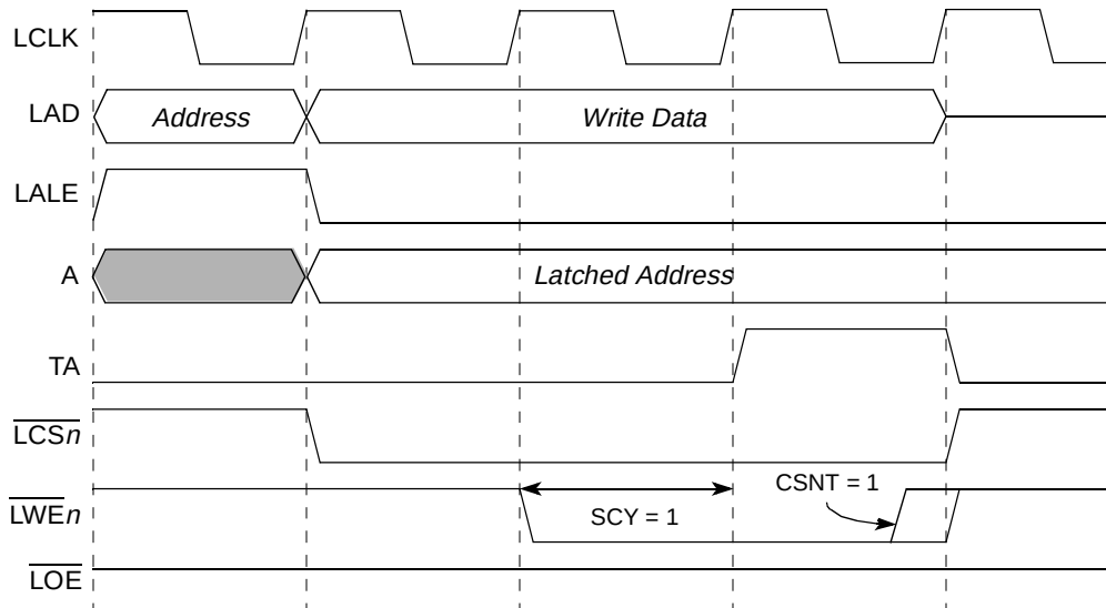
Figure 12-38. GPCM Basic Write Timing (XACS = 0, ACS = 00, CSNT = 1, SCY = 1, TRLX = 0)
