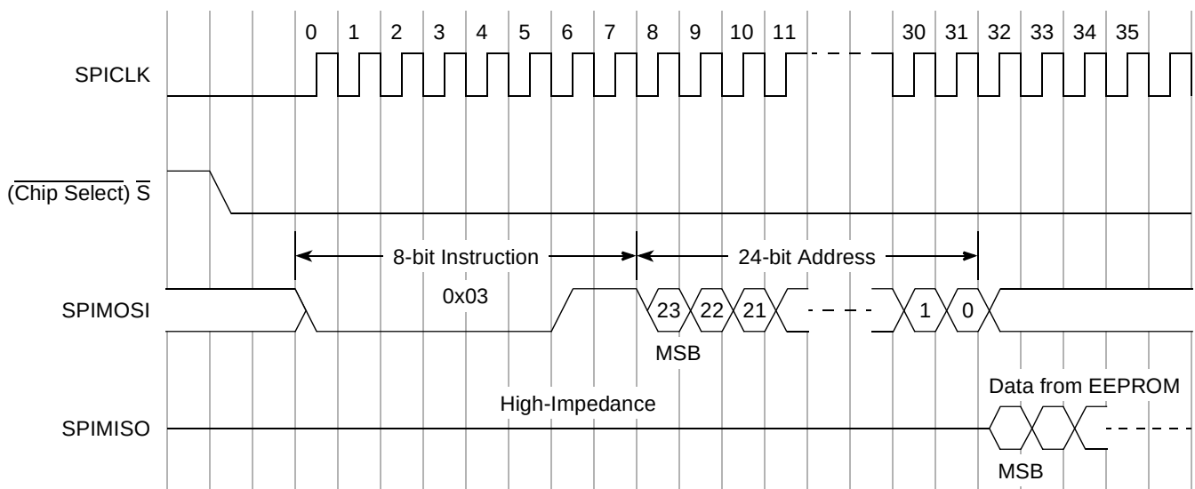
Figure 4-15. Read Instruction Timing Diagram (24-bit addressable eSPI memory)
