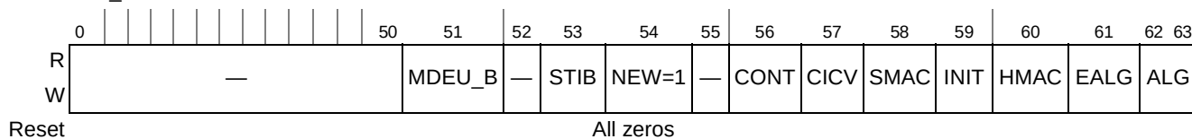
Figure 20-80. MDEU Mode Register in New Configuration
