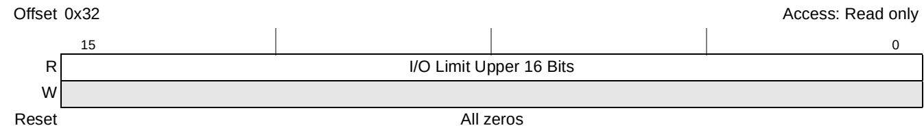
Figure 16-74. PCI Express I/O Limit Upper 16 Bits Register
