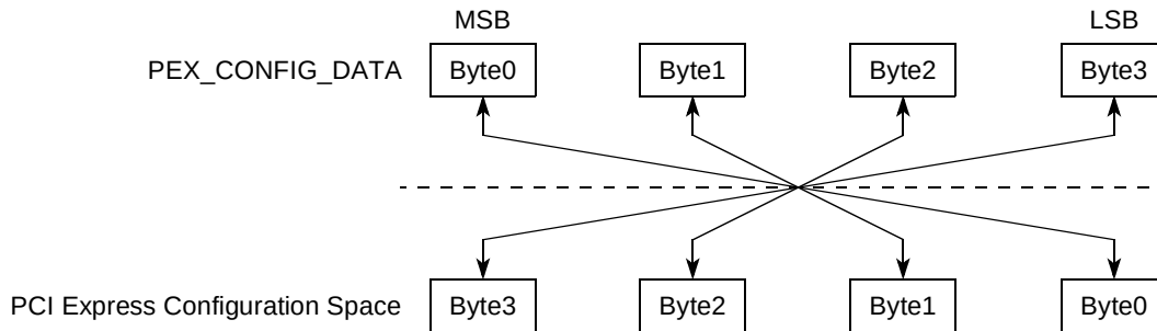
Figure 16-130. PEX_CONFIG_DATA Byte Ordering
