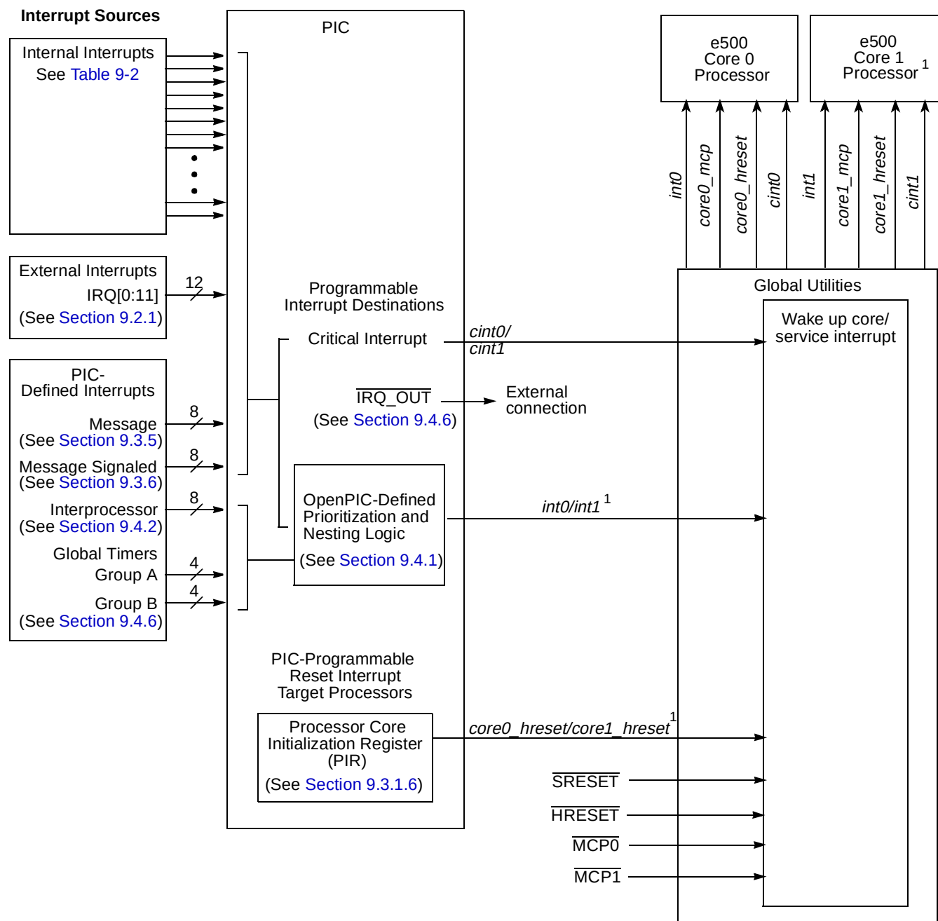
Figure 9-1. Interrupt Sources Block Diagram Features
