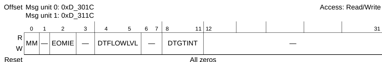
Figure 15-73. Outbound Message n Destination Attributes Registers (OM n DATR)
