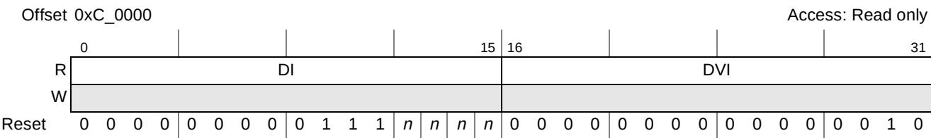
Figure 15-2. Device Identity Capability Register (DIDCAR)
