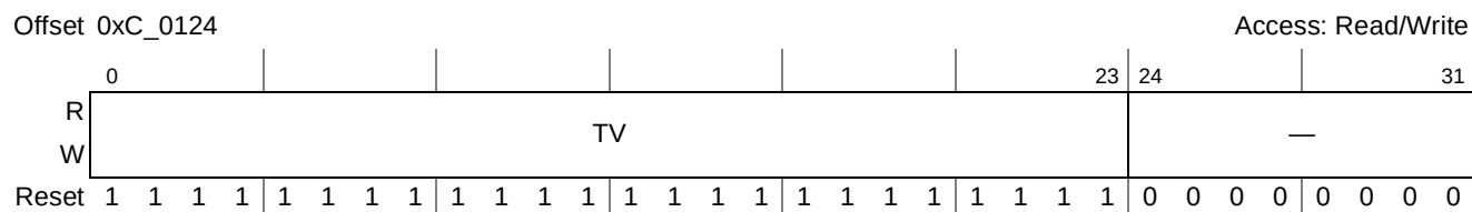
Figure 15-18. Port Response Time-Out Control Command and Status Register (PRTOCCSR)
