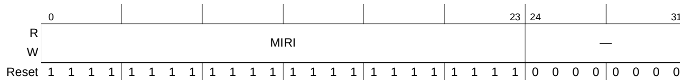
Figure 15-84. Inbound Message n Maximum Interrupt Report Interval Registers (IM n MIRIR)
