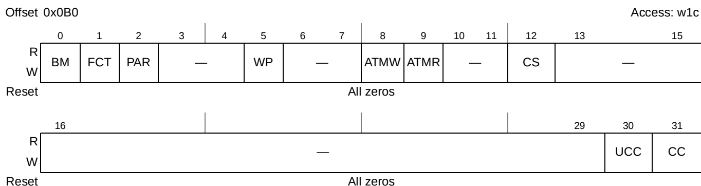
Figure 12-13. Transfer Error Status Register (LTESR)
