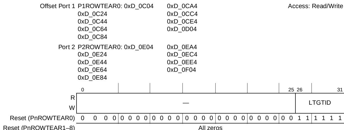
Figure 15-56. Port n RapidIO Outbound Window Translation Extended Address Registers 0–8
