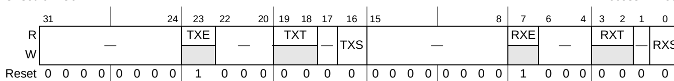
Figure 18-27. Endpoint Control 0 (ENDPTCTRL0)
