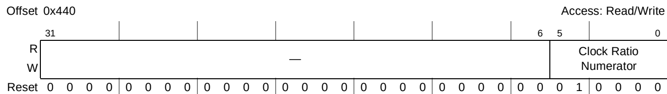
Figure 16-116. PCI Express IP Block Core Clock Ratio Register (PEX_GCLK_RATIO)
