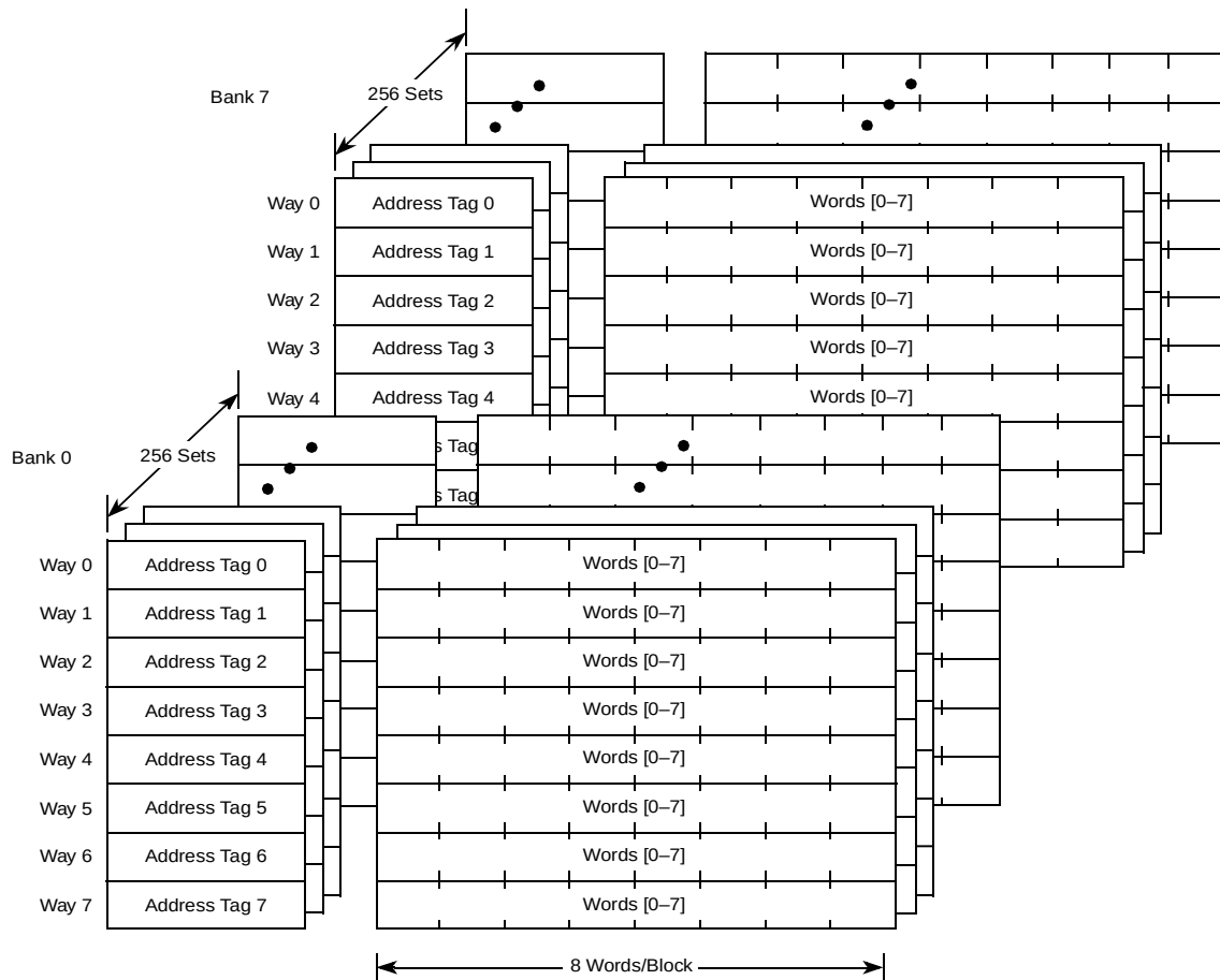
Figure 6-2. Cache Organization
