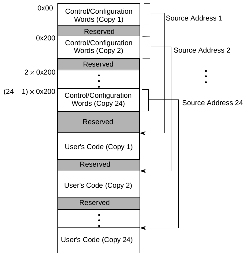
Figure 4-10. SD/MMC Card Data Structure for Maximum Redundancy
