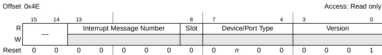
Figure 16-85. PCI Express Capabilities Register
