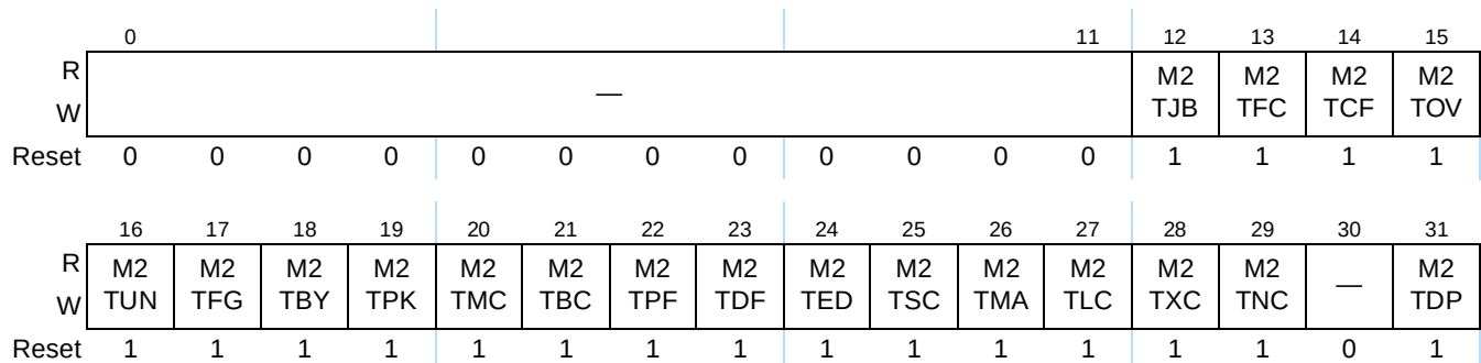
Figure 14-101. Carry Mask Register 2 (CAM2) Register Definition
