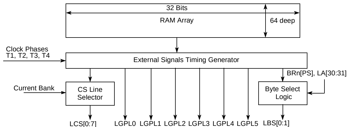
Figure 12-65. RAM Array and Signal Generation
