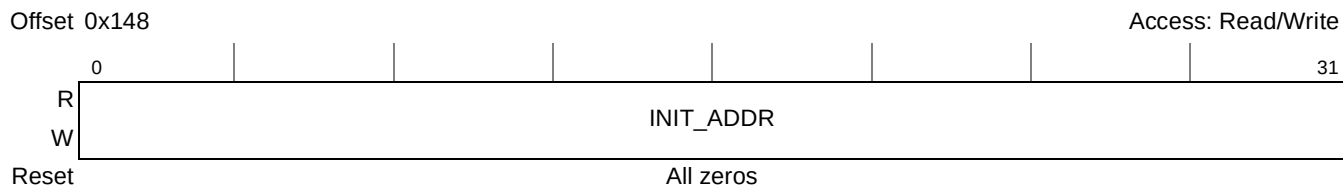
Figure 8-17. DDR Initialization Address Configuration Register (DDR_INIT_ADDR)
