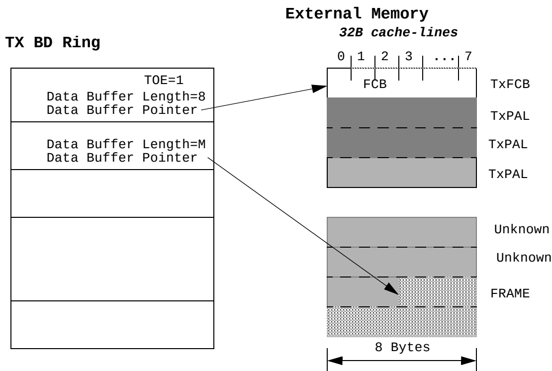
Figure 14-154. Buffer Format for Transmit Time-Stamp Insertion
