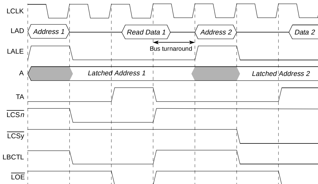
Figure 12-43. GPCM Read Followed by Read (TRLX = 0, EHTR = 0, Fastest Timing)
