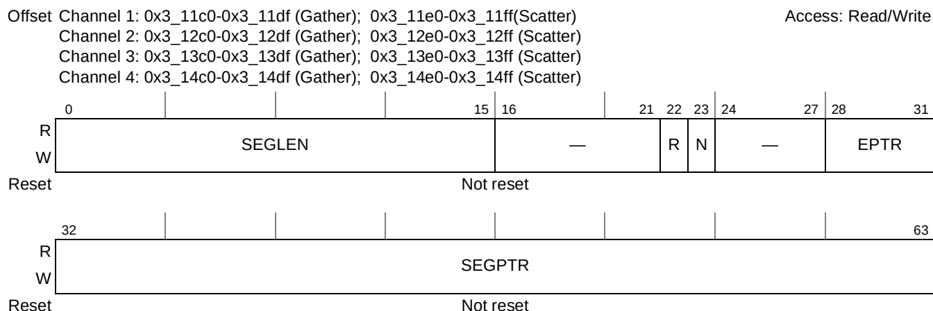
Figure 20-15. Gather/Scatter Link Table Entry Format and Memory Ranges
