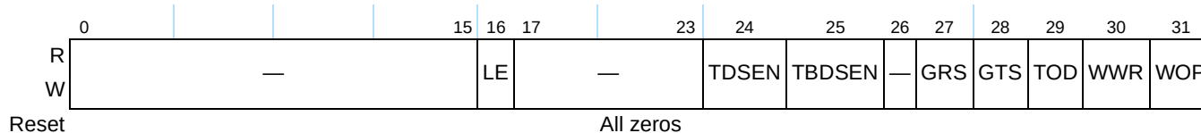
Figure 14-9. DMACTRL Register
