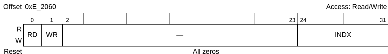
Figure 24-14. Trace Buffer Access Control Register (TBACR)
