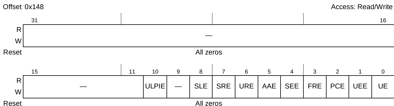
Figure 18-10. USB Interrupt Enable (USBINTR)
