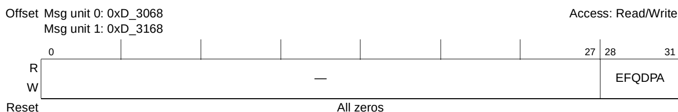
Figure 15-80. Extended Inbound Message n Frame Queue Dequeue Pointer Address Registers (EIM n FQDPA)
