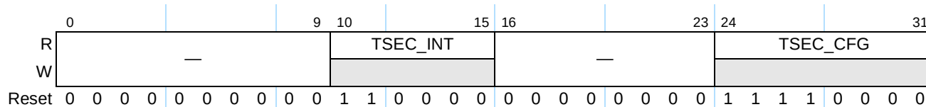
Figure 14-3. TSEC_ID2 Register
