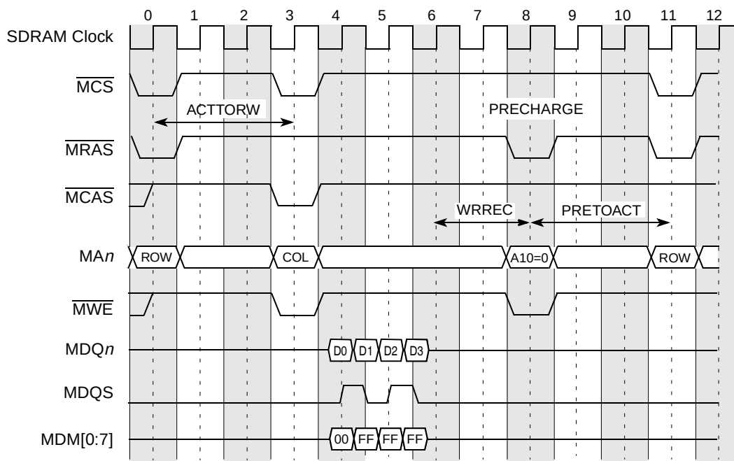
Figure 8-52. DDR SDRAM Single-Beat (Double Word) Write Timing—ACTTOR
