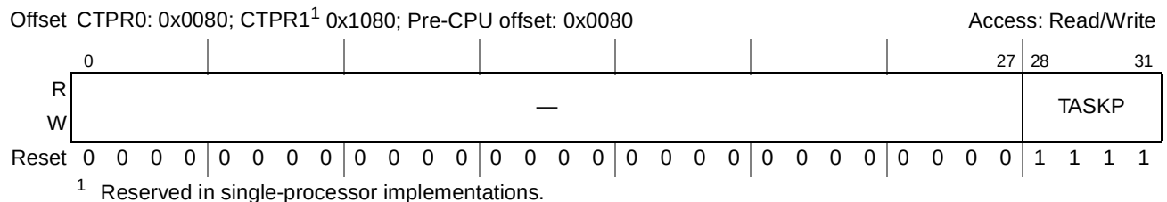
Figure 9-46. Processor Core Current Task Priority Registers (CTPR n )
