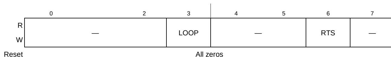
Figure 11-11. Modem Control Register (UMCR)
