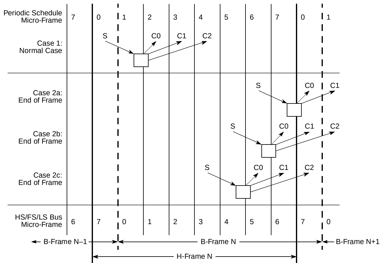
Figure 18-52. Split Transaction, Interrupt Scheduling Boundary Conditions
