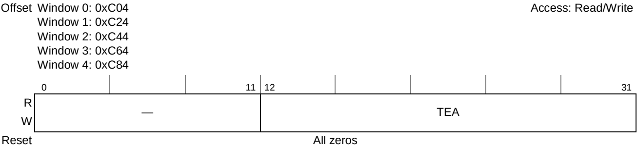
Figure 16-15. PCI Express Outbound Translation Extended Address Registers (PEXOTEAR n )
