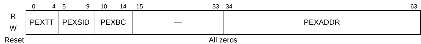
Figure 24-21. PCI Express Trace Buffer Entry
