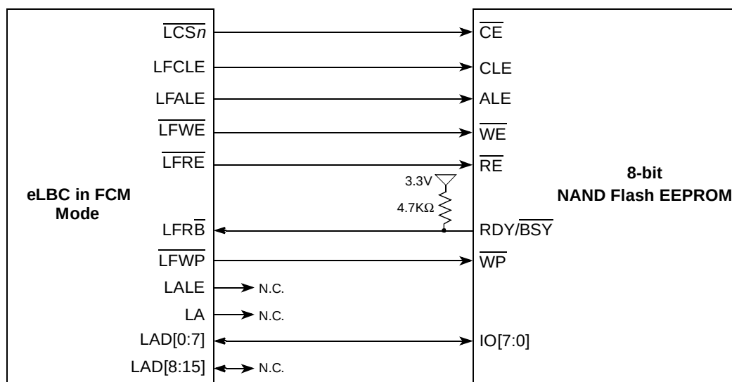
Figure 12-46. Local Bus to 8-Bit FCM Device Interface
