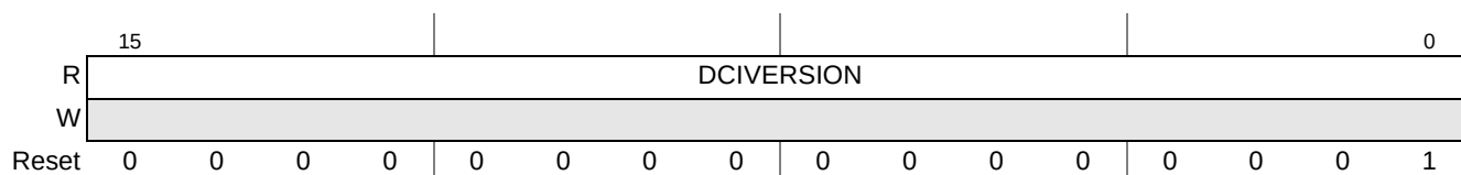
Figure 18-6. Device Interface Version (DCIVERSION)
