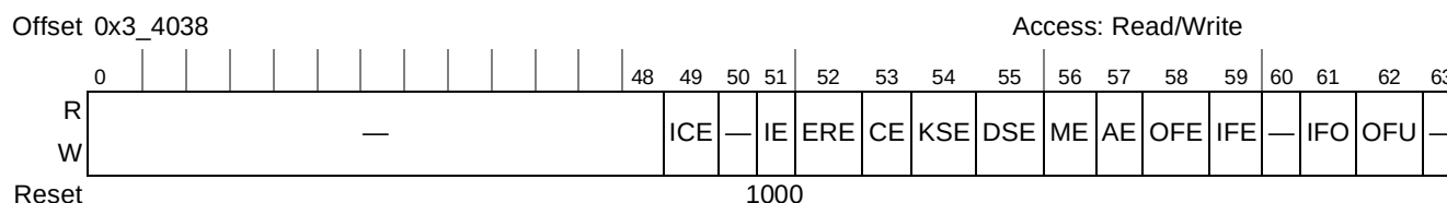
Figure 20-27. AESU Interrupt Mask Register
