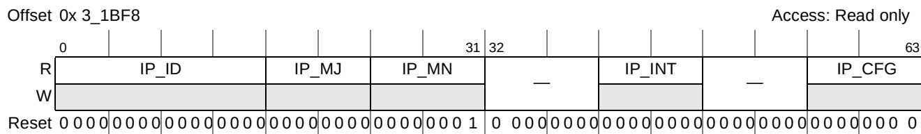
Figure 20-19. IP Block Revision Register
