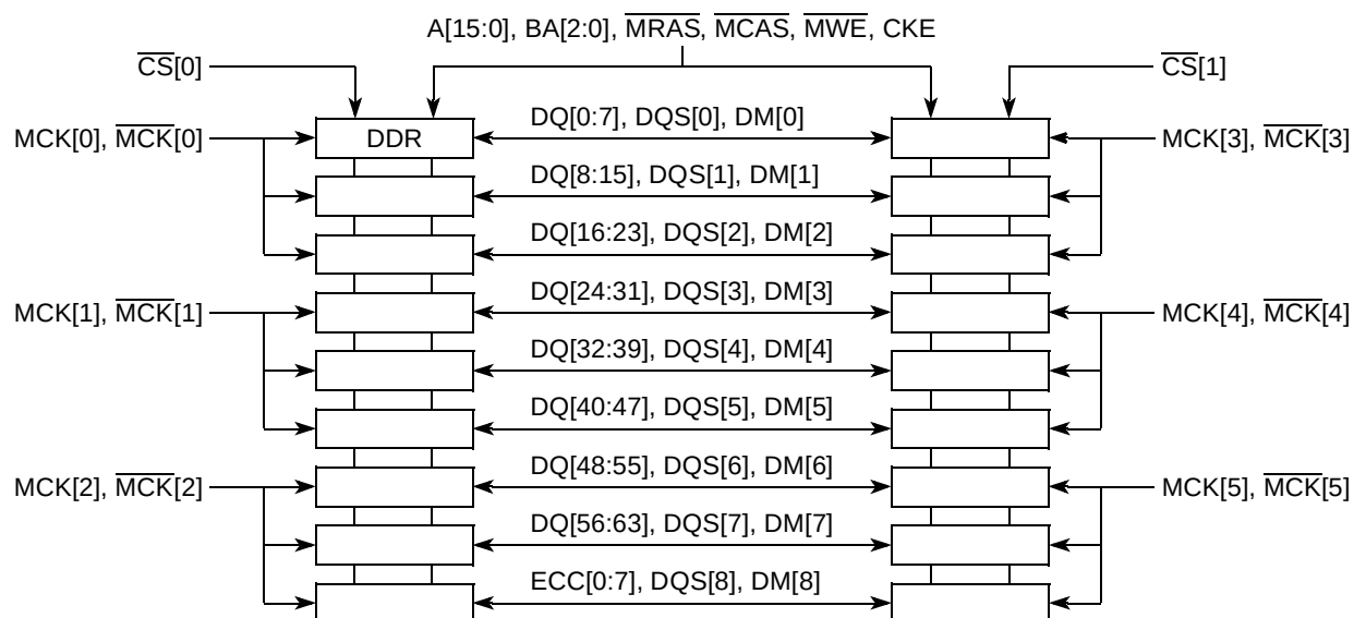
Figure 8-54. DDR SDRAM Clock Distribution Example for x8 DDR SDRAMs
