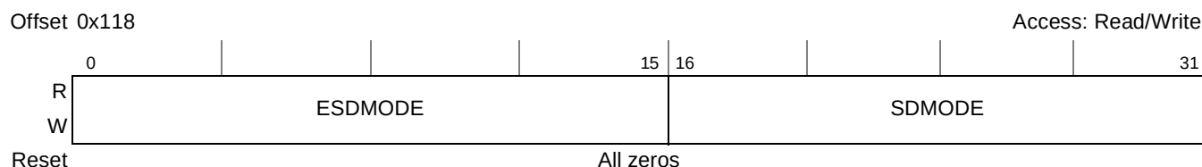
Figure 8-11. DDR SDRAM Mode Configuration Register (DDR_SDRAM_MODE)
