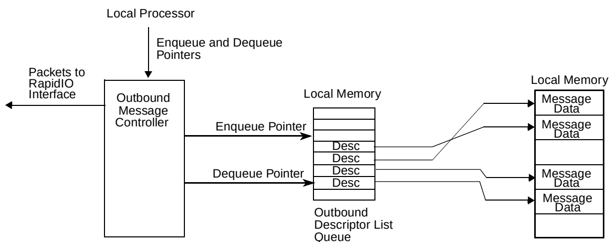
Figure 15-106. Outbound Frame Queue Structure
