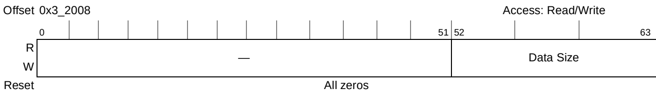
Figure 20-58. DEU Data Size Register
