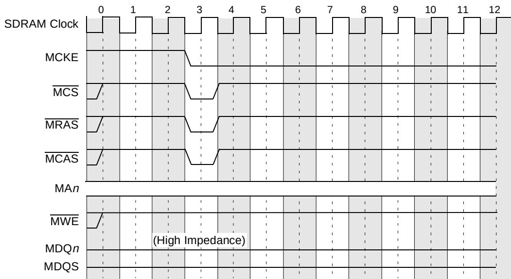
Figure 8-60. DDR SDRAM Self-Refresh Entry Timing
