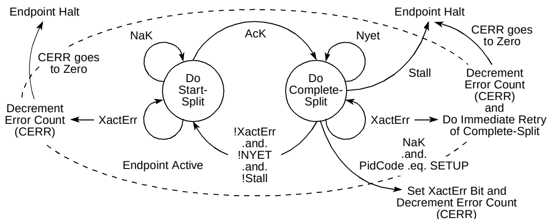
Figure 18-51. Host Controller Asynchronous Schedule Split-Transaction State Machine
