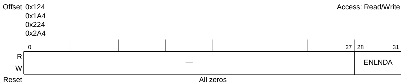
Figure 13-17. Extended Next Link Descriptor Address Registers (ENLNDAR n )
