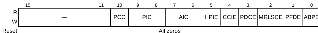
Figure 16-93. PCI Express Slot Control Register
