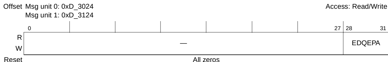
Figure 15-68. Extended Outbound Message n Descriptor Queue Enqueue Pointer Registers (EOM n DQEPAR)
