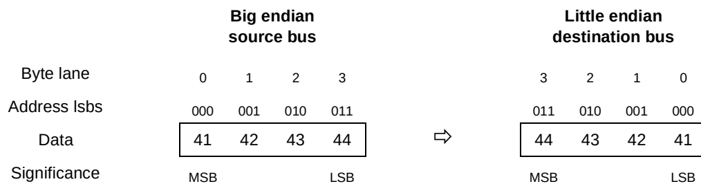
Figure 16-126. Address Invariant Byte Ordering—4 bytes Outbound
