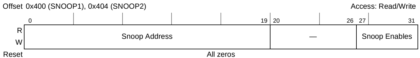
Figure 18-29. Snoop 1 and Snoop 2 (SNOOP n )
