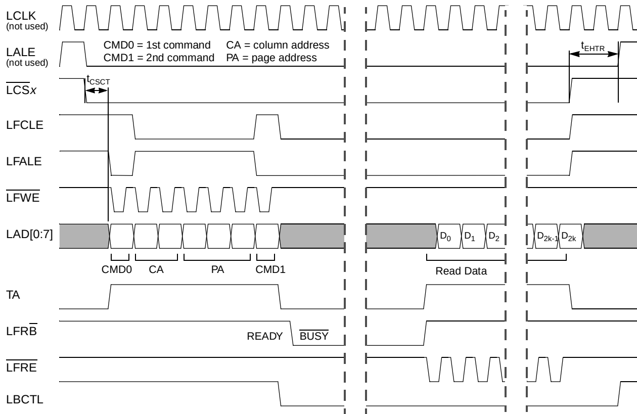
Figure 12-47. FCM Basic Page Read Timing (PGS = 1, CSCT = 0, CST = 0, CHT = 1, RST = 1, SCY = 0, TRLX = 0, EHTR = 1)
