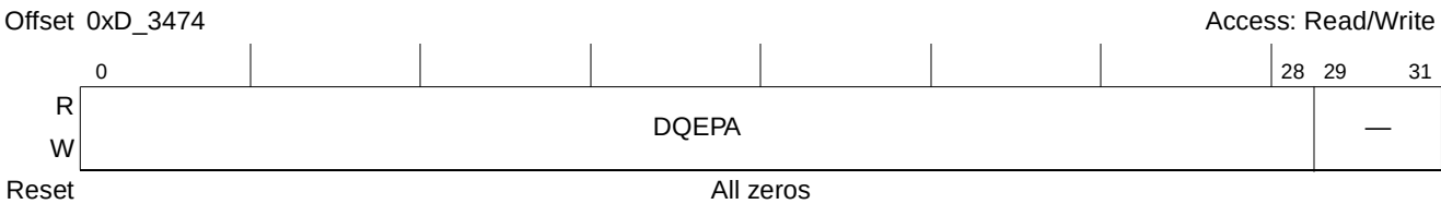
Figure 15-95. Inbound Doorbell Queue Enqueue Pointer Address Register (IDQEPAR)
