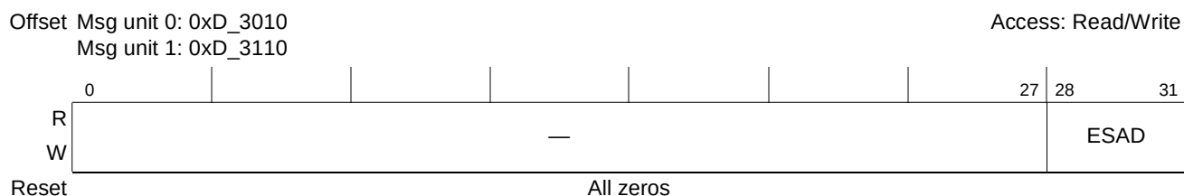
Figure 15-70. Extended Outbound Message n Source Address Registers (EOM n SAR)
