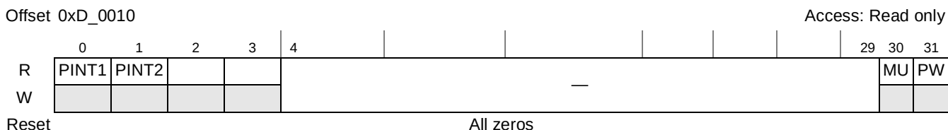
Figure 15-41. Error/Port-Write Interrupt Status Register (EPWISR)
