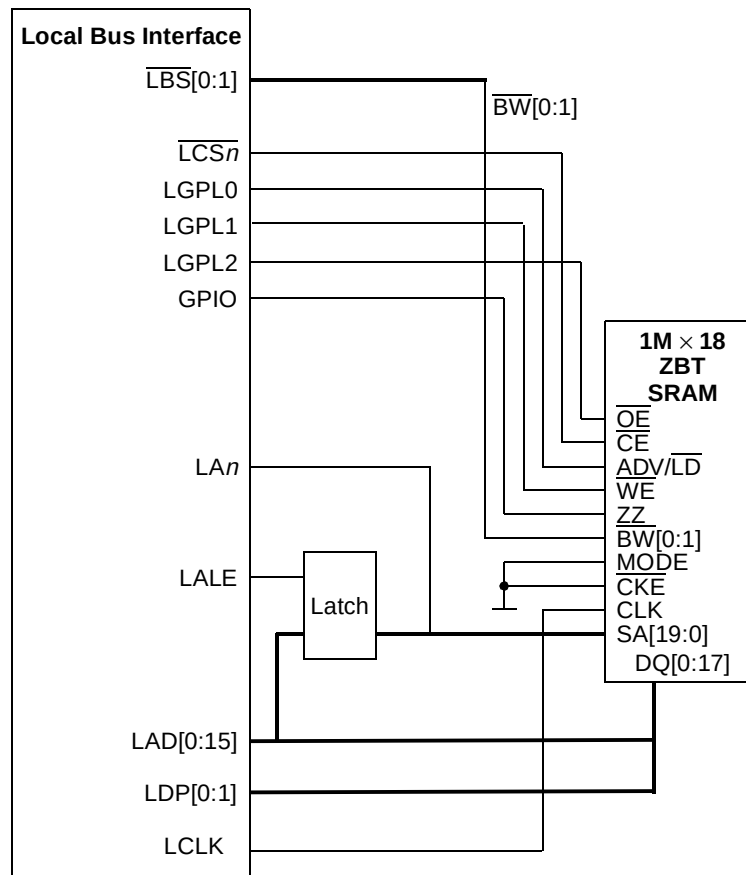
Figure 12-82. Interface to ZBT SRAM
