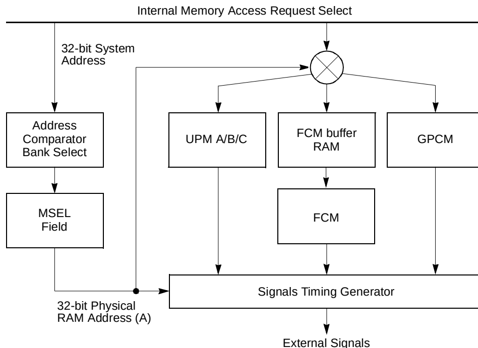
Figure 12-29. Basic Operation of Memory Controllers in the eLBC
