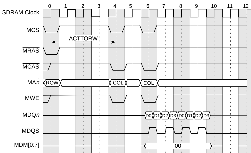
Figure 8-56. Registered DDR SDRAM DIMM Burst Write Timing
