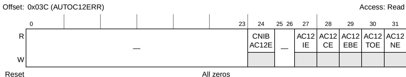
Figure 17-15. Auto CMD12 Error Status Register (AUTOC12ERR)
