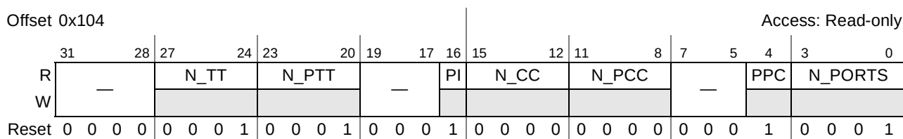
Figure 18-4. Host Controller Structural Parameters (HCSPARAMS)
