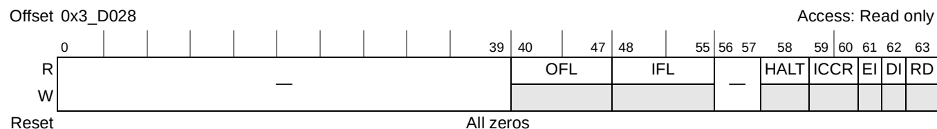
Figure 20-111. STEU Status Register
