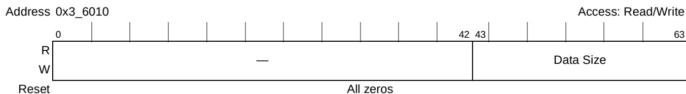
Figure 20-83. MDEU Data Size Register
