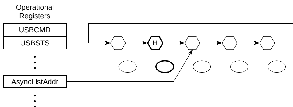
Figure 18-43. General Format of Asynchronous Schedule List
