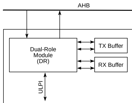
Figure 18-1. USB Interface Block Diagram
