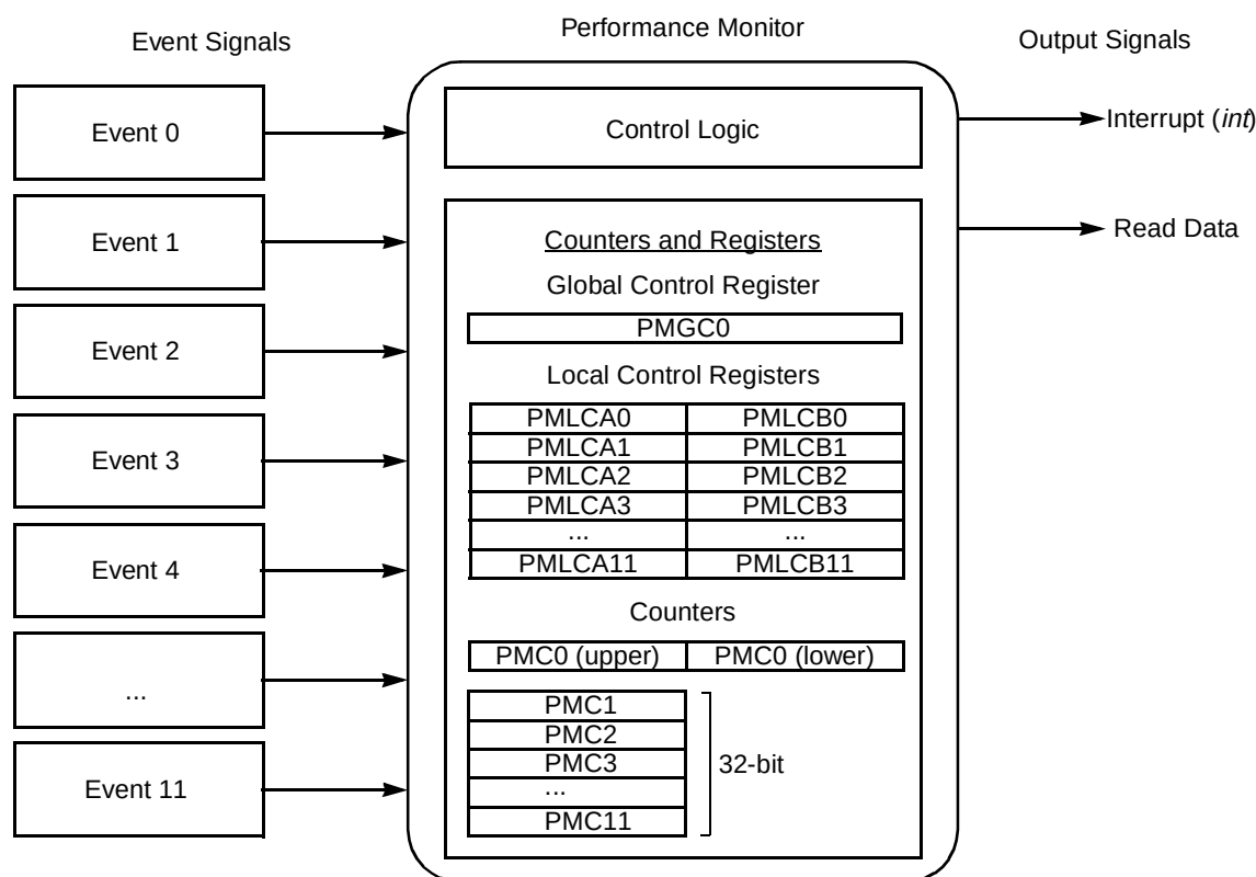
Figure 23-1. Performance Monitor Block Diagram
