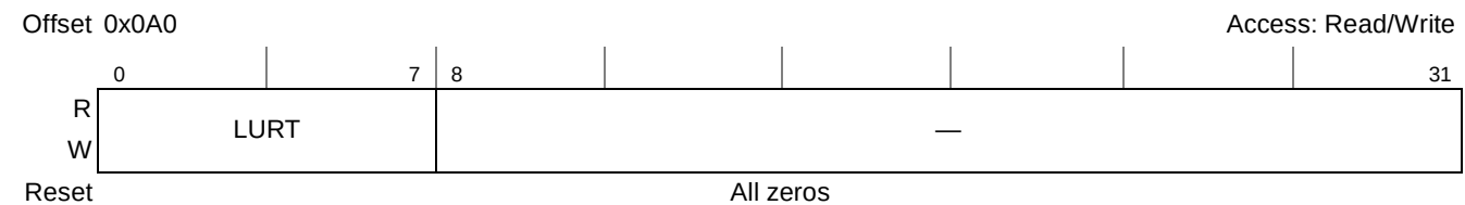
Figure 12-12. UPM Refresh Timer (LURT)
