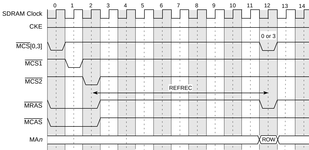
Figure 8-58. DDR SDRAM Bank Staggered Auto Refresh Timing
