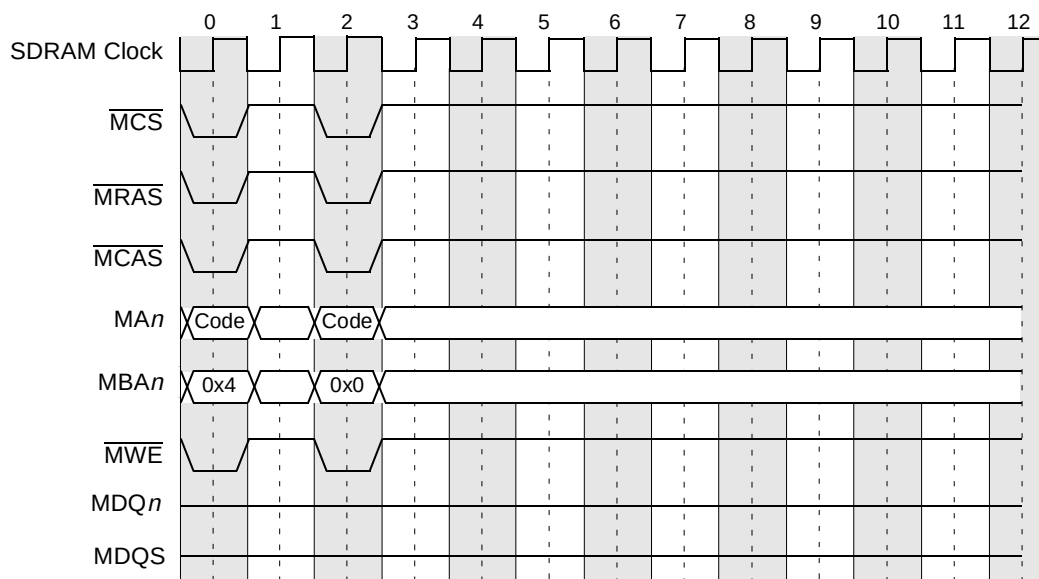
Figure 8-55. DDR SDRAM Mode-Set Command Timing
