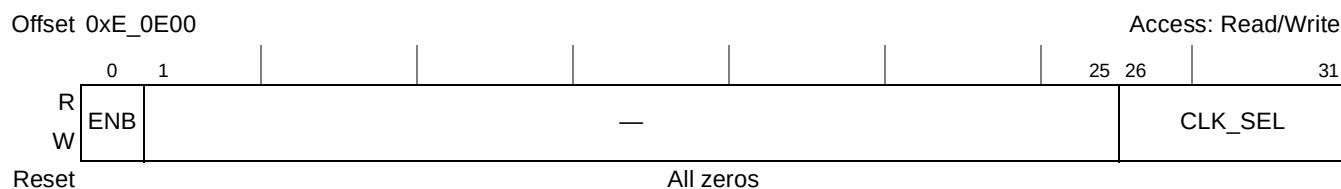
Figure 22-20. Clock Out Control Register (CLKOCR)
