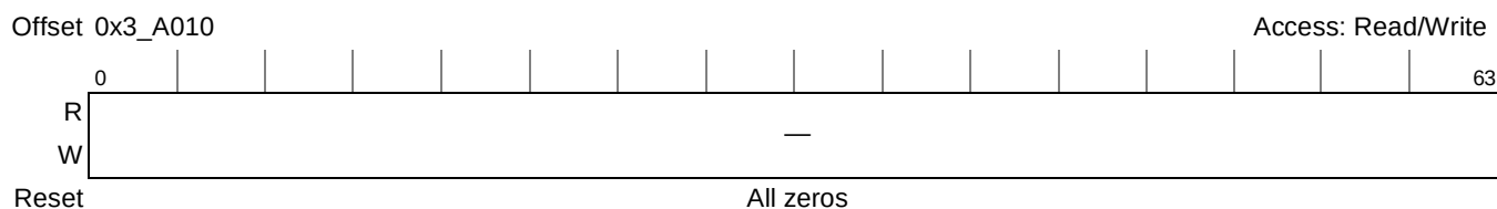
Figure 20-101. RNGU Data Size Register
