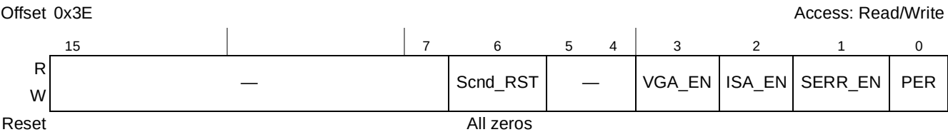
Figure 16-78. PCI Express Bridge Control Register
