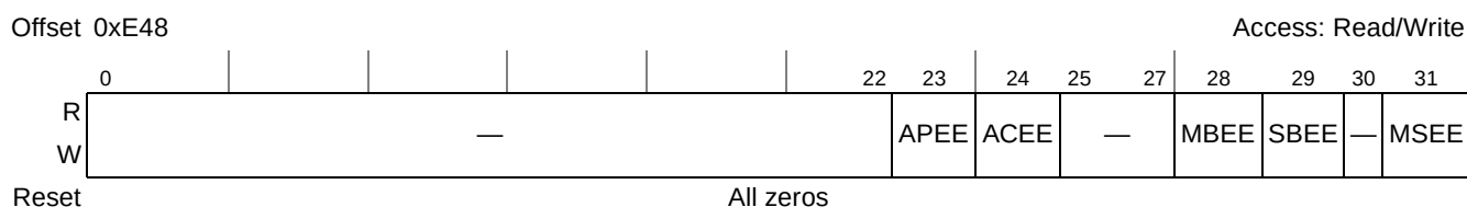
Figure 8-42. Memory Error Interrupt Enable Register (ERR INT EN)
