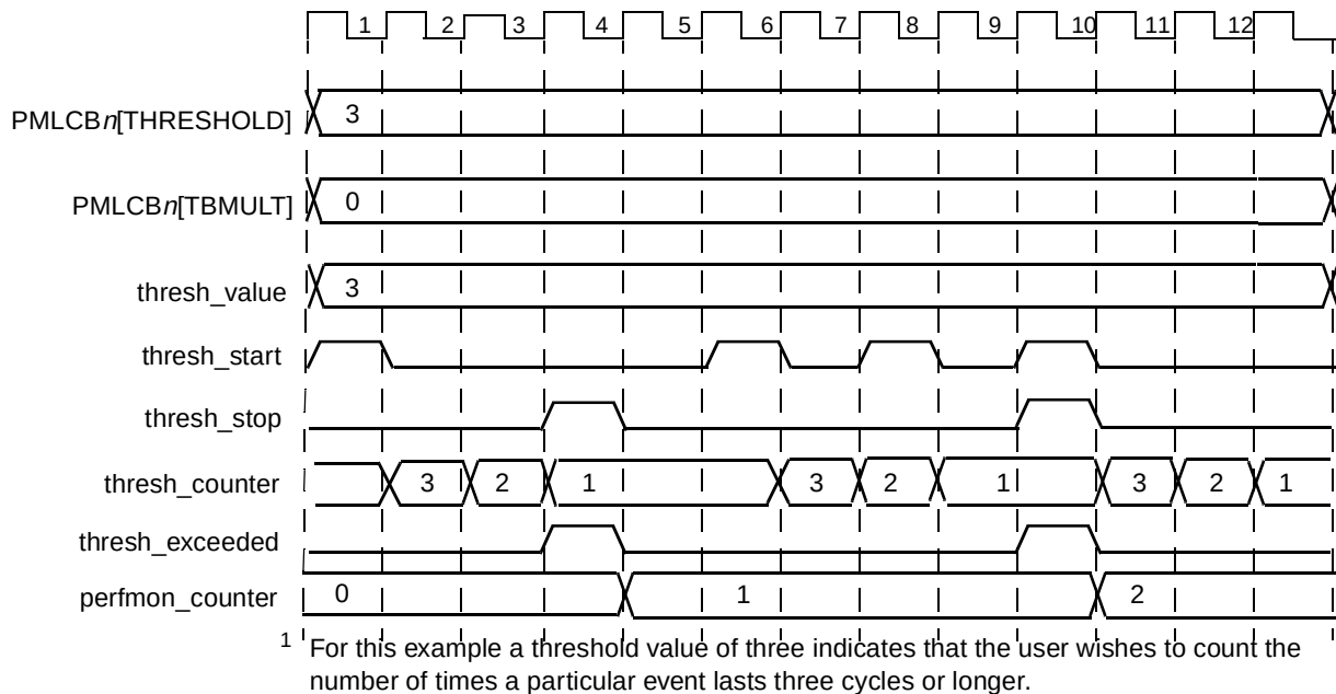
Figure 23-9. Duration Threshold Event Sequence Timing Diagram
