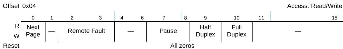
Figure 14-124. AN Advertisement Register Definition
