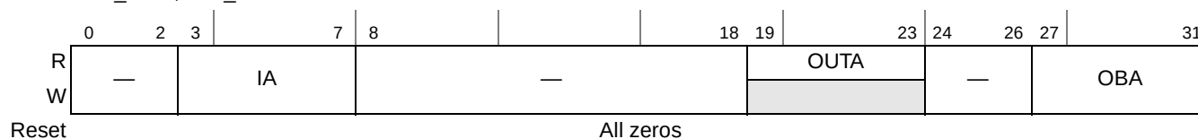
Figure 15-22. Port n Local ackID Status Command and Status Register (PnLASCSR)
