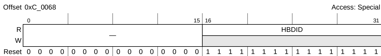
Figure 15-14. Host Base Device ID Lock Command and Status Register (HBDIDLCSR)
