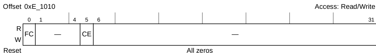
Figure 23-3. Performance Monitor Local Control Register A0 (PMLCA0)
