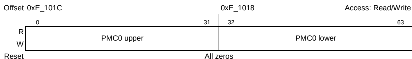
Figure 23-7. Performance Monitor Counter Register 0 (PMC0)
