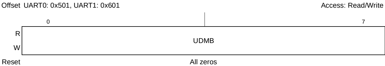
Figure 11-4. Divisor Most Significant Byte Registers (UDMB0, UDMB1)
