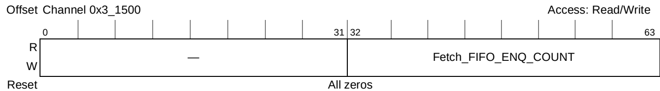
Figure 20-7. Fetch FIFO Enqueue Counter
