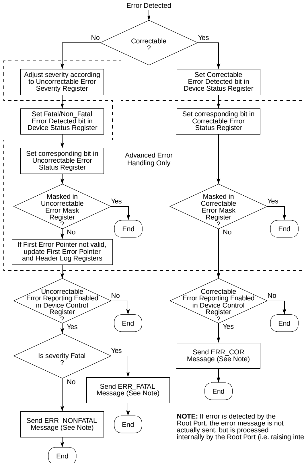
Figure 16-132. PCI Express Device Error Signaling Flowchart
