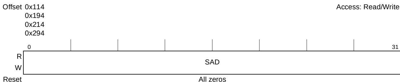
Figure 13-10. Source Address Registers (SAR n )
