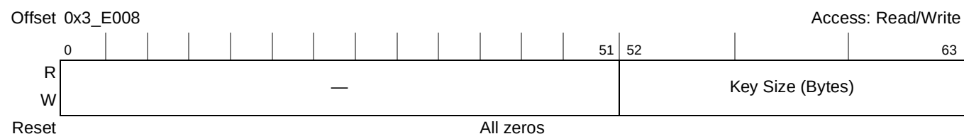
Figure 20-65. KEU Key Size Register
