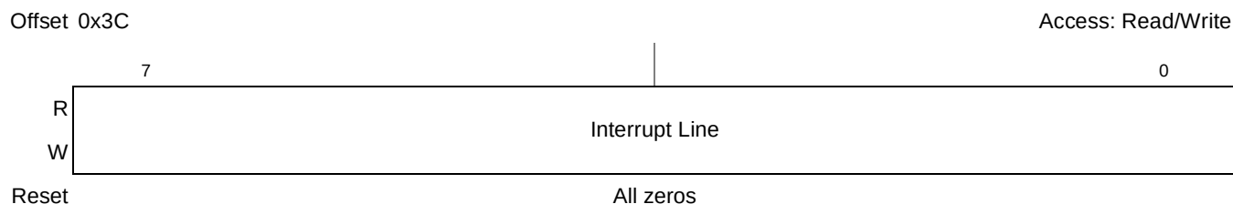
Figure 16-76. PCI Express Interrupt Line Register
