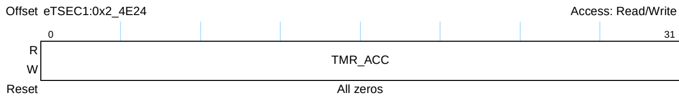
Figure 14-116. TMR_ACC Register Definition
