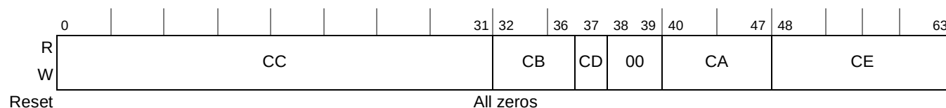
Figure 20-73. KEU IV_1 Register
