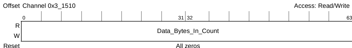
Figure 20-9. Data Bytes In Counter
