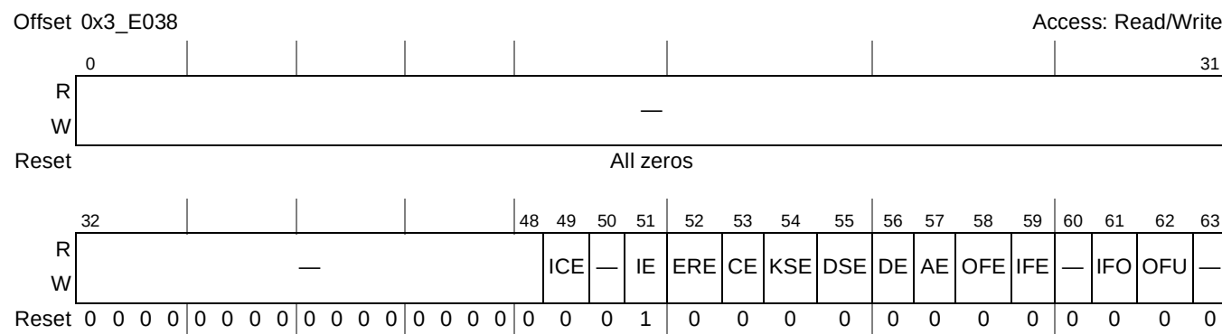
Figure 20-70. KEU Interrupt Mask Register
