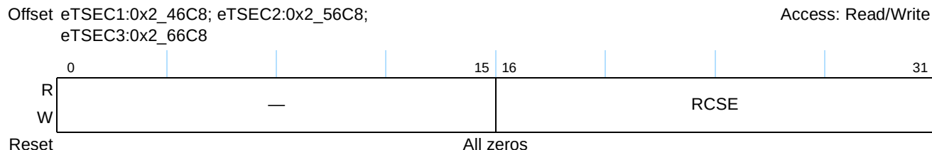
Figure 14-73. Receive Carrier Sense Error Counter Register Definition
