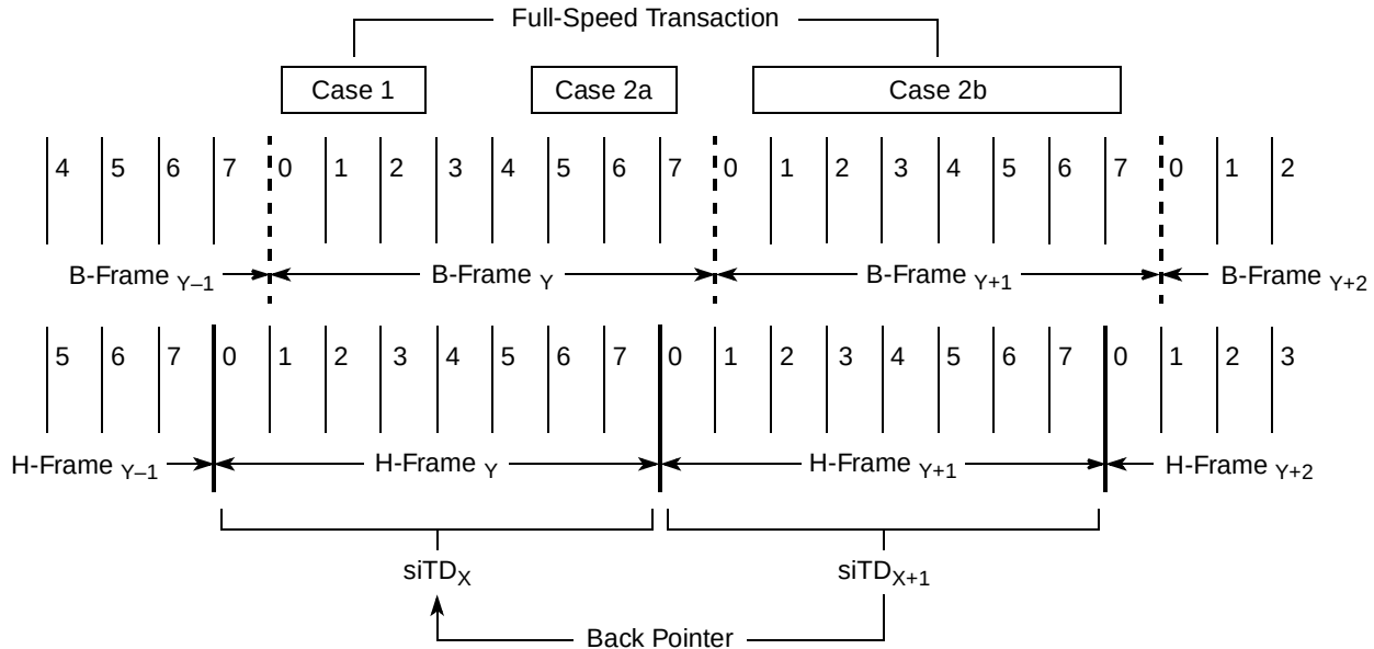
Figure 18-57. siTD Scheduling Boundary Examples
