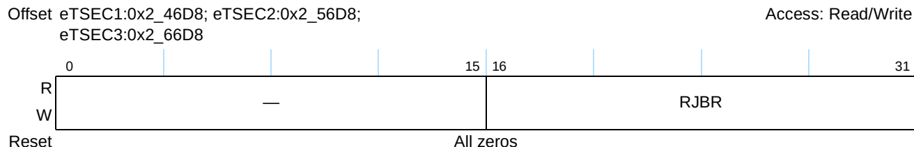
Figure 14-77. Receive Jabber Counter Register Definition
