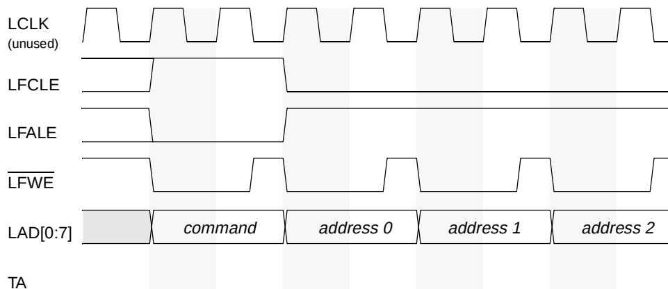
Figure 12-55. Example of FCM Command and Address Timing with Minimum Delay Parameters (for TRLX = 0, CHT = 0, CST = 0, SCY = 0)
