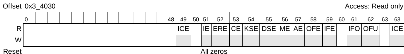
Figure 20-26. AESU Interrupt Status Register
