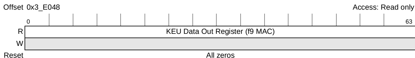
Figure 20-71. KEU Data Out Register (f9 MAC)
