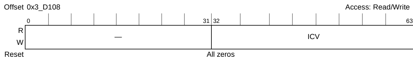
Figure 20-117. STEU ICD In Register
