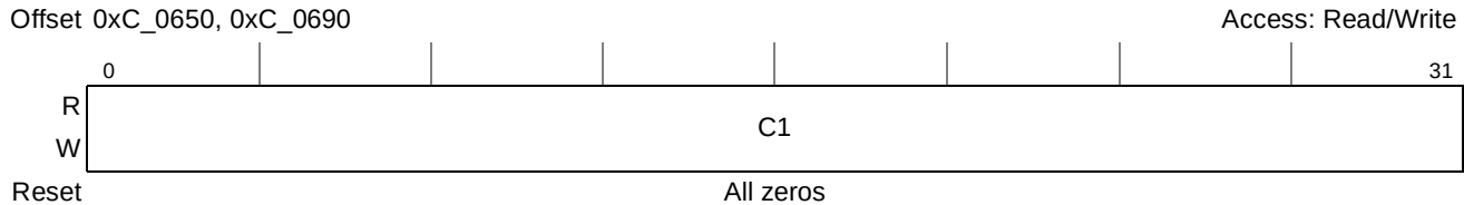
Figure 15-35. Port n Packet Error Capture Command and Status Register 1 ( PnPECCSR1 )
