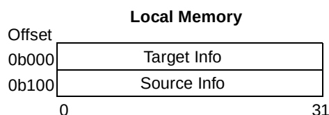
Figure 15-110. Doorbell Entry Format
