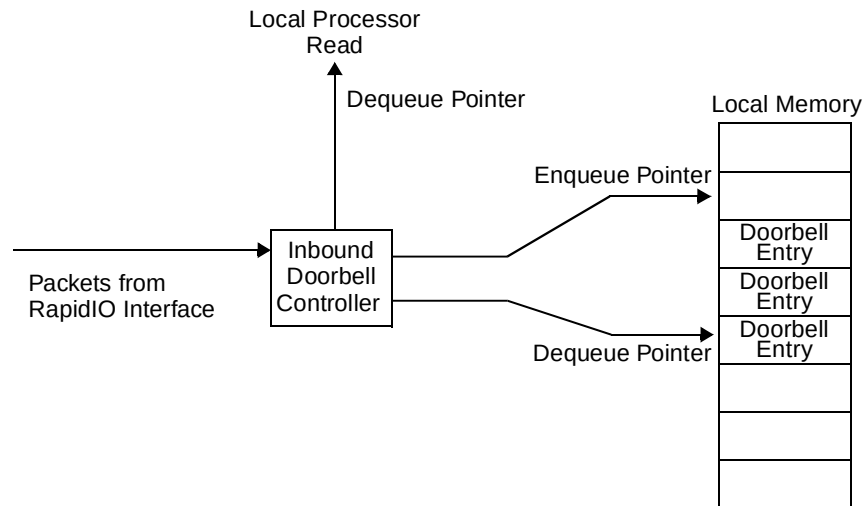
Figure 15-109. Inbound Doorbell Queue and Pointer Structure
