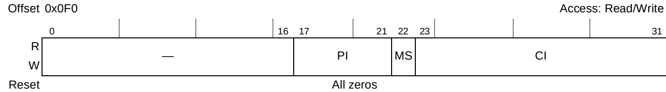
Figure 12-25. Flash Page Address Register, Small Page Device (OR x [PGS] = 0)
