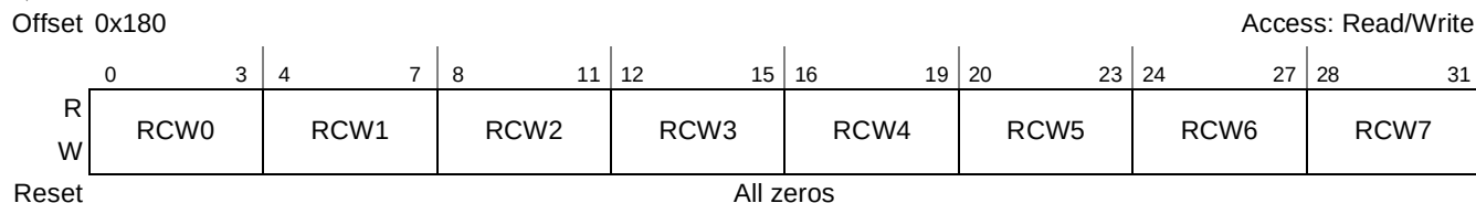
Figure 8-26. DDR Register Control Word 1 (DDR_SDRAM_RCW_1)
