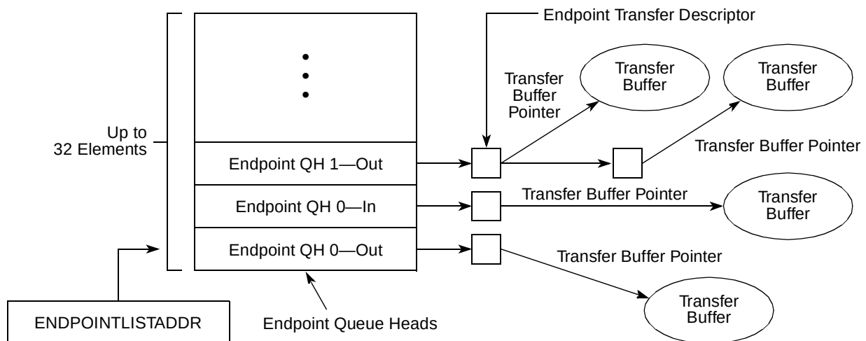
Figure 18-59. Endpoint Queue Head Organization
