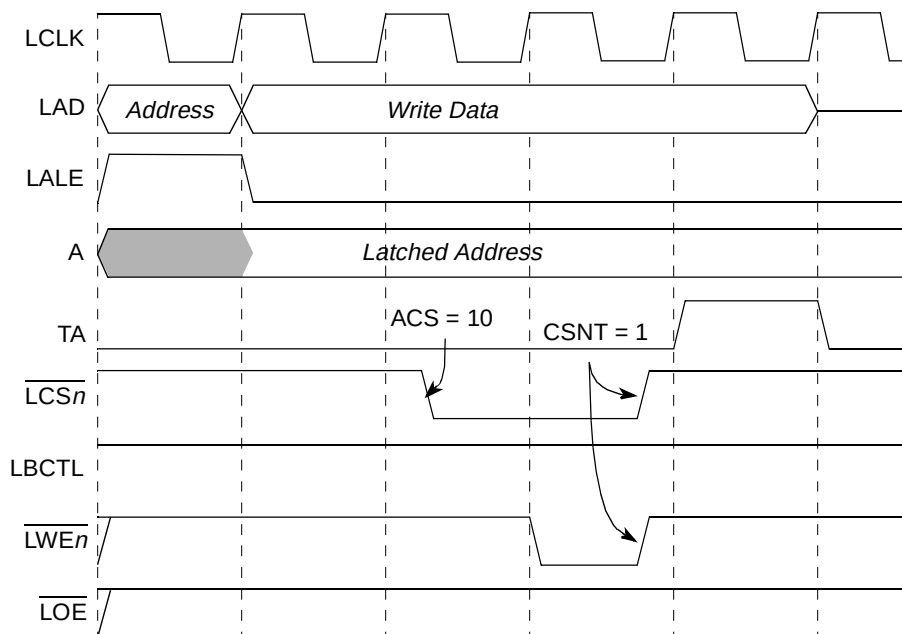
Figure 12-41. GPCM Relaxed Timing Write (XACS = 0, ACS = 10, SCY = 0, CSNT = 1, TRLX = 1)
