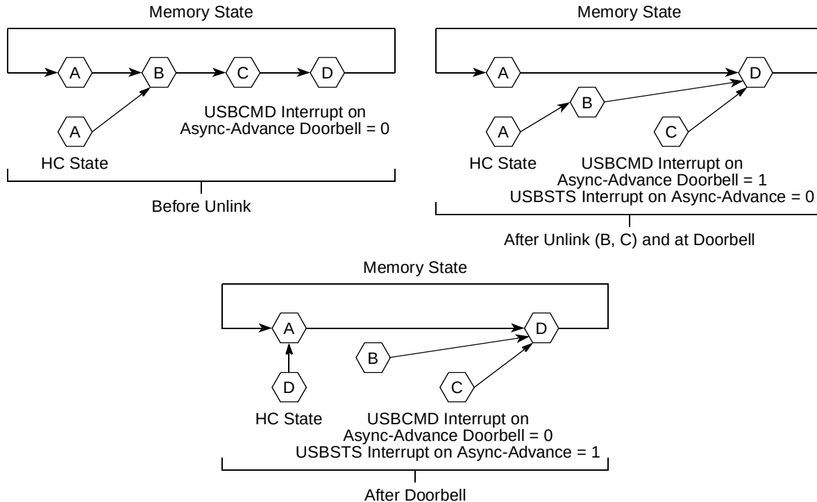
Figure 18-48. Generic Queue Head Unlink Scenario
