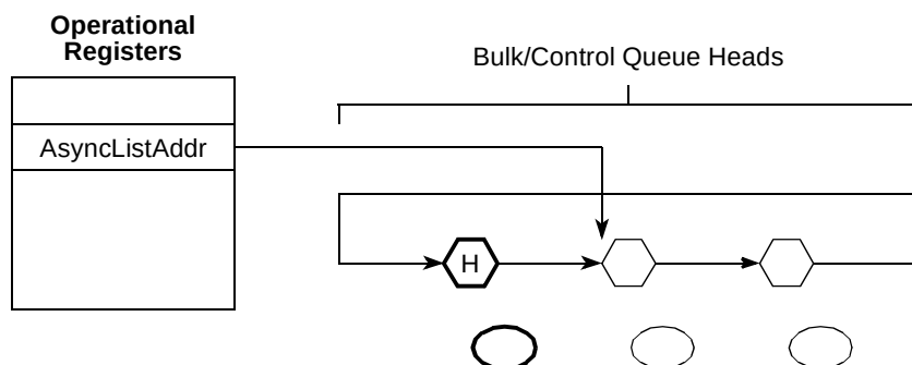
Figure 18-36. Asynchronous Schedule Organization
