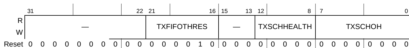
Figure 18-17. Transmit FIFO Tuning Controls (TXFILLTUNING)
