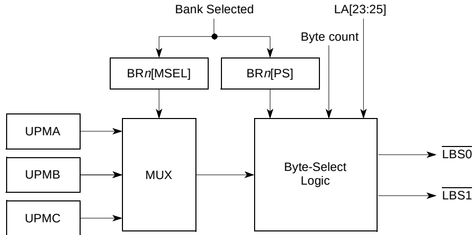
Figure 12-68. \overline{\text{LBS}} Signal Selection
