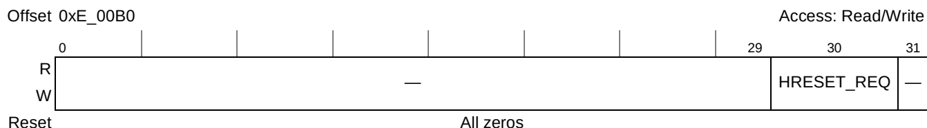
Figure 22-17. Reset Control Register (RSTCR)
