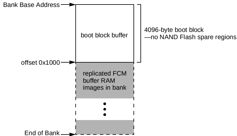
Figure 12-60. FCM Buffer RAM Memory Map During Boot Loading
