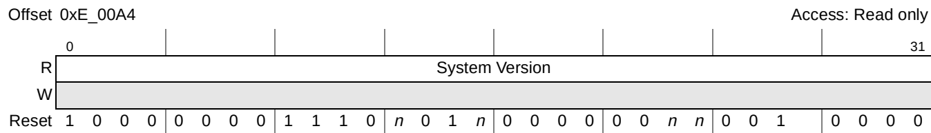
Figure 22-16. System Version Register (SVR)
