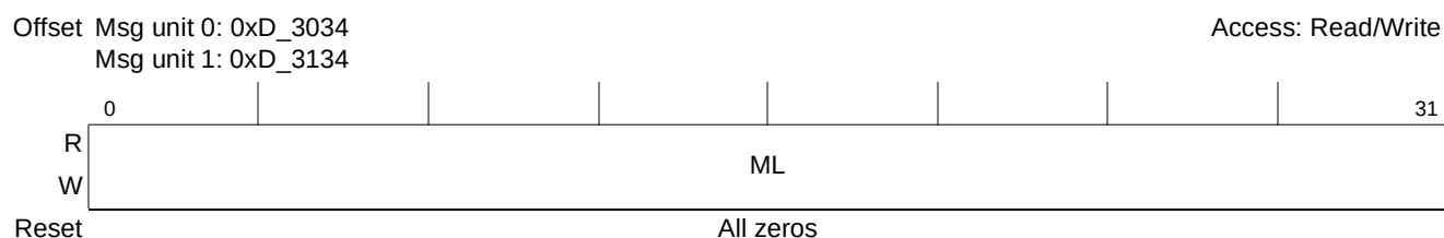
Figure 15-77. Outbound Message n Multicast List Registers (OM n MLR)
