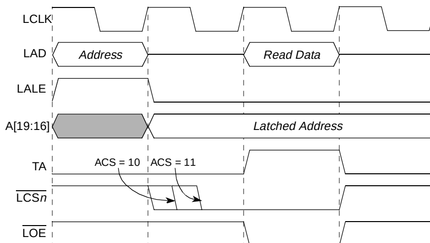
Figure 12-35. GPCM Basic Read Timing (XACS = 0, ACS = 1x, TRLX = 0)
