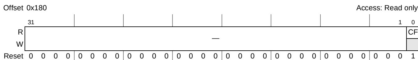
Figure 18-19. Configure Flag Register (CONFIGFLAG)
