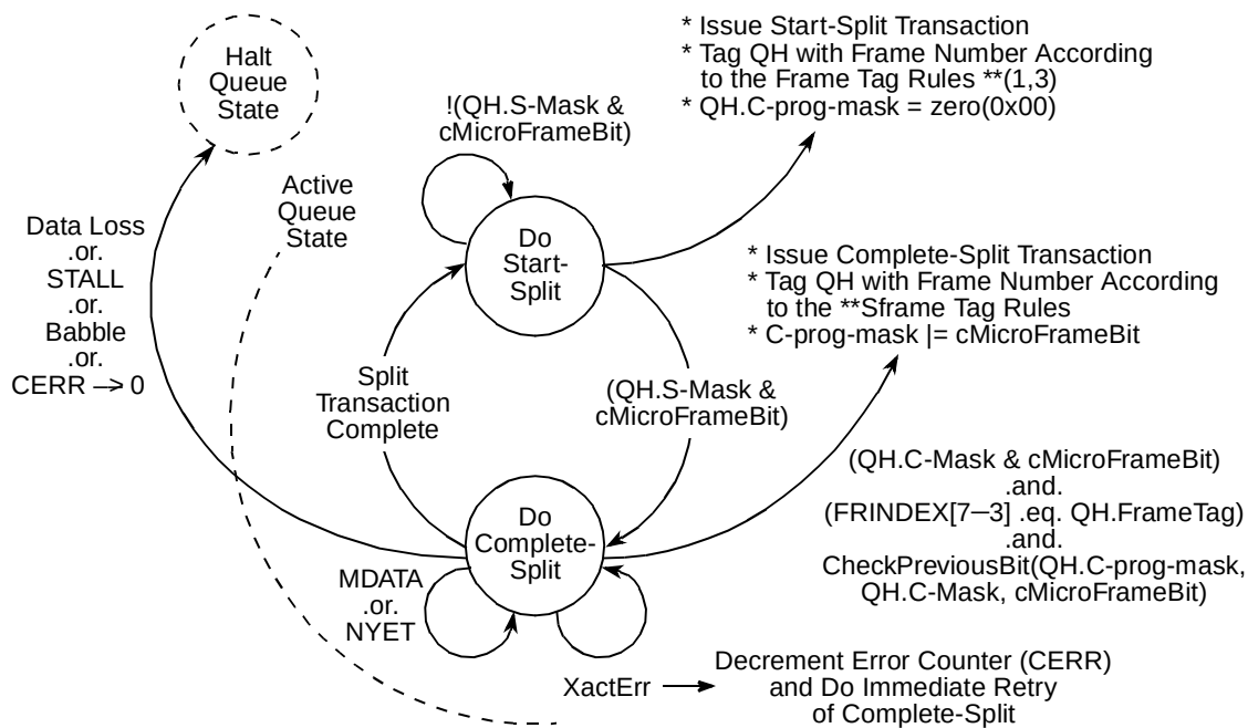
Figure 18-55. Split Transaction State Machine for Interrupt
