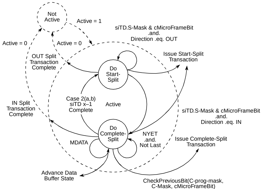
Figure 18-58. Split Transaction State Machine for Isochronous
