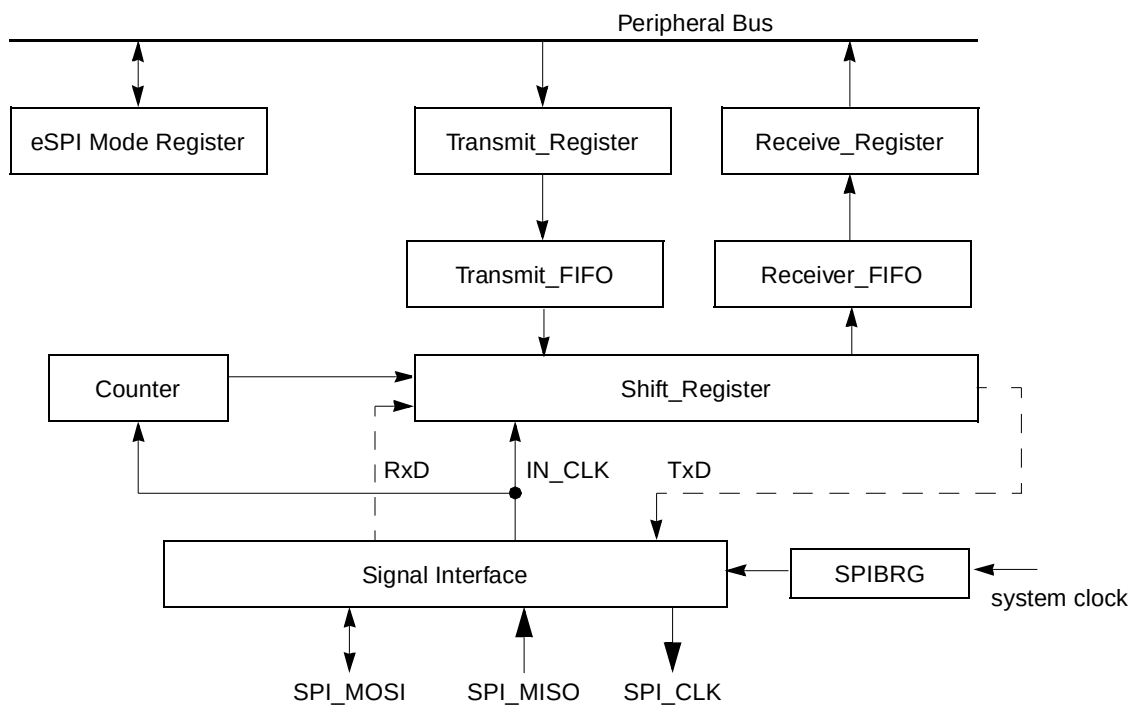
Figure 19-1. eSPI Block Diagram
