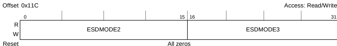
Figure 8-12. DDR SDRAM Mode 2 Configuration Register (DDR_SDRAM_MODE_2)
