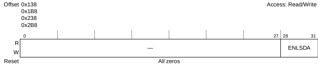
Figure 13-20. Extended Next List Descriptor Address Registers (ENLSDAR n )
