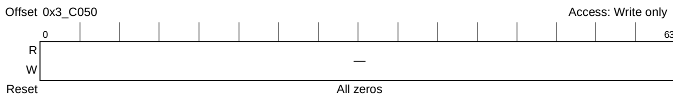
Figure 20-99. PKEU End of Message Register
