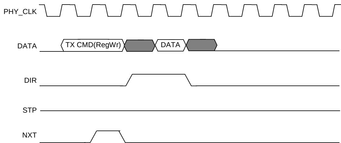
Figure 18-71. ULPI Register Read
