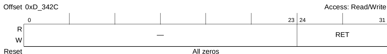
Figure 15-89. Outbound Doorbell Retry Error Threshold Configuration Register (ODRETCR)
