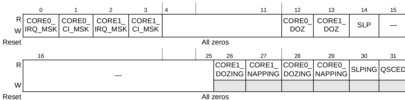
Figure 22-9. Power Management Control &amp; Status Register (POWMGTCSR)
