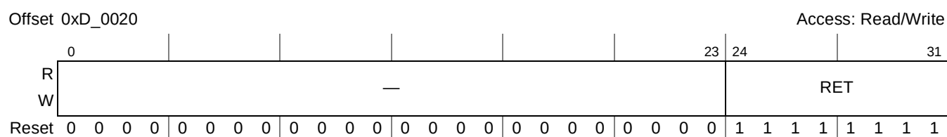
Figure 15-42. Logical Retry Error Threshold Configuration Register (LRETCR)
