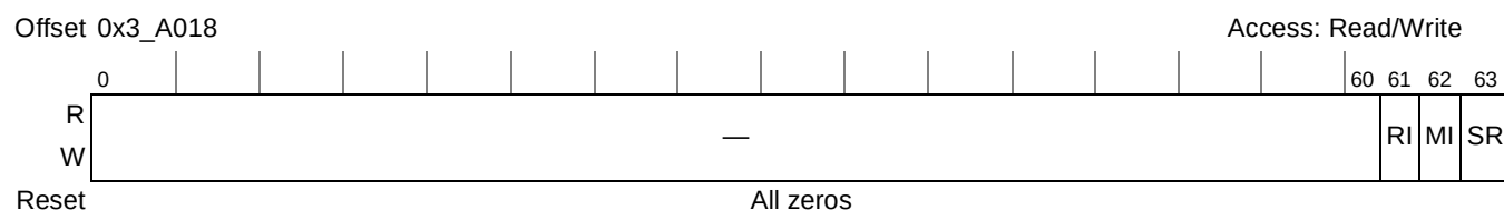
Figure 20-102. RNGU Reset Control Register
