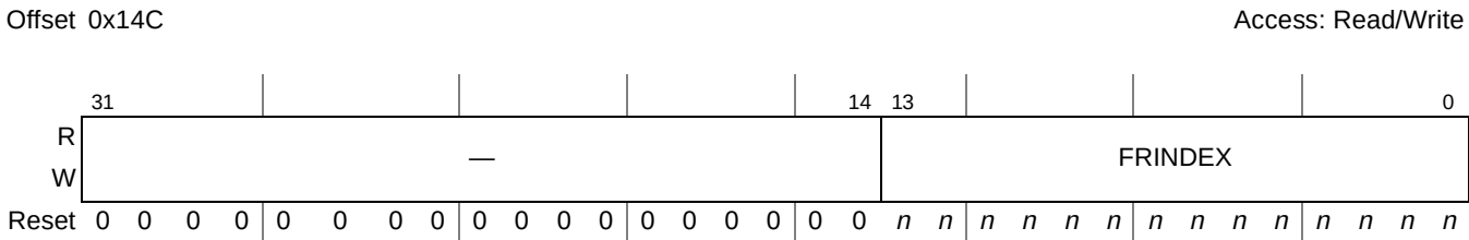
Figure 18-11. USB Frame Index (FRINDEX)
