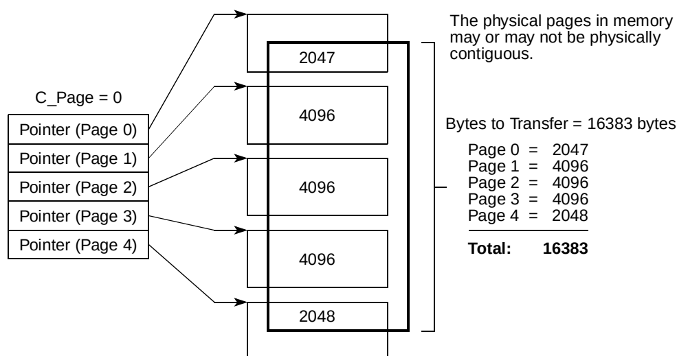
Figure 18-50. Example Mapping of qTD Buffer Pointers to Buffer Pages
