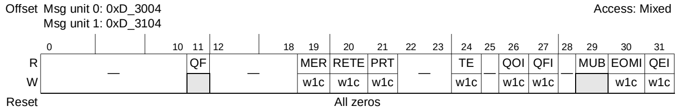
Figure 15-65. Outbound Message n Status Registers (OM n SR)
