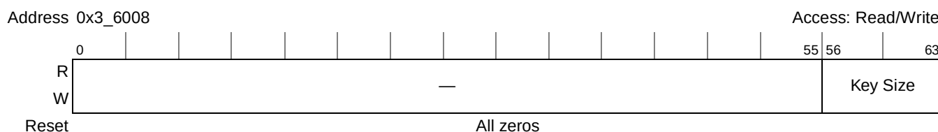
Figure 20-82. MDEU Key Size Register
