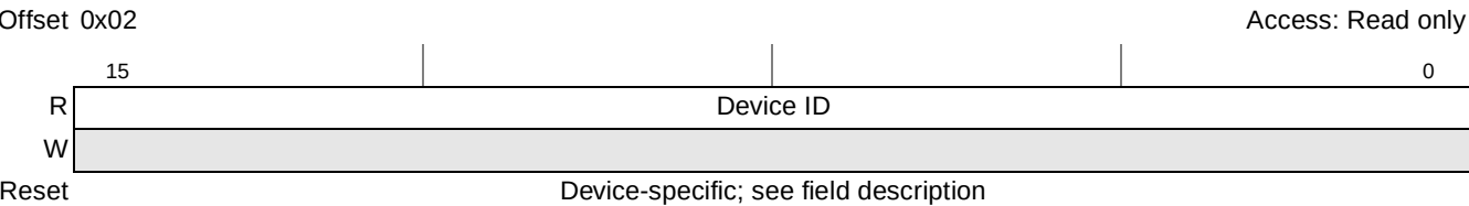
Figure 16-39. PCI Express Device ID Register
