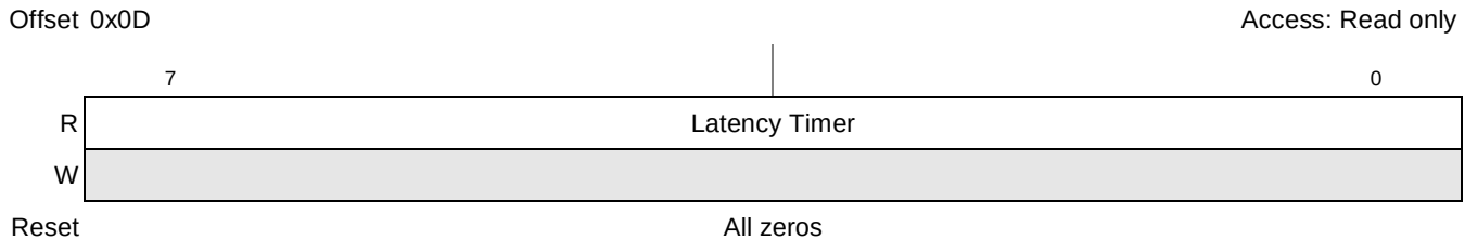
Figure 16-45. PCI Express Bus Latency Timer Register
