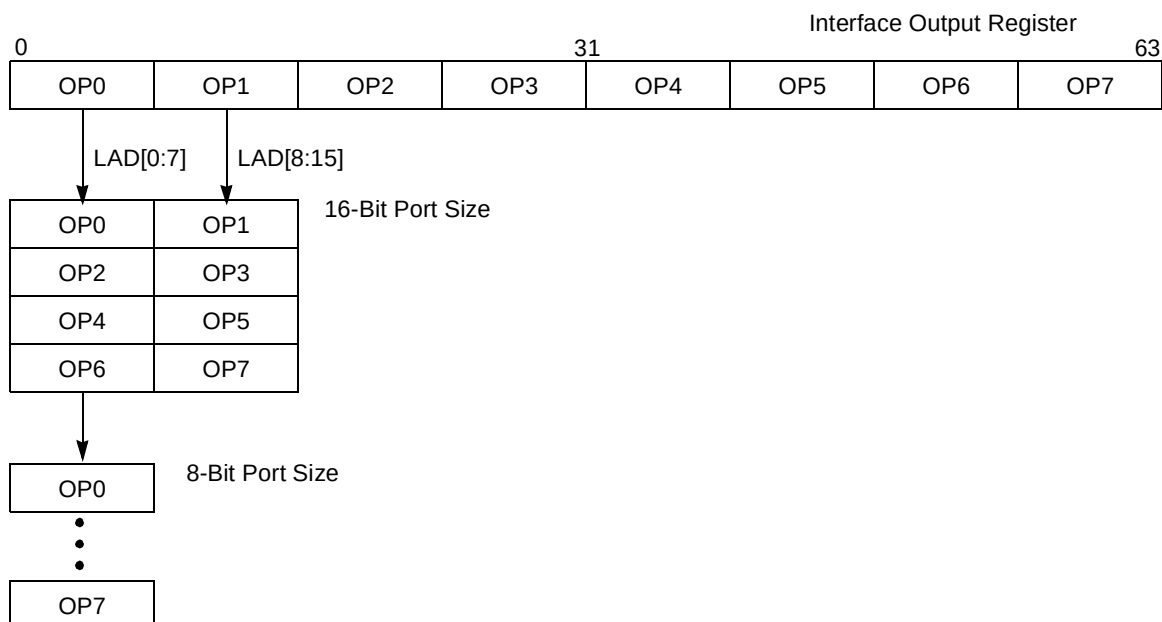
Figure 12-76. Interface to Different Port-Size Devices
