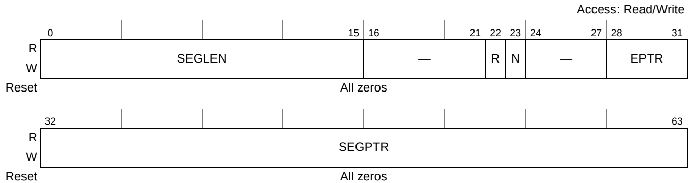
Figure 20-5. Link Table Entry
