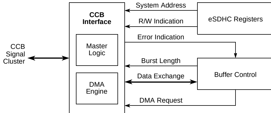
Figure 17-22. DMACCB Interface Block
