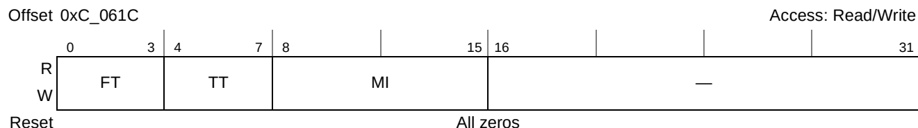
Figure 15-30. Logical/Transport Layer Control Capture Command and Status Register (LTLCCSR)
