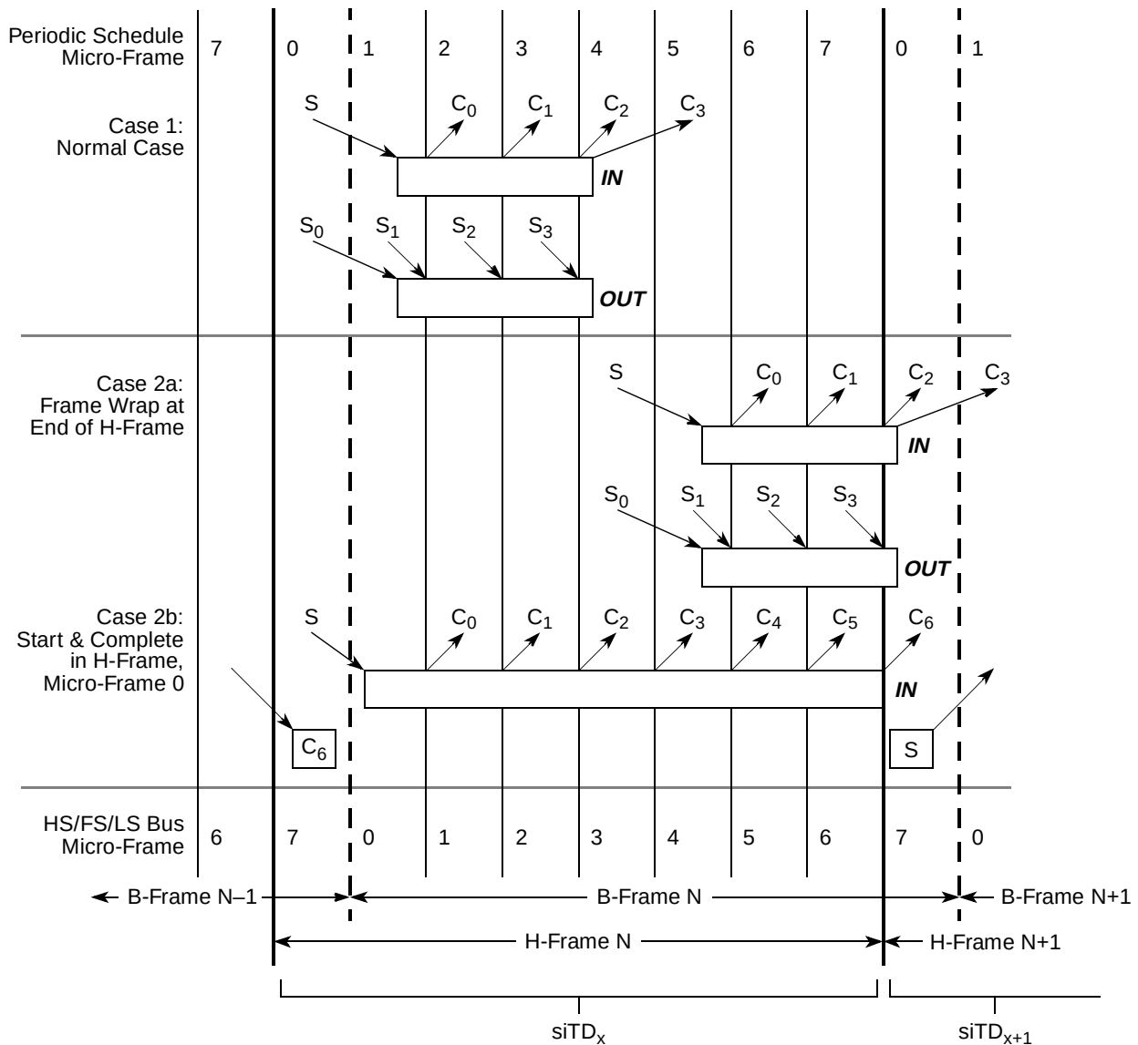
Figure 18-56. Split Transaction, Isochronous Scheduling Boundary Conditions
