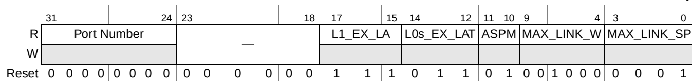
Figure 16-89. PCI Express Link Capabilities Register
