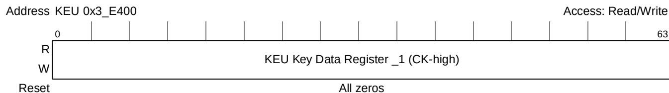
Figure 20-75. KEU Key Data Register _1 (CK-high)
