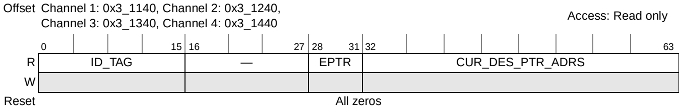
Figure 20-13. Current Descriptor Pointer Register
