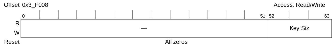
Figure 20-41. CRCU Key Size Register
