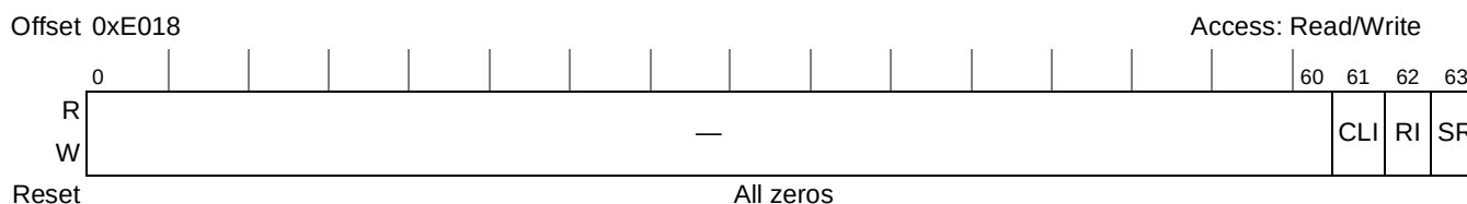
Figure 20-67. KEU Reset Control Register
