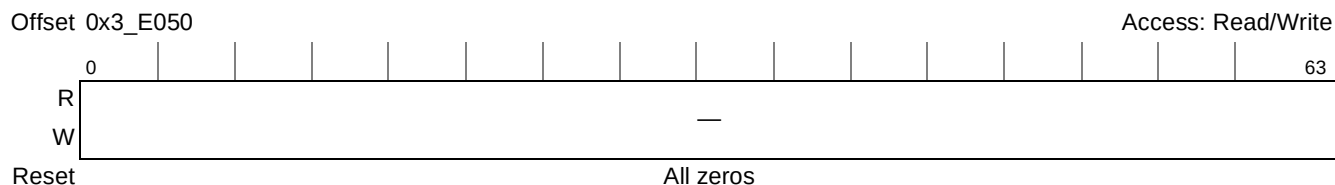
Figure 20-72. KEU End of Message Register
