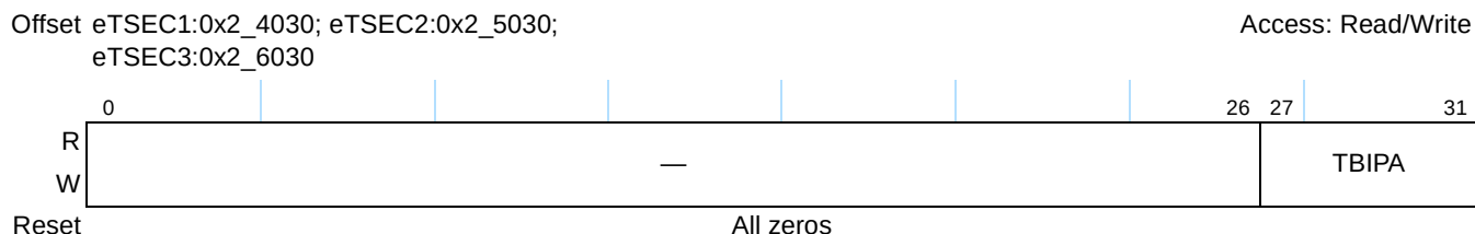
Figure 14-10. TBIPA Register Definition
