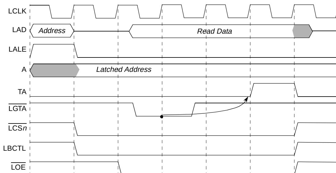
Figure 12-45. External Termination of GPCM Access
