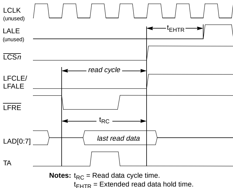
Figure 12-59. FCM Read Data Timing with Extended Hold Time (for TRLX = 0 , EHTR = 1 , RST = 1 , SCY = 1 )
