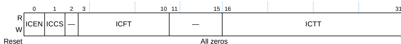
Figure 14-14. TXIC Register Definition
