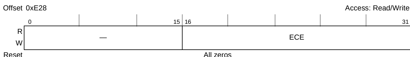
Figure 8-39. Memory Data Path Read Capture ECC Register (CAPTURE_ECC)
