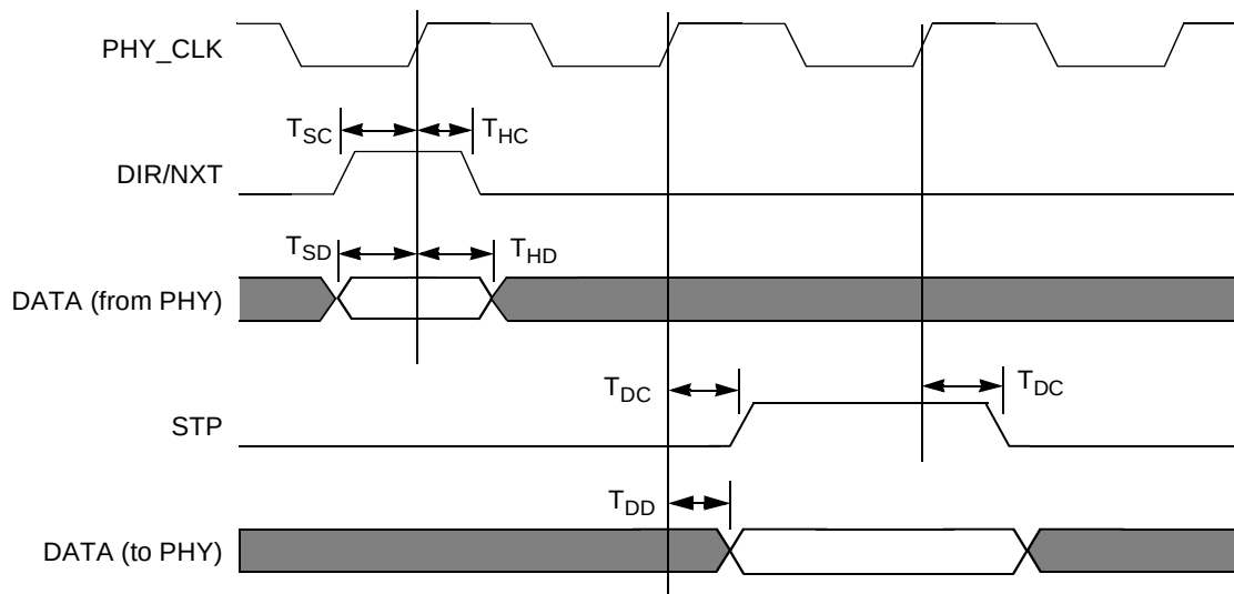
Figure 18-65. ULPI Timing
