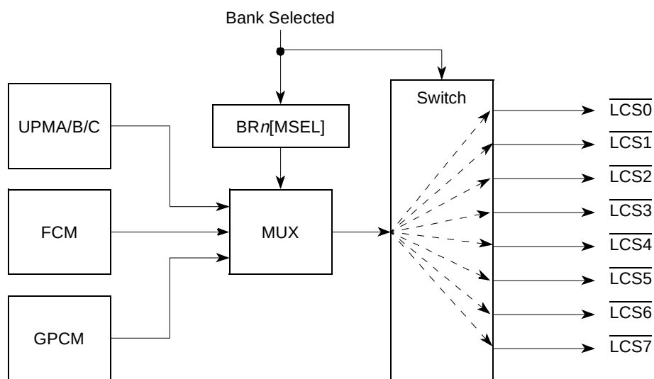
Figure 12-67. \overline{\text{LCS}}n Signal Selection
