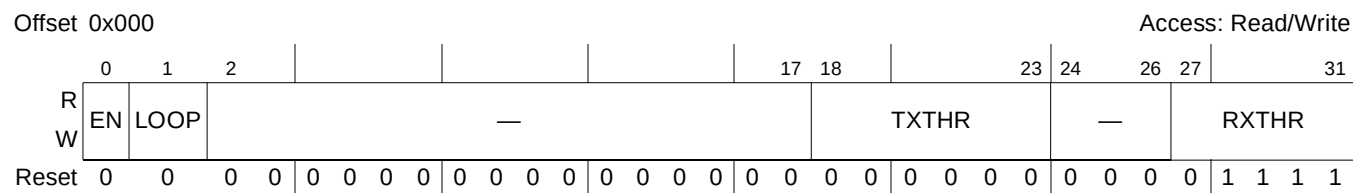
Figure 19-3. eSPI Mode Register (SPMODE)
