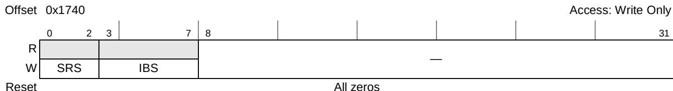
Figure 9-33. Shared Message Signaled Interrupt Index Register (MSIIR)
