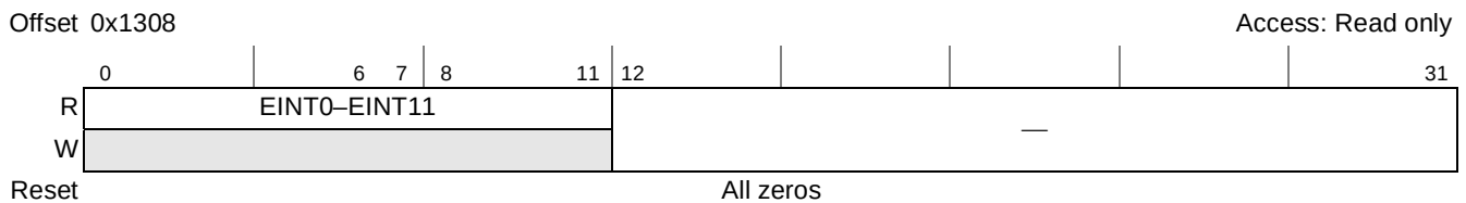
Figure 9-18. External Interrupt Summary Register (ERQSR)
