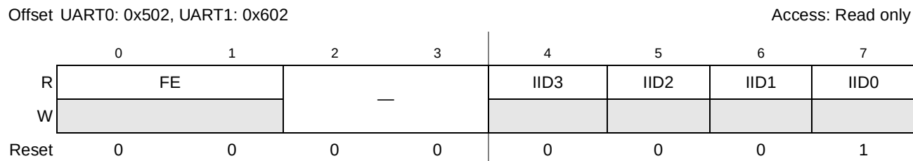
Figure 11-7. Interrupt ID Registers (UIIR)
