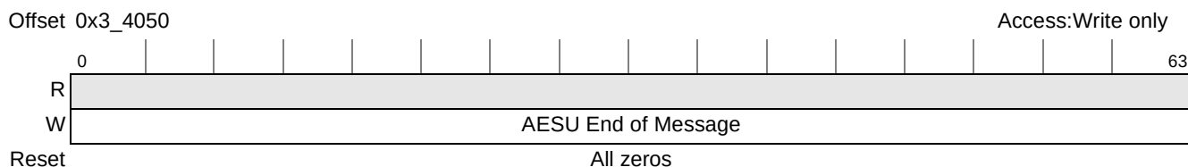
Figure 20-29. AESU End of Message Register
