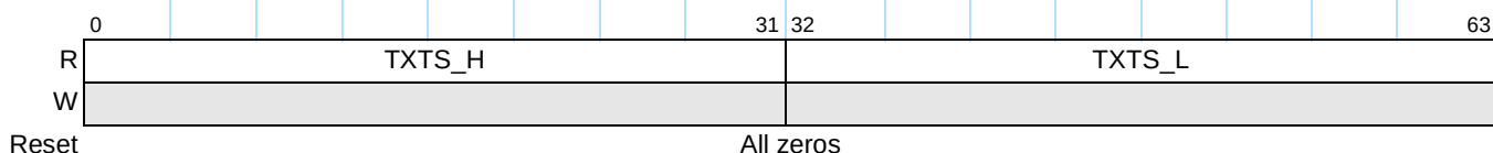
Figure 14-23. TMR_TXTSn_H/L Register Definition
