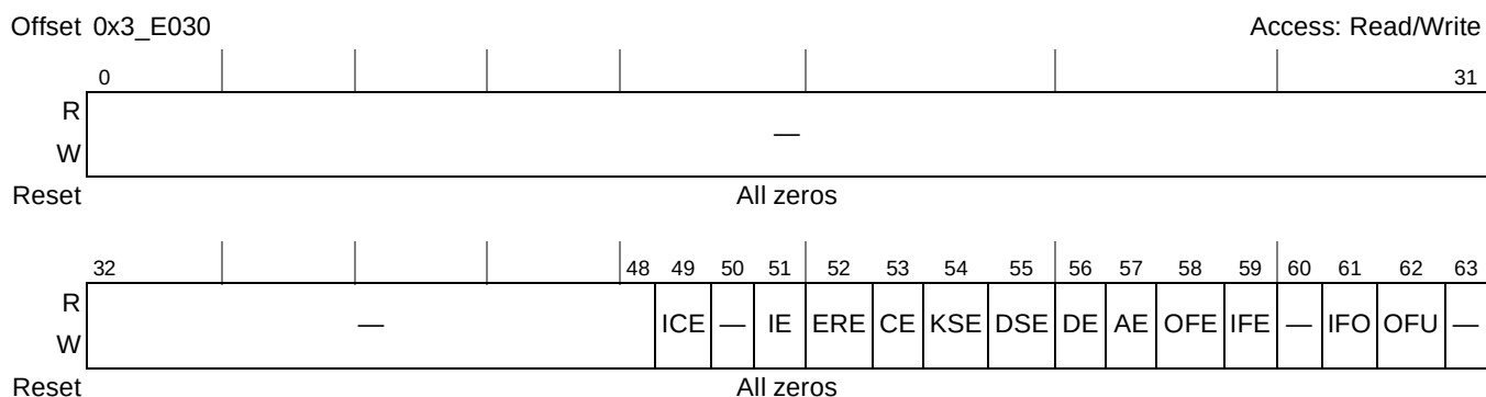
Figure 20-69. KEU Interrupt Status Register
