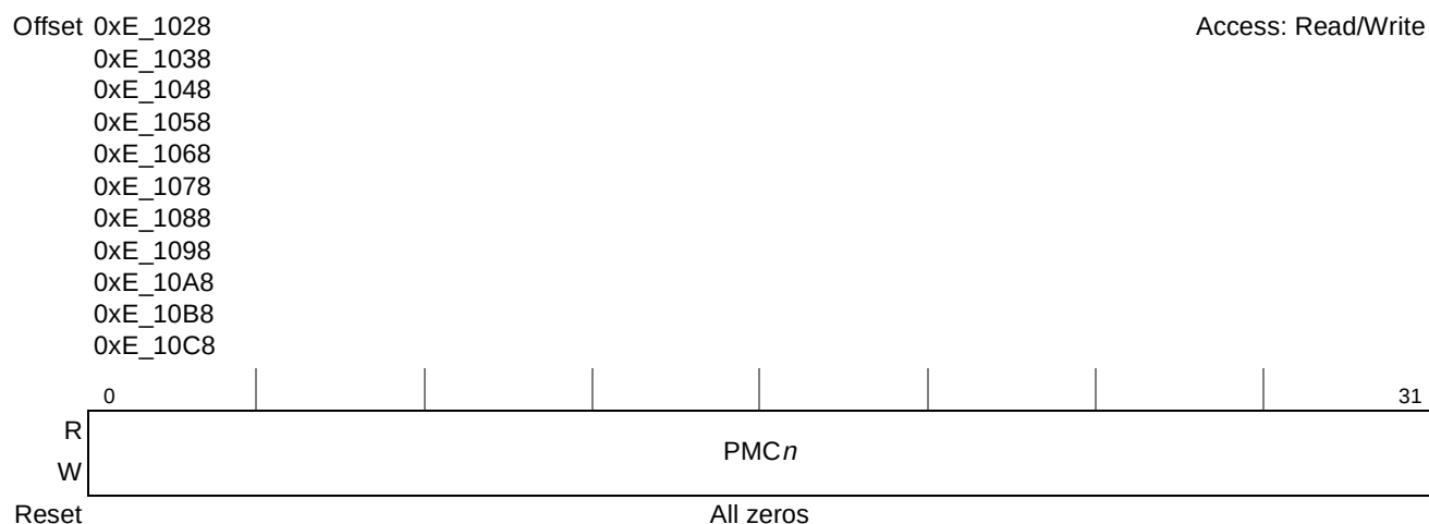
Figure 23-8. Performance Monitor Counter Register (PMC1–PMC11)
