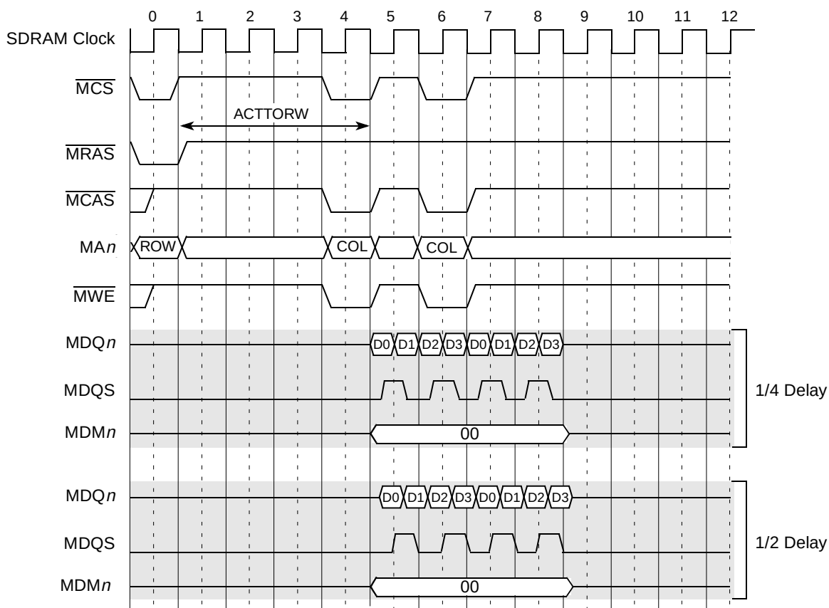
Figure 8-57. Write Timing Adjustments Example for Write Latency = 1
