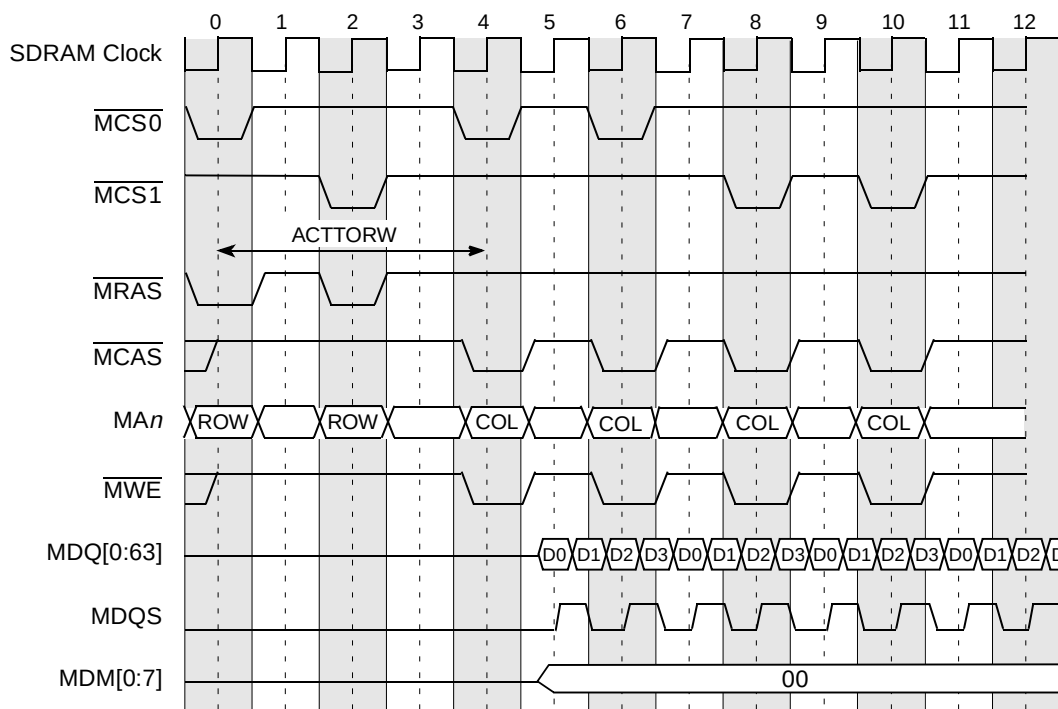
Figure 8-53. DDR SDRAM Single-Beat (Double Word) Write Timing—ACTTORW = 3
