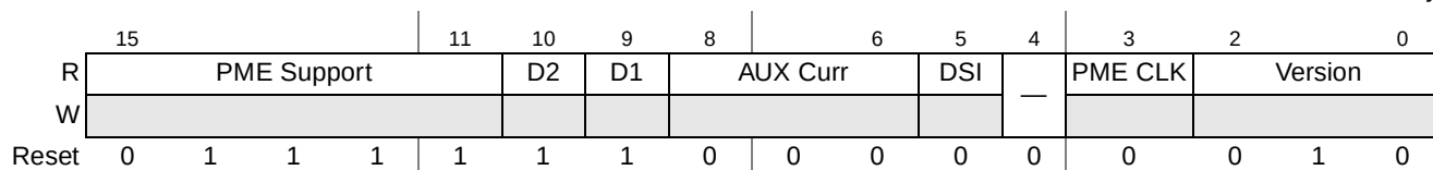
Figure 16-81. PCI Express Power Management Capabilities Register
