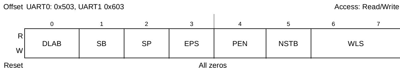
Figure 11-10. Line Control Register (ULCR)
