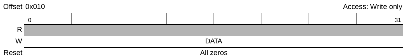
Figure 19-7. eSPI Transmit Data Register (SPITF)
