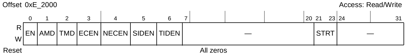
Figure 24-2. Watchpoint Monitor Control Register 0 (WMCR0)
