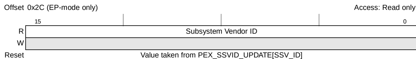
Figure 16-52. PCI Express Subsystem Vendor ID Register
