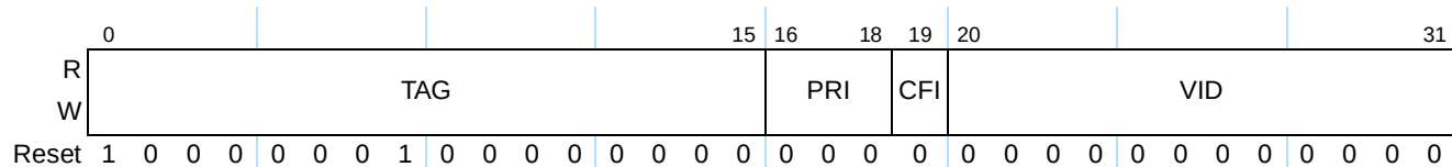
Figure 14-13. DFVLAN Register Definition
