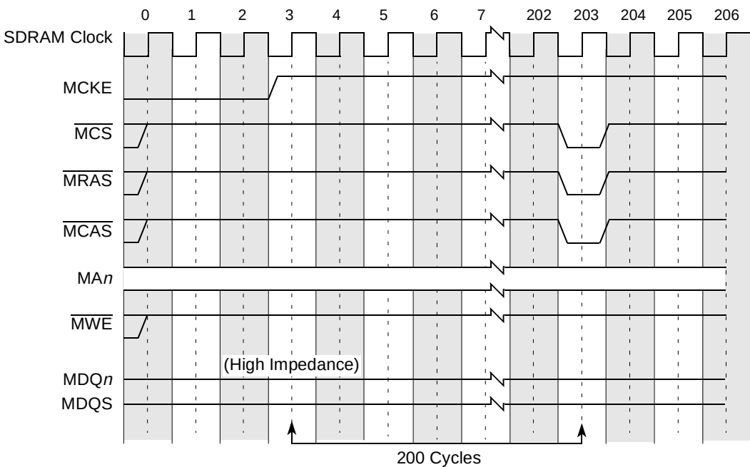
Figure 8-61. DDR SDRAM Self-Refresh Exit Timing
