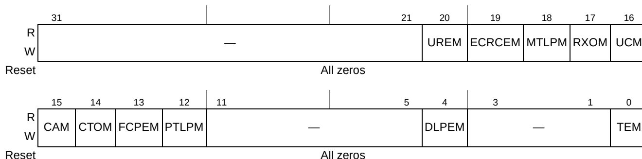
Figure 16-105. PCI Express Uncorrectable Error Mask Register
