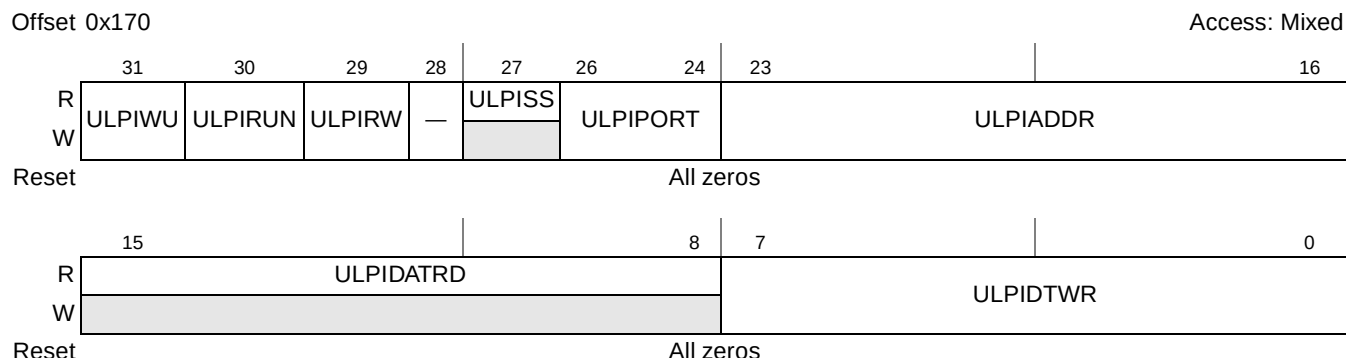
Figure 18-18. ULPI Register Access (ULPI VIEWPORT)
