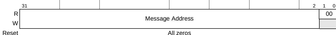
Figure 16-99. PCI Express MSI Message Address Register
