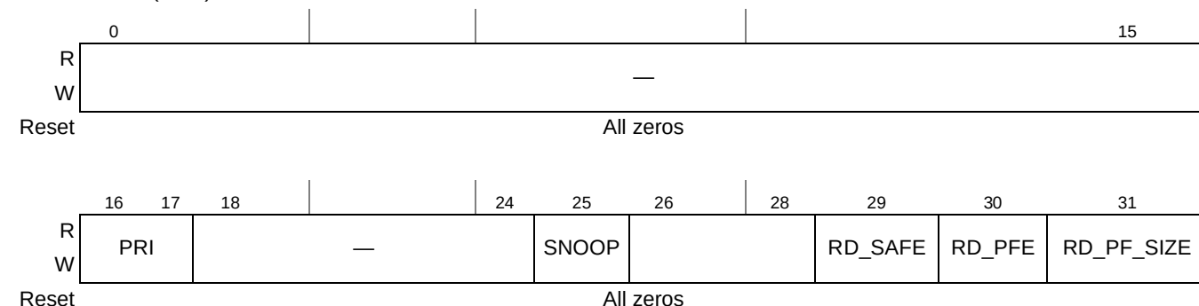
Figure 17-20. DMA Control Register (DCR)
