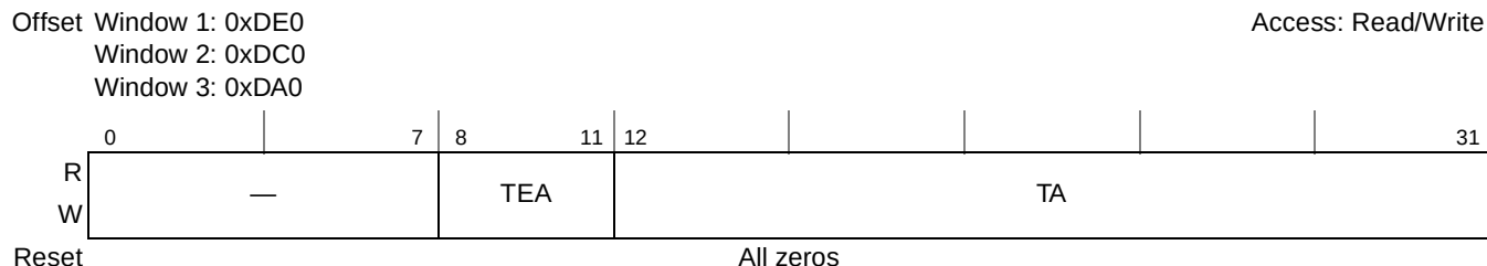
Figure 16-21. PCI Express Inbound Translation Address Registers (PEXITAR n )
