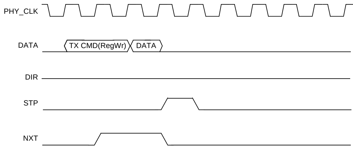
Figure 18-70. ULPI Register Write
