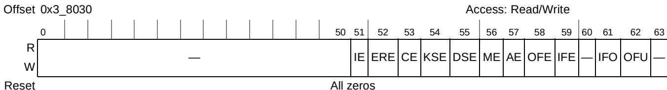
Figure 20-37. AFEU Interrupt Status Register
