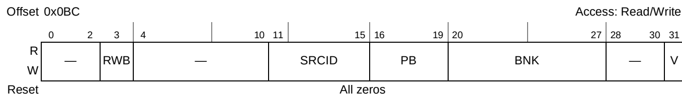
Figure 12-16. Transfer Error Attributes Register (LTEATR)
