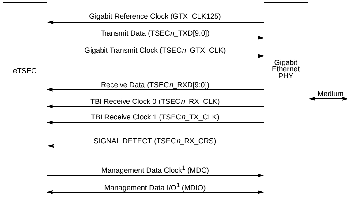
Figure 14-136. eTSEC-TBI Connection
