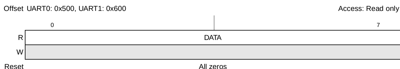
Figure 11-2. Receiver Buffer Registers (URBR n )
