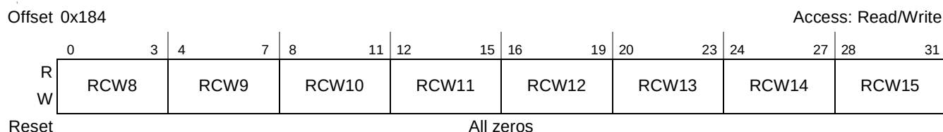
Figure 8-27. DDR Register Control Word 2 (DDR_SDRAM_RCW_2)
