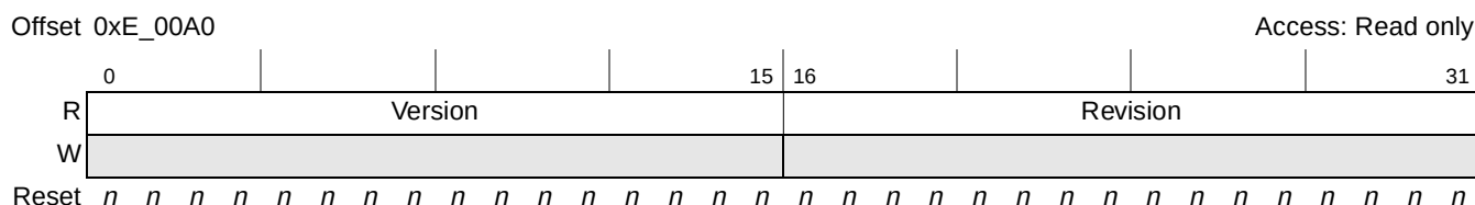
Figure 22-15. Processor Version Register (PVR)
