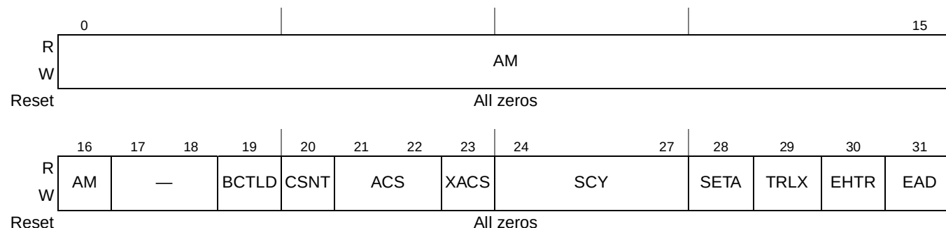
Figure 12-3. Option Registers (OR n ) in GPCM Mode
