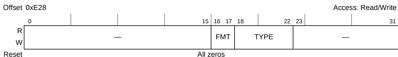
Figure 16-29. PCI Express Error Capture Register 0 (PEX_ERR_CAP_R0) Internal Source, Outbound Transaction
