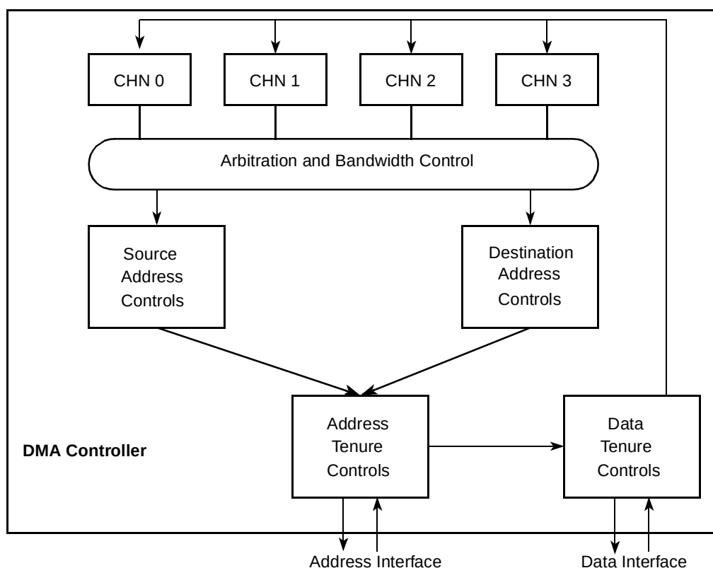
Figure 13-1. DMA Block Diagram
