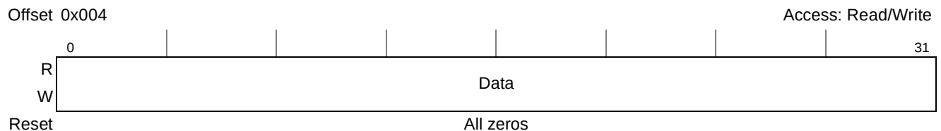
Figure 16-3. PCI Express Configuration Data Register (PEX_CONFIG_DATA)
