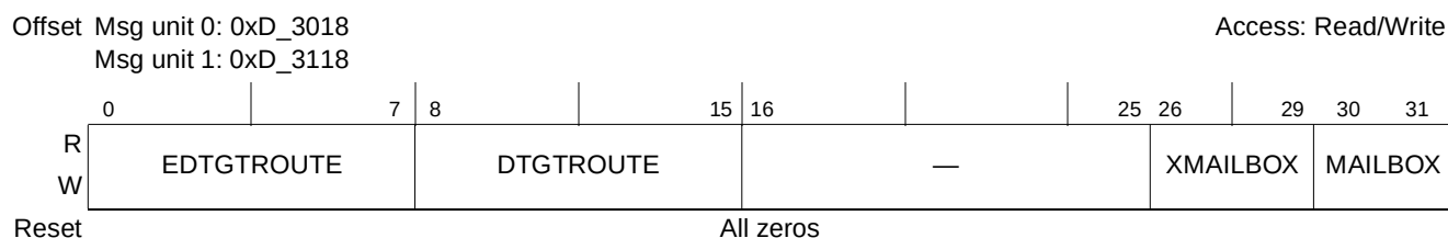
Figure 15-72. Outbound Message n Destination Port Registers (OM n DPR)
