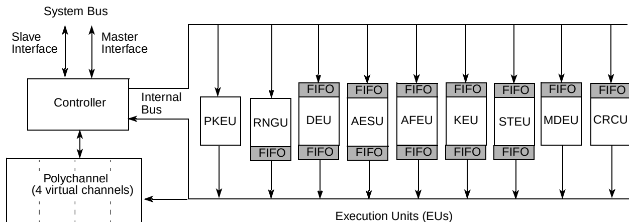
Figure 20-1. SEC Functional Modules
