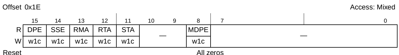
Figure 16-66. PCI Express Secondary Status Register
