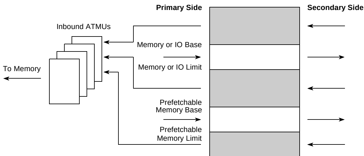
Figure 16-20. RC Inbound Transaction Flow
