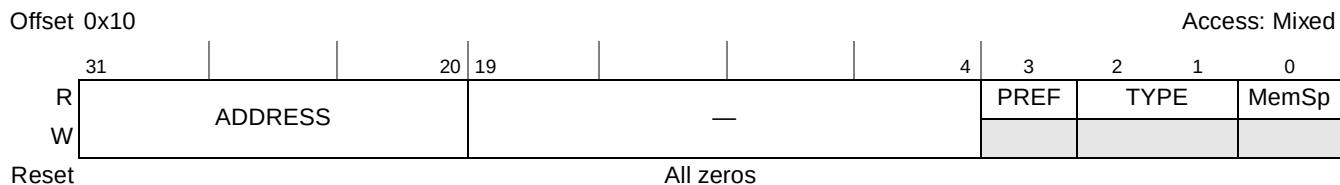
Figure 16-60. PCI Express Base Address Register 0 (PEXCSRBAR)
