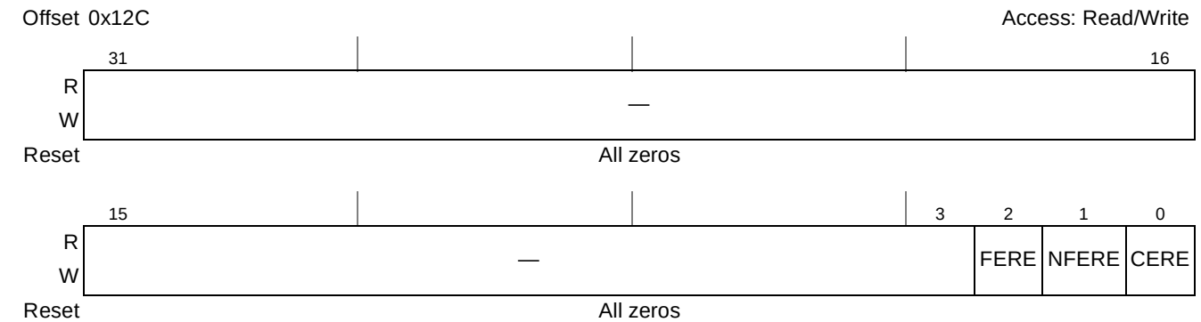
Figure 16-111. PCI Express Root Error Command Register
