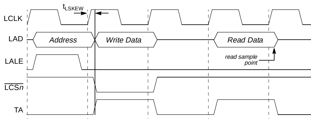
Figure 12-32. eLBC Bus Cycles in PLL Mode (GPCM and UPM only)
