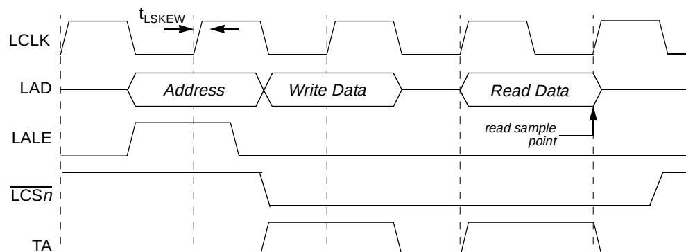
Figure 12-33. eLBC Bus Cycles in PLL-bypassed Mode (GPCM and UPM only)
