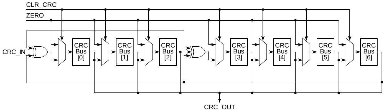
Figure 17-23. Command CRC Shift Register
