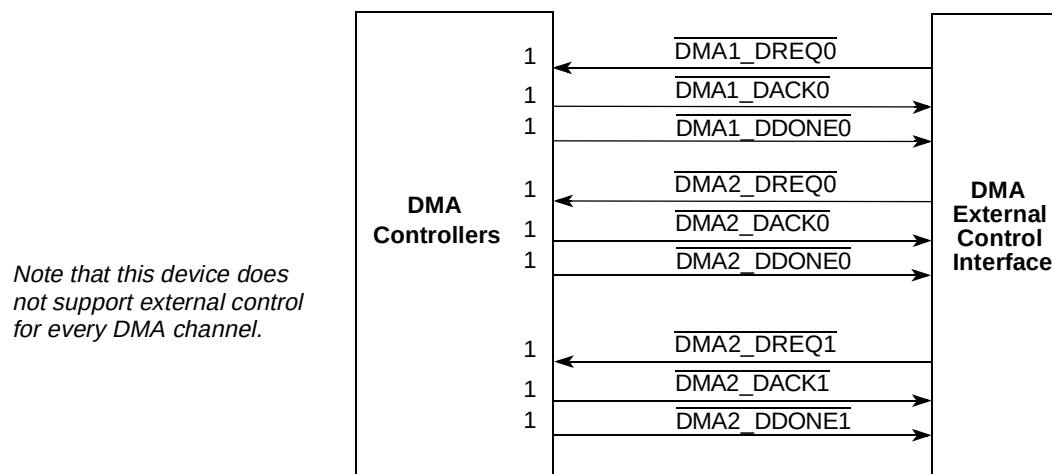
Figure 13-3. DMA Signal Summary
