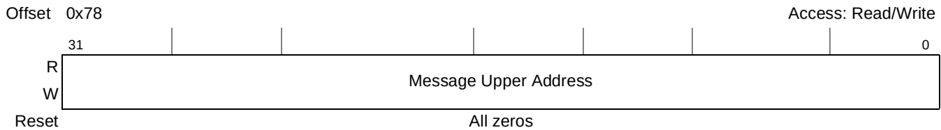
Figure 16-100. PCI Express MSI Message Upper Address Register
