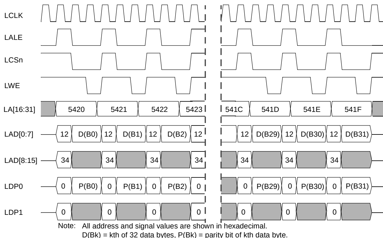
Figure 12-30. Example of 8-Bit GPCM Writing 32 Bytes to Address 0x1234_5420 (LCRR[PBYP] = 0)
