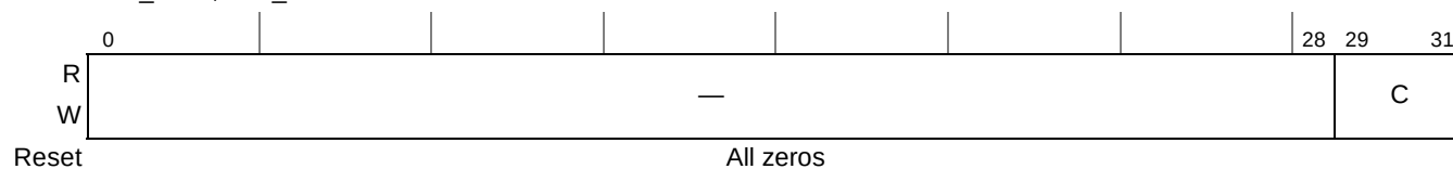
Figure 15-20. Port n Link Maintenance Request Command and Status Register (P n LMREQCSR)
