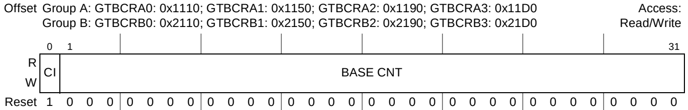
Figure 9-13. Global Timer Base Count Register (GTBCR xn )
