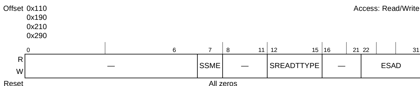
Figure 13-9. Source Attributes Registers (SATR n )
