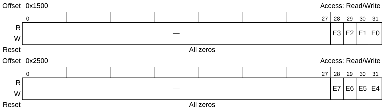
Figure 9-29. Message Enable Register (MER)
