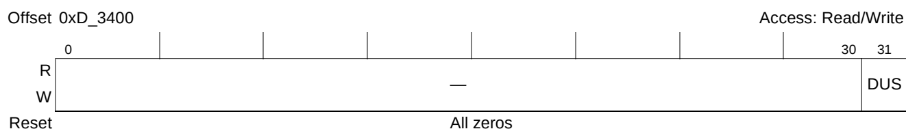
Figure 15-85. Outbound Mode Register (ODMR)
