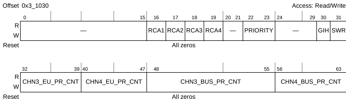
Figure 20-20. Master Control Register
