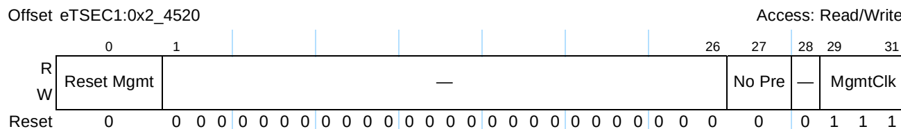
Figure 14-44. MII Management Configuration Register Definition
