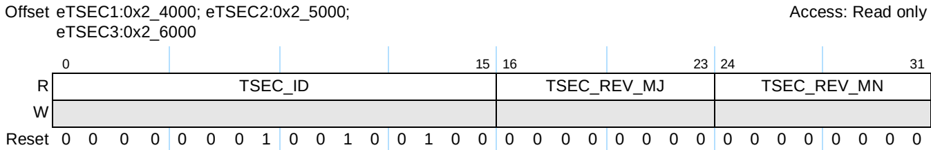
Figure 14-2. TSEC_ID Register
