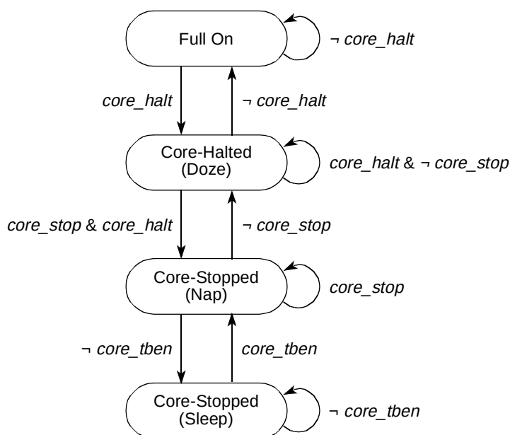
Figure 22-26. e500 Cores Power Management State Diagram
