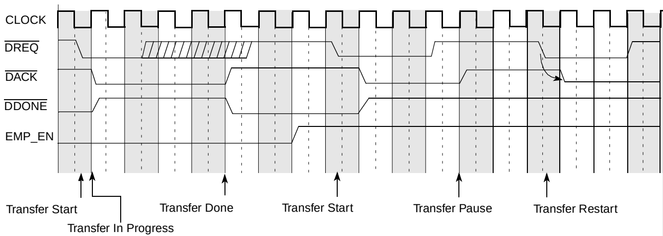
Figure 13-25. External Control Interface Timing
