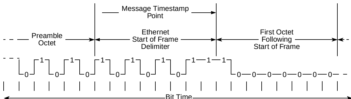
Figure 14-152. Ethernet Sampling Points for 1588
