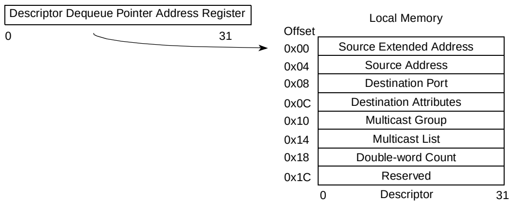
Figure 15-107. Descriptor Dequeue Pointer and Descriptor
