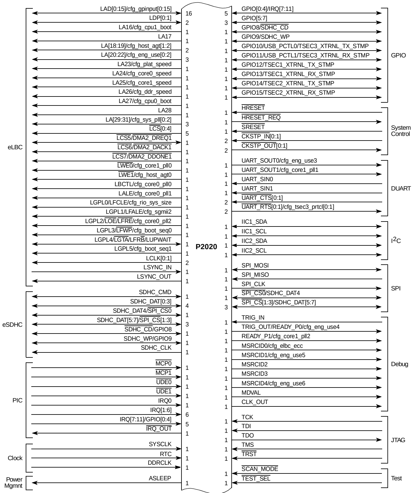
Figure 3-2. P2020 Signal Groupings (2/3) (Continued)
