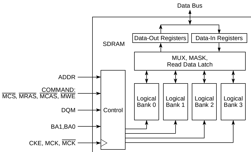
Figure 8-48. Typical Dual Data Rate SDRAM Internal Organization
