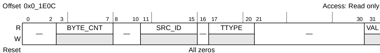
Figure 7-8. ECM Error Attributes Capture Register (EEATR)
