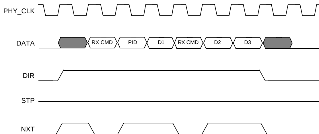
Figure 18-69. ULPI Data Receive
