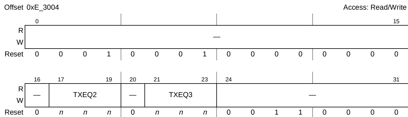
Figure 22-24. SRDS Control Register 1 (SRDSCR1)
