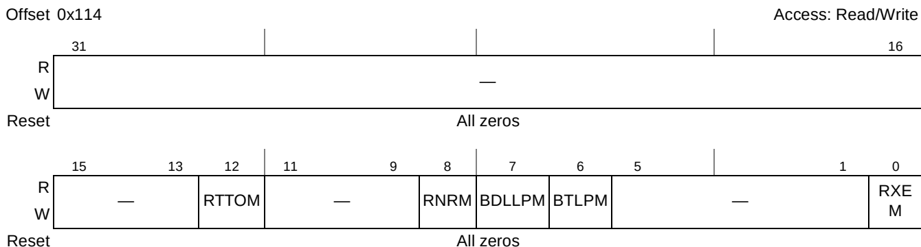
Figure 16-108. PCI Express Correctable Error Mask Register
