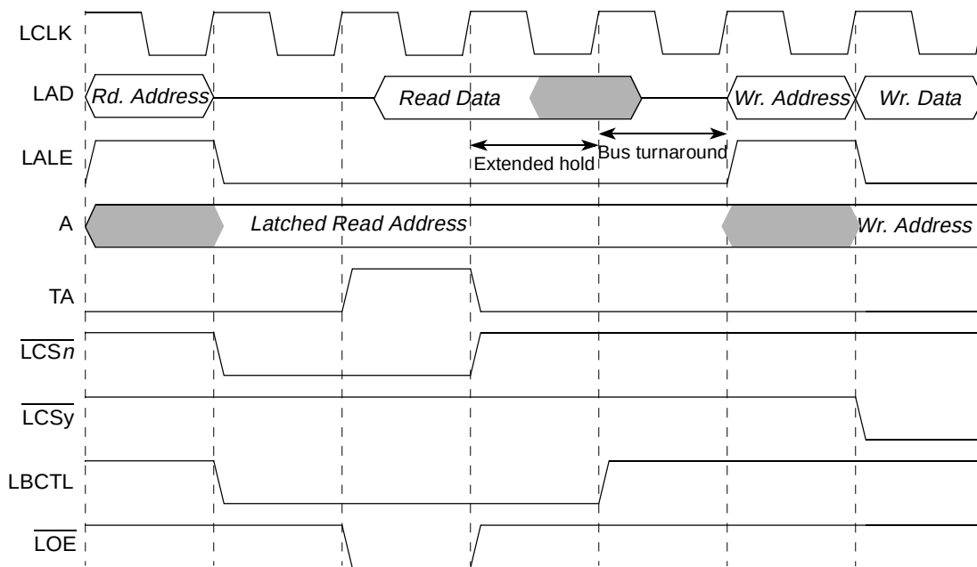
Figure 12-44. GPCM Read Followed by Write (TRLX = 0, EHTR = 1, One-Cycle Extended Hold Time on Reads)
