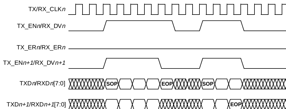
Figure 14-141. 16-Bit GMII-Style Packet FIFO Timing
