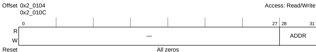
Figure 6-12. L2 Memory-Mapped SRAM Base Address Registers Extended Address 0–1 (L2SRBAREAn)
