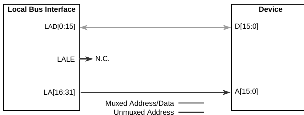
Figure 12-72. Non-Multiplexed Address and Data Buses
