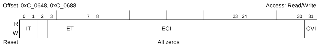
Figure 15-33. Port n Error Capture Attributes Command and Status Register ( PnECACSR )
