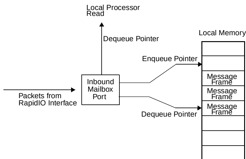
Figure 15-108. Inbound Message Structure
