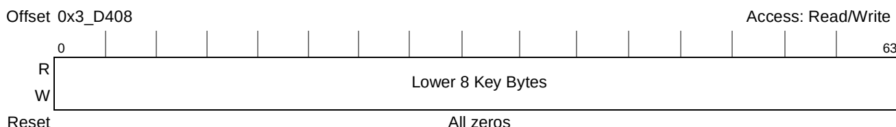
Figure 20-128. STEU Key Data Register 2
