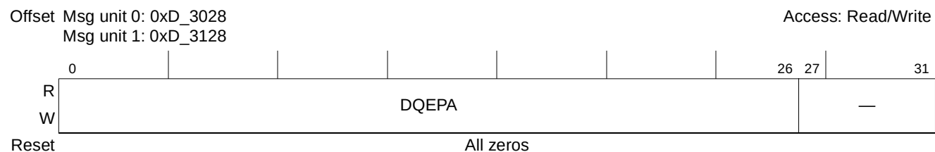
Figure 15-69. Outbound Message n Descriptor Queue Enqueue Pointer Registers (OM n DQEPAR)
