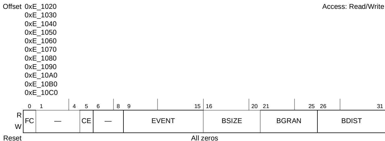
Figure 23-4. Performance Monitor Local Control A Registers (PMLCA1–PMLCA11)
