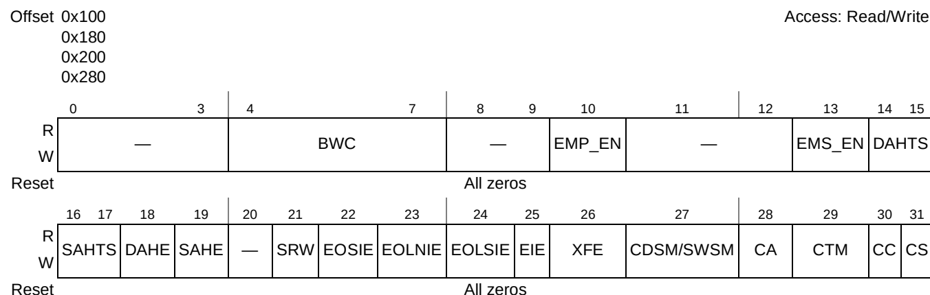
Figure 13-4. DMA Mode Registers (MR n )
