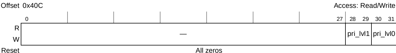
Figure 18-31. Priority Control (PRI CTRL)
