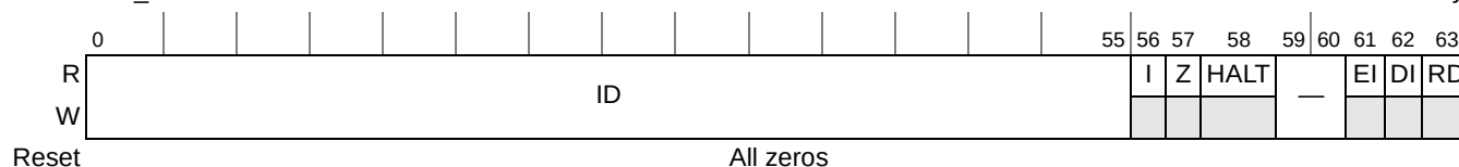
Figure 20-96. PKEU Status Register
