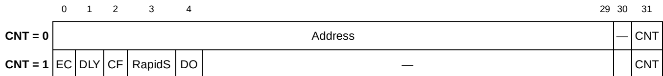
Figure 4-12. Config Address Fields
