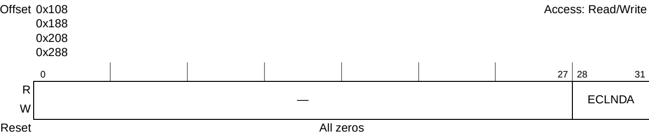
Figure 13-7. Extended Current Link Descriptor Address Registers (ECLNDAR n )
