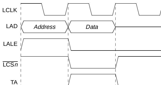
Figure 12-31. Basic eLBC Bus Cycle with LALE, TA, and \overline{\text{LCSn}}
