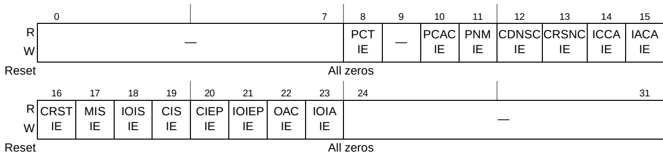
Figure 16-26. PCI Express Error Interrupt Enable Register (PEX_ERR_EN)
