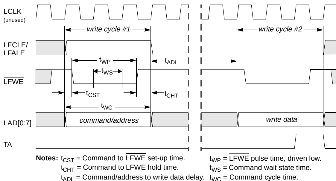
Figure 12-54. Timing of FCM Command/Address and Write Data Cycles (for TRLX = 0 , CHT = 0 , CST = 1 , SCY = 1 )
