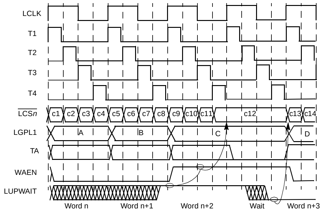
Figure 12-70. Effect of LUPWAIT Signal
