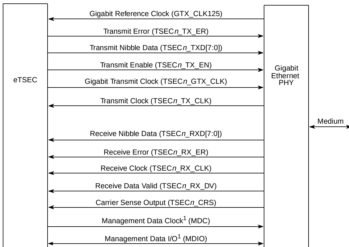
Figure 14-134. eTSEC-GMII Connection
