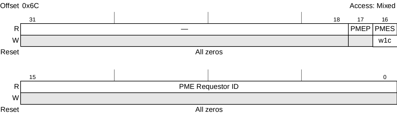
Figure 16-96. PCI Express Root Status Register
