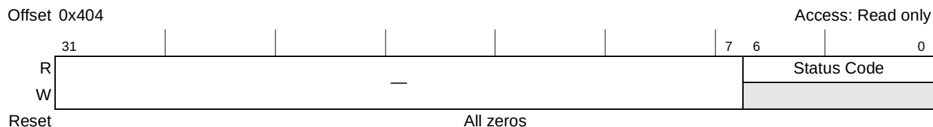
Figure 16-115. PCI Express LTSSM State Status Register (PEX_LTSSM_STAT)
