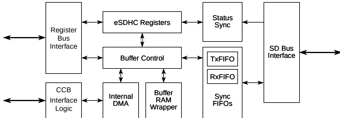
Figure 17-21. eSDHC Buffer Scheme
