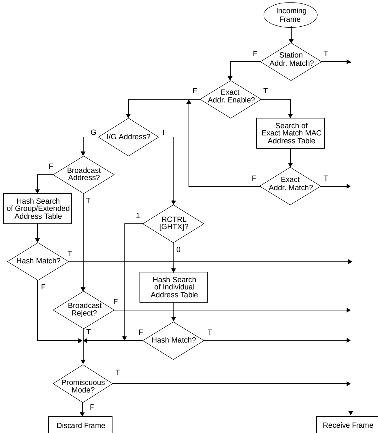
Figure 14-145. Ethernet Address Recognition Flowchart
