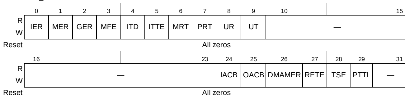
Figure 15-27. Logical/Transport Layer Error Enable Command and Status Register (LTLEECR)
