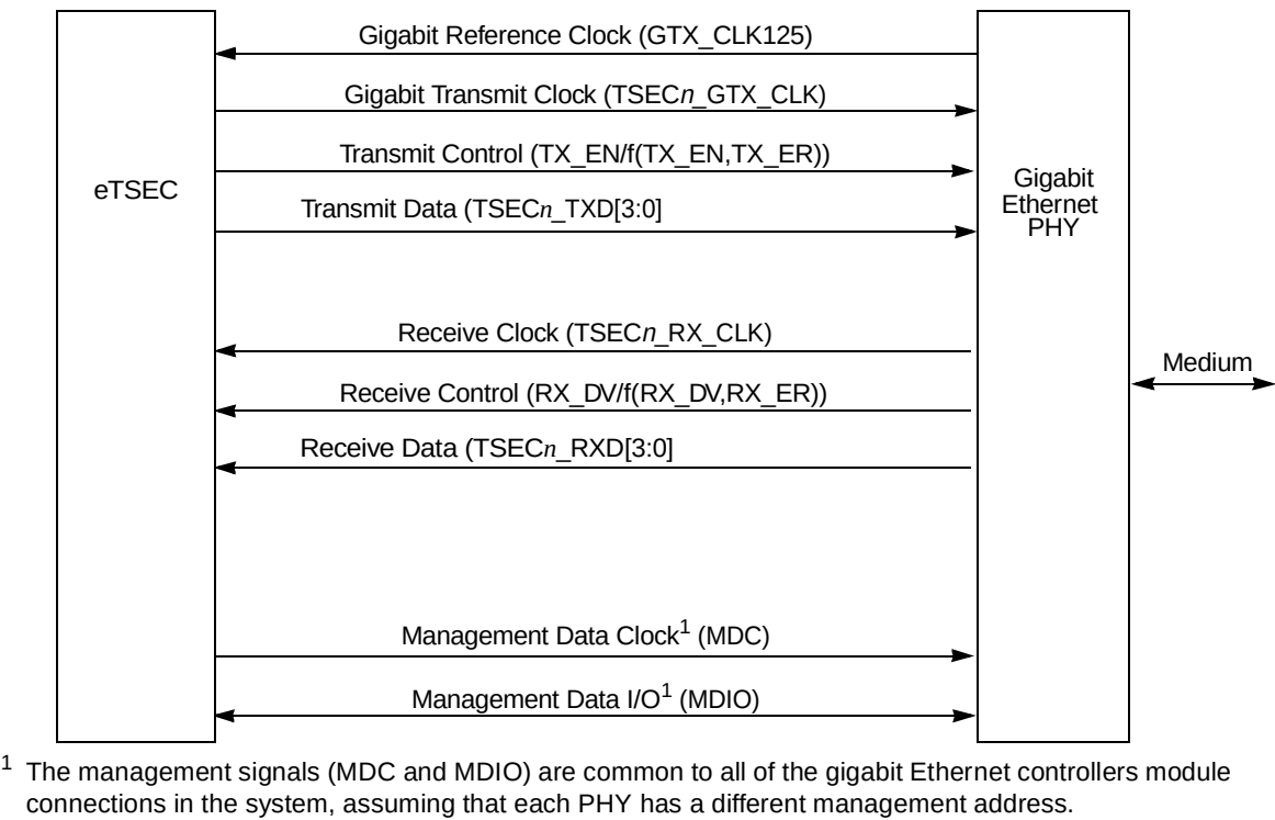
Figure 14-135. eTSEC-RGMII Connection
