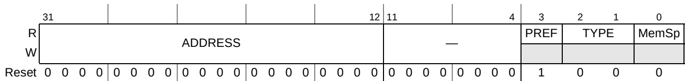
Figure 16-49. 32-Bit Memory Base Address Register (BAR1)
