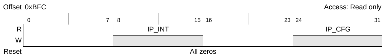
Figure 16-12. IP Block Revision Register 2
