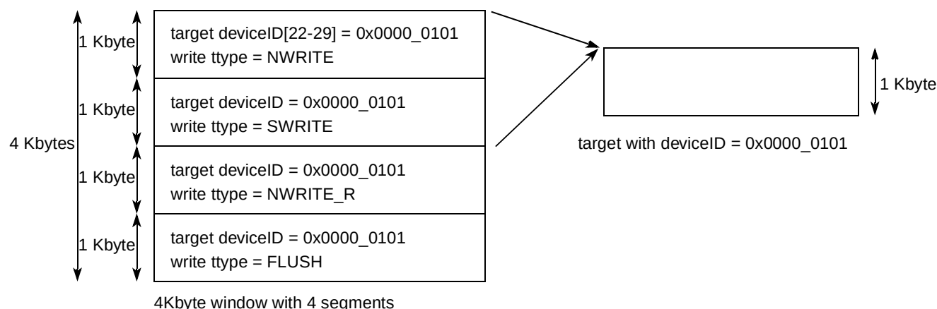
Figure 15-53. Example of Attribute Aliasing
