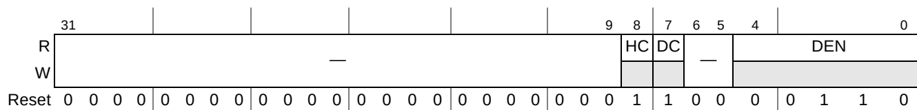
Figure 18-7. Device Control Capability Parameters (DCCPARAMS)
