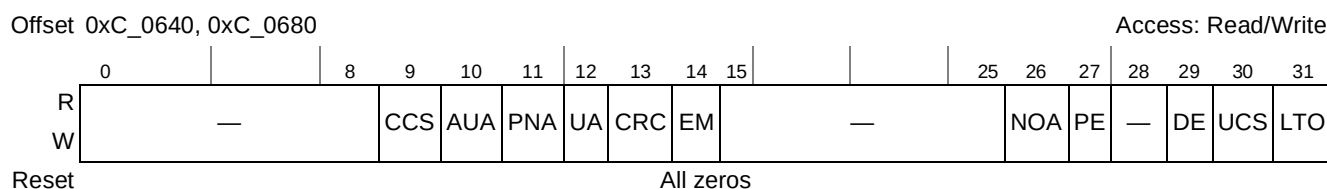
Figure 15-31. Port n Error Detect Command and Status Register (PnEDCSR)
