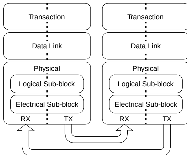
Figure 16-124. PCI Express High-Level Layering
