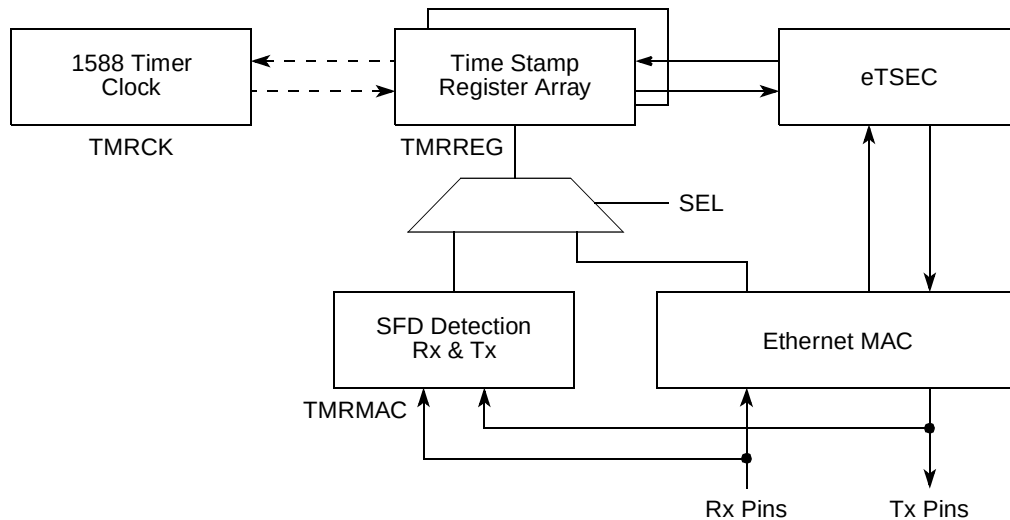
Figure 14-151. 1588 Timer Design Partition
