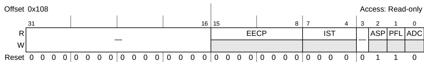
Figure 18-5. Host Control Capability Parameters (HCCPARAMS)
