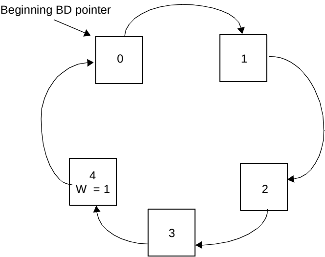
Figure 14-157. Buffer Descriptor Ring
