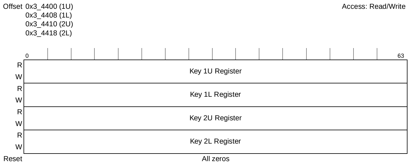
Figure 20-31. AESU Key Registers
