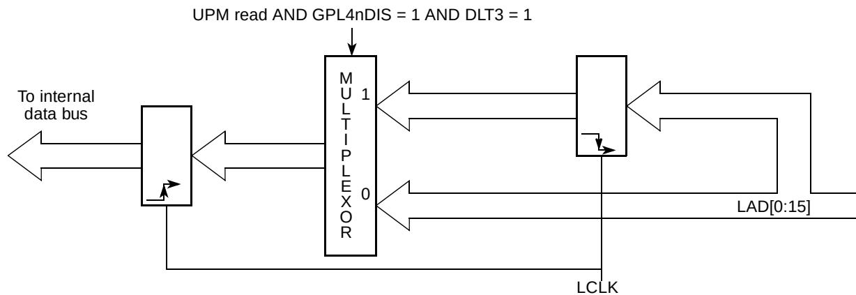
Figure 12-69. UPM Read Access Data Sampling
