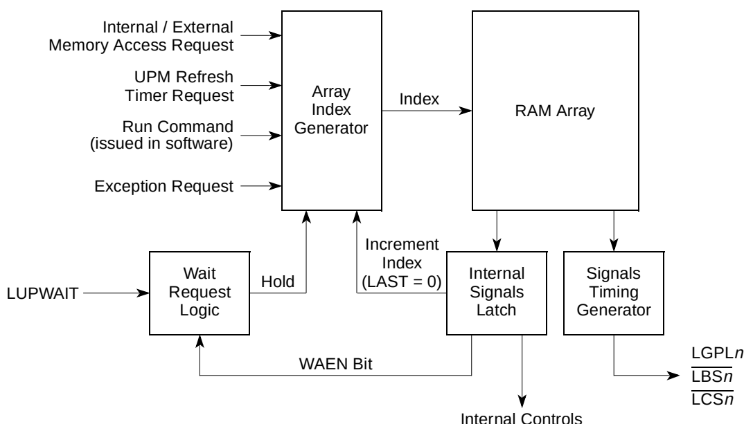
Figure 12-61. User-Programmable Machine Functional Block Diagram
