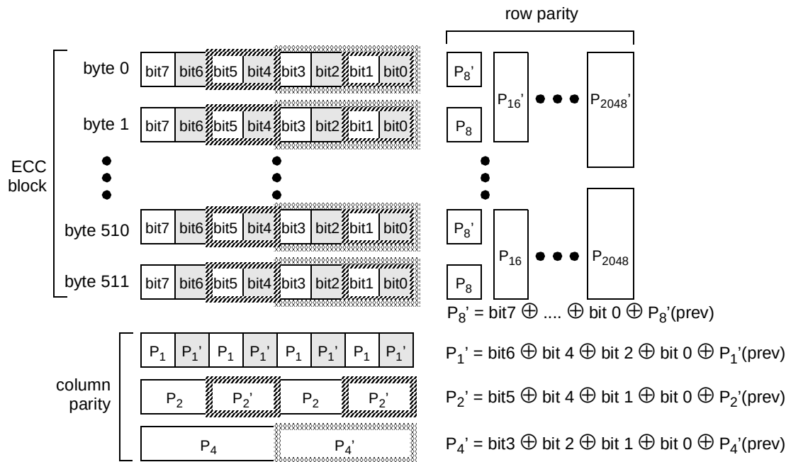
Figure 12-50. FCM ECC Calculation
