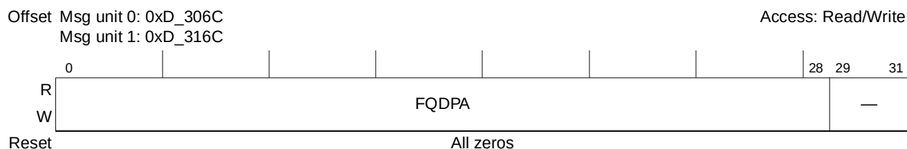
Figure 15-81. Inbound Message n Frame Queue Dequeue Pointer Address Registers (IM n FQDPA)
