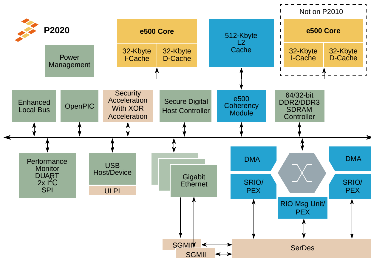
Figure 1-1. P2020/P2010 Block Diagram
