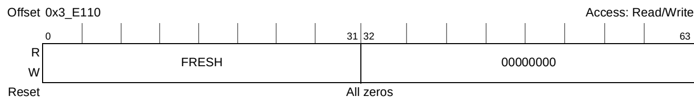
Figure 20-74. KEU IV_2 Register (FRESH)
