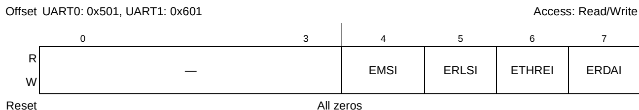
Figure 11-6. Interrupt Enable Register (UIER)
