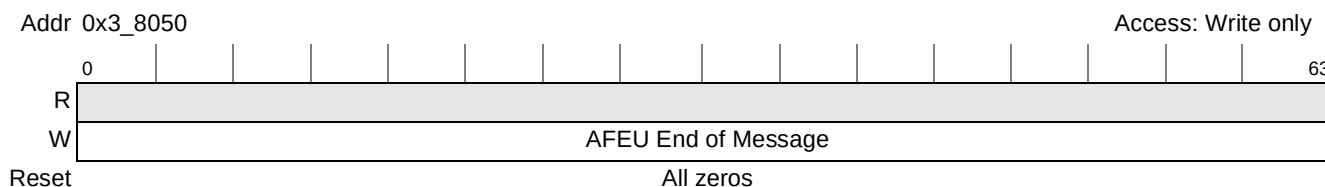
Figure 20-39. AFEU End of Message Register
