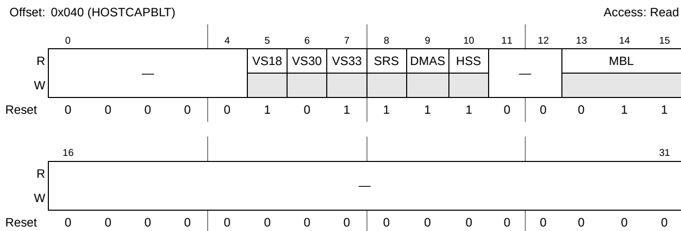
Figure 17-16. Host Capabilities Register (HOSTCAPBLT)
