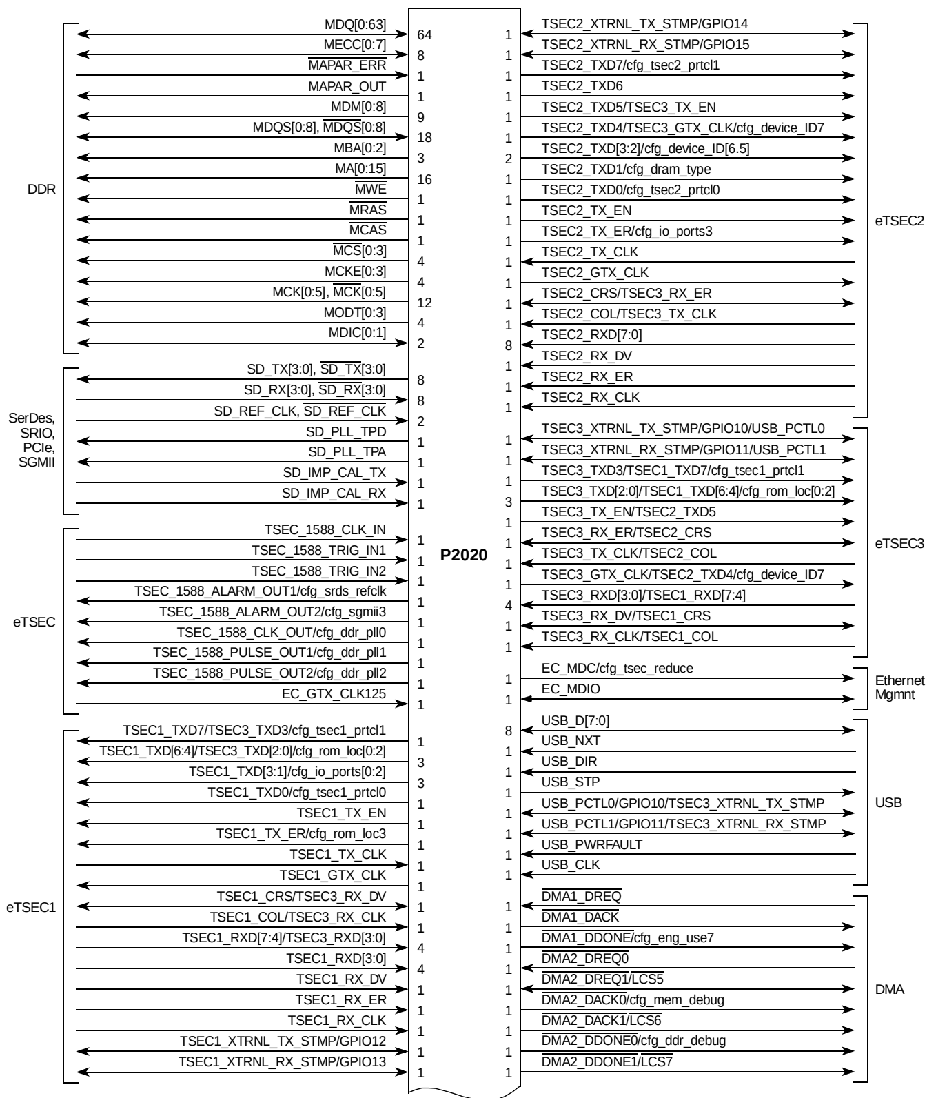
Figure 3-1. P2020 Signal Groupings (1/3)
