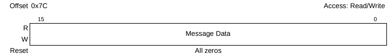
Figure 16-101. PCI Express MSI Message Data Register
