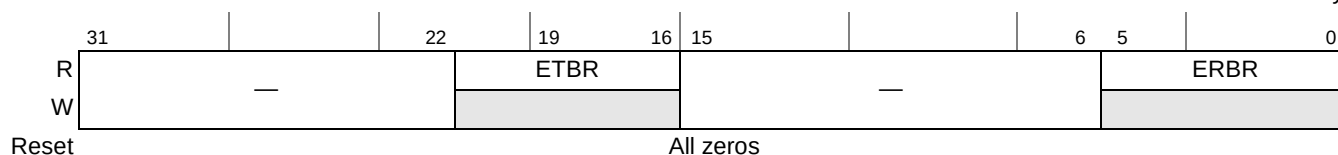
Figure 18-25. Endpoint Status (ENDPTSTATUS)
