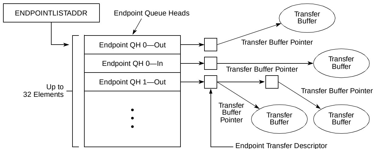
Figure 18-63. Endpoint Queue Head Diagram
