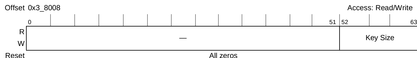
Figure 20-33. AFEU Key Size Register
