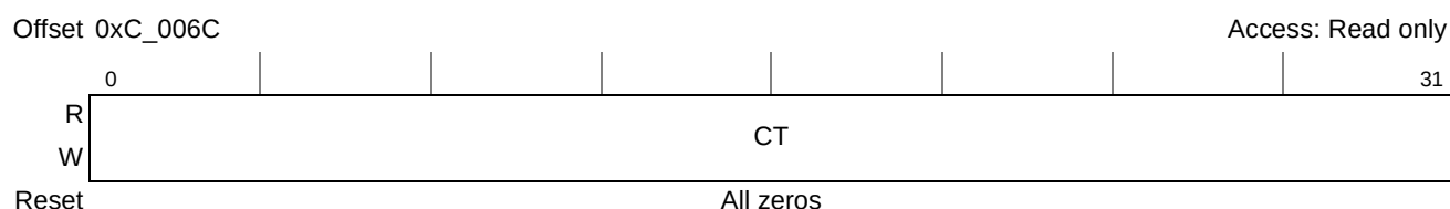
Figure 15-15. Component Tag Command and Status Register (CTCSR)
