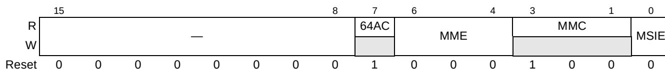
Figure 16-98. PCI Express MSI Message Control Register
