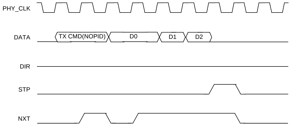
Figure 18-67. ULPI Data Transmit (NOPID)
