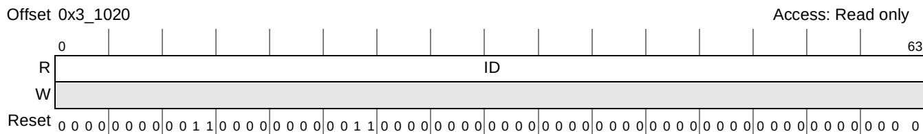
Figure 20-18. ID Register
