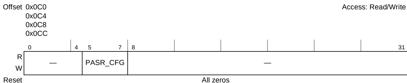
Figure 8-4. Chip Select Configuration Register 2 (CS n _CONFIG_2)
