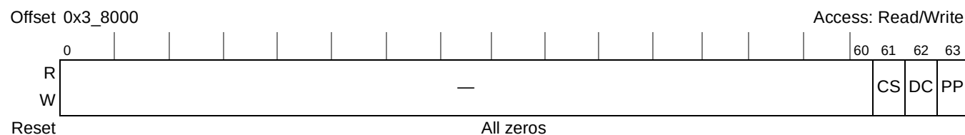
Figure 20-32. AFEU Mode Register
