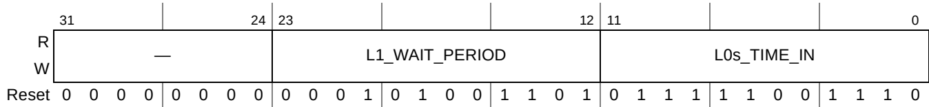
Figure 16-117. PCI Express Power Management Timer Register (PEX_PM_TIMER)
