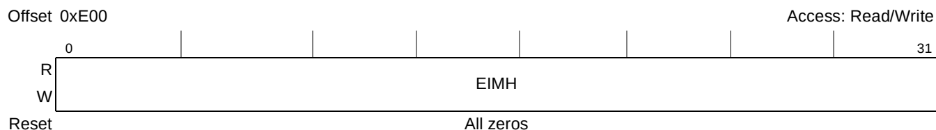
Figure 8-34. Memory Data Path Error Injection Mask High Register (DATA_ERR_INJECT_HI)
