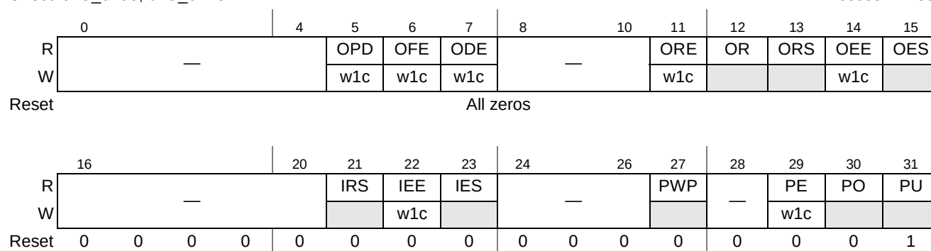
Figure 15-23. Port n Error and Status Command and Status Register (PnESCSR)
