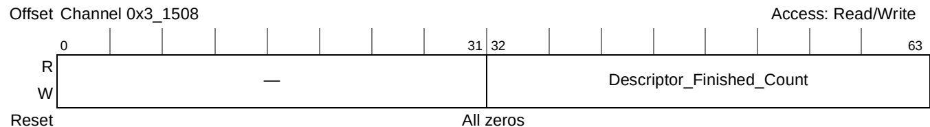
Figure 20-8. Descriptor Finished Counter
