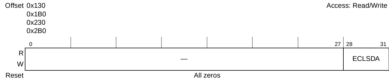
Figure 13-18. Extended Current List Descriptor Address Registers (ECLSDAR n )
