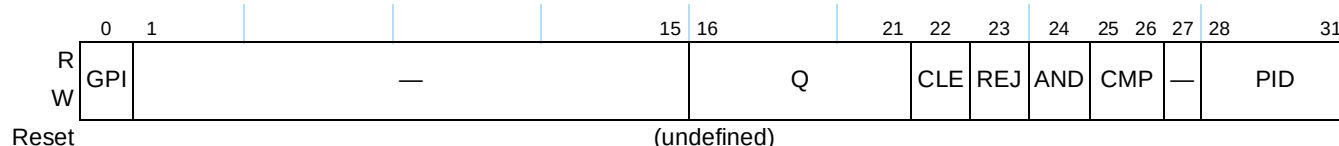
Figure 14-30. Receive Queue Filer Table Control Register Definition
