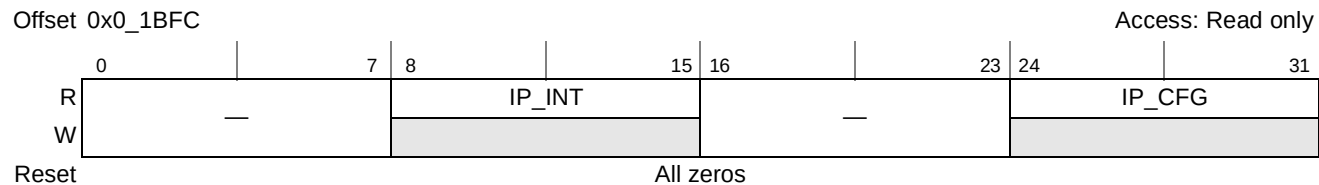
Figure 7-5. ECM IP Block Revision Register 2 (EIPBRR2)
