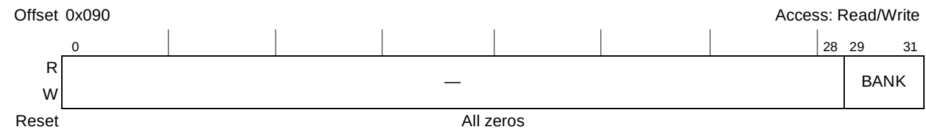
Figure 12-11. Special Operation Initiation Register (LSOR)
