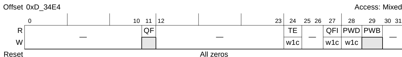
Figure 15-98. Inbound Port-Write Status Register (IPWSR)
