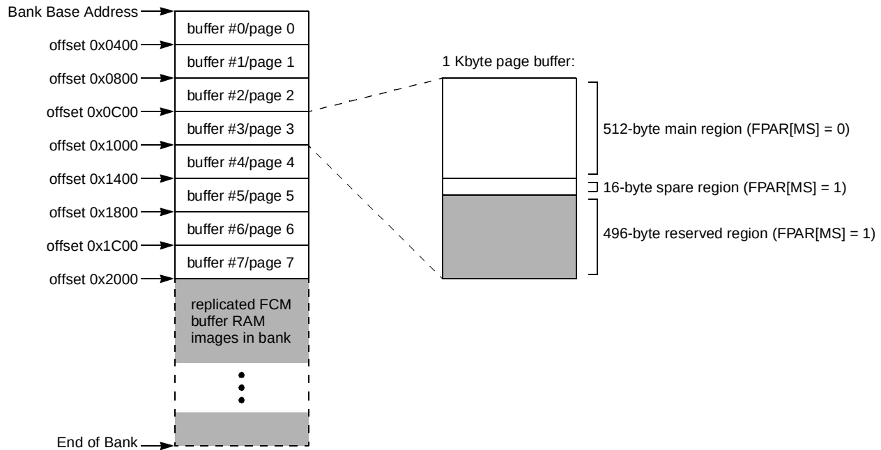
Figure 12-48. FCM Buffer RAM Memory Map for Small-Page (512-byte page) NAND Flash Devices
