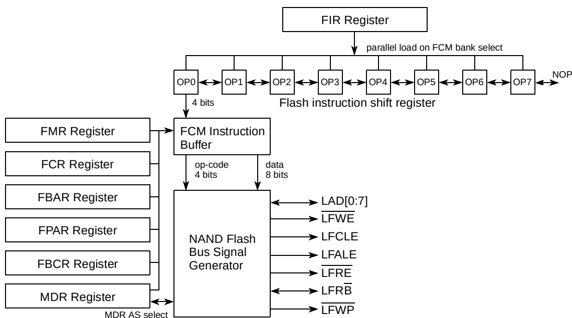
Figure 12-53. FCM Instruction Sequencer Mechanism
