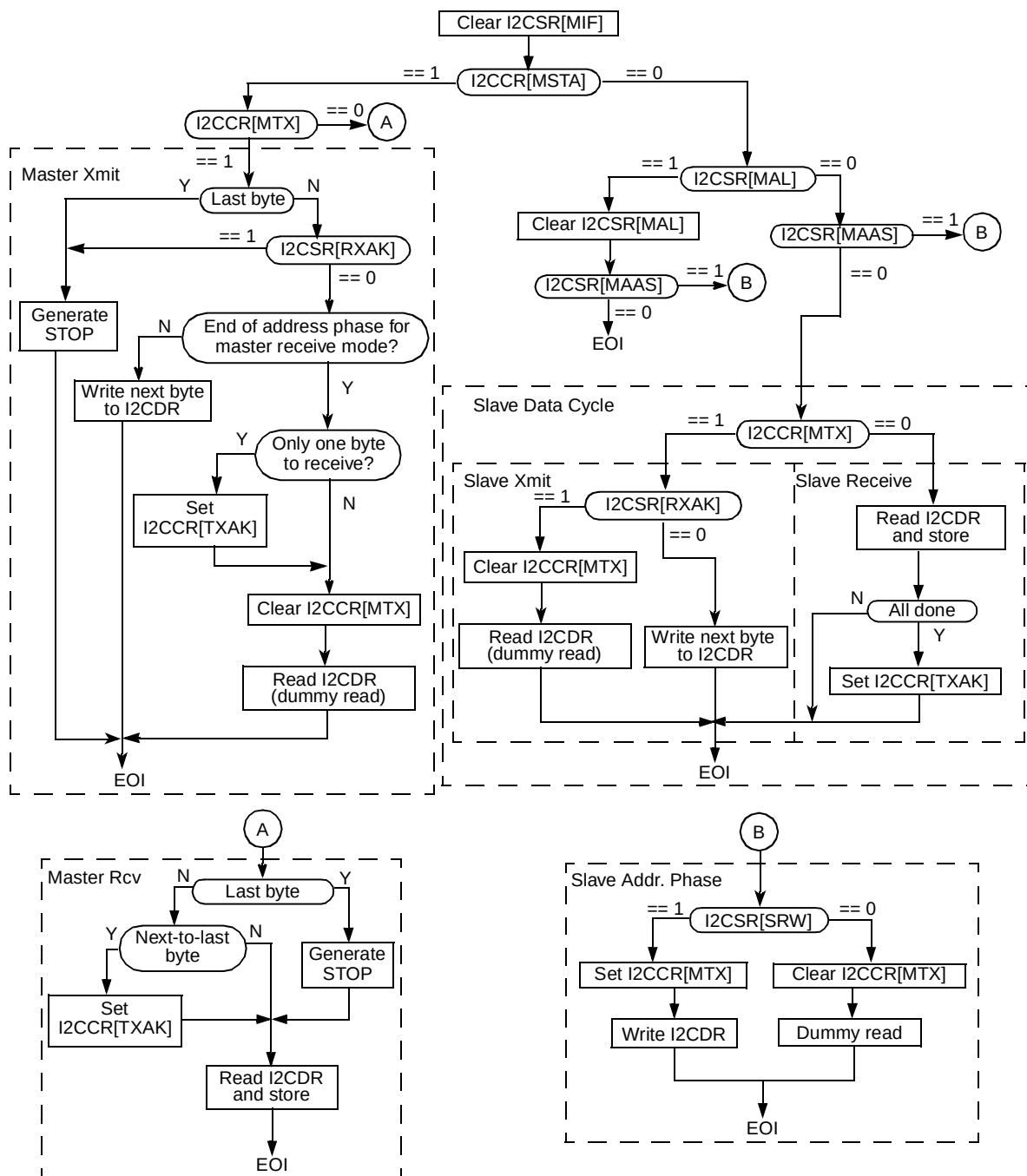
Figure 10-11. Example I 2 C Interrupt Service Routine Flowchart
