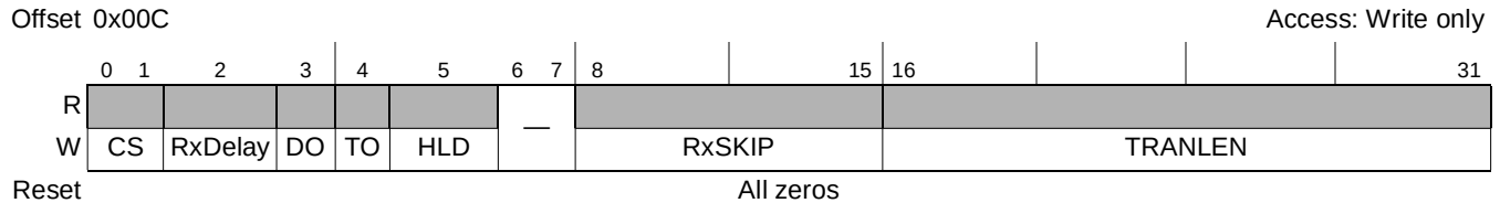
Figure 19-6. eSPI Command Register (SPCOM)
