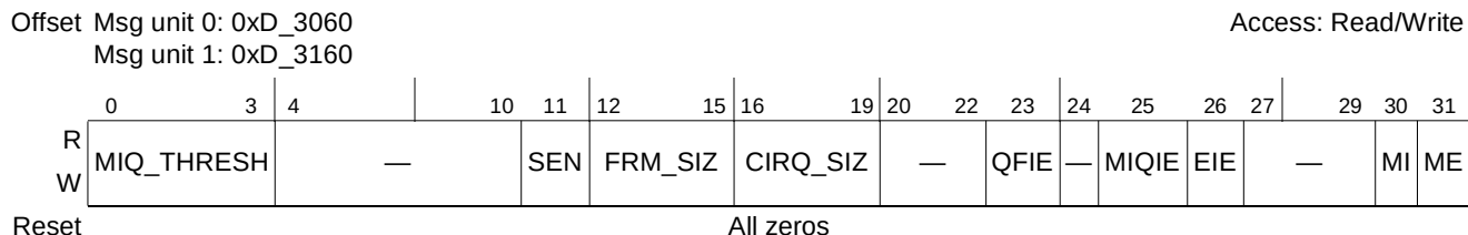
Figure 15-78. Inbound Message n Mode Registers (IM n MR)
