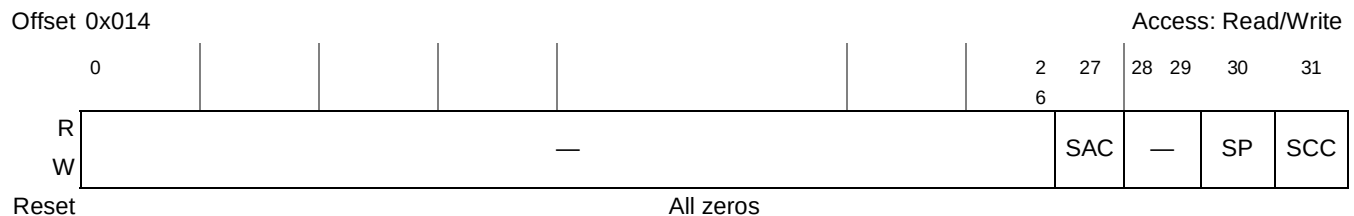
Figure 16-6. PCI Express Configuration Register (PEX_CONFIG)
