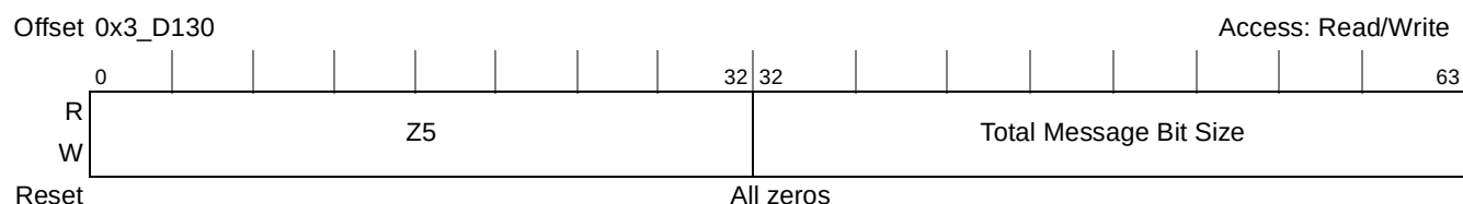
Figure 20-123. STEU Context_4 Register
