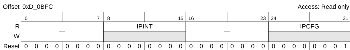
Figure 15-52. IP Block Revision Register 2 (IPBRR2)
