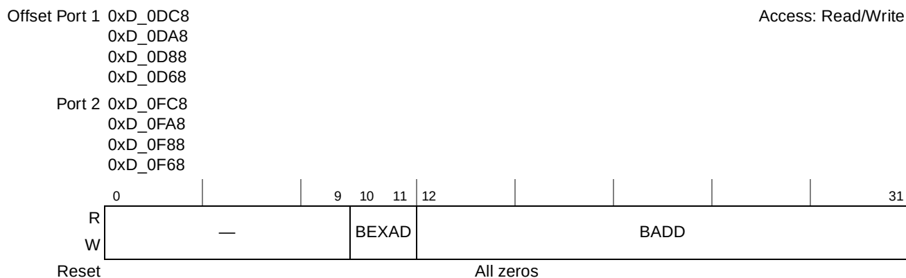
Figure 15-61. Port n RapidIO Inbound Window Base Address Registers1–4
