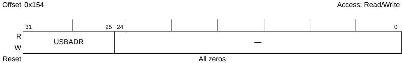
Figure 18-13. Device Address (DEVICEADDR)
