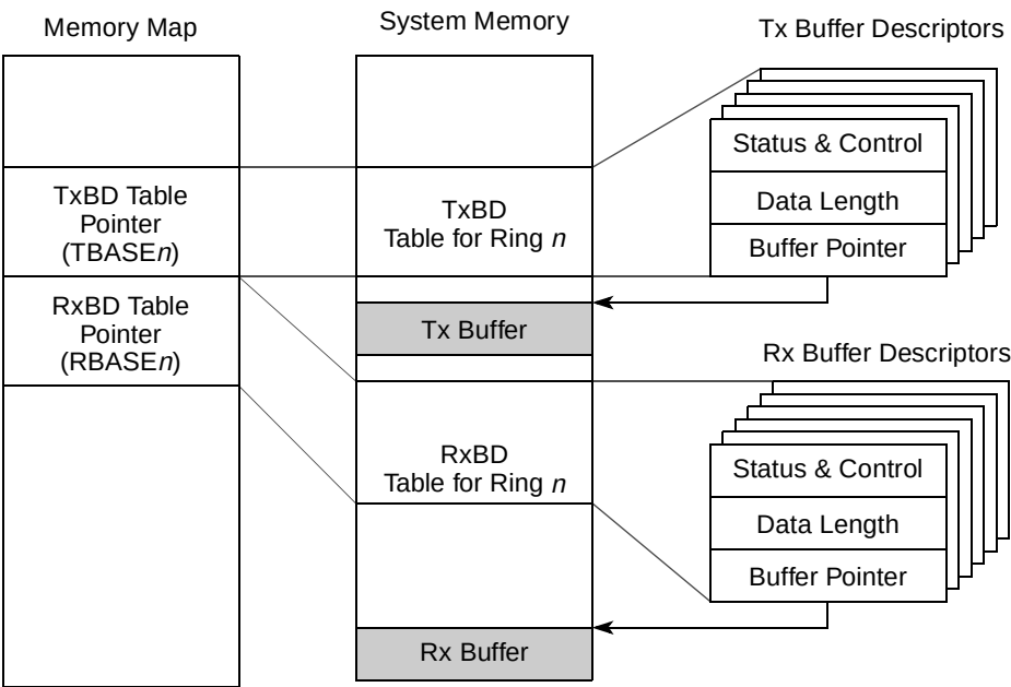
Figure 14-156. Example of eTSEC Memory Structure for BDs
