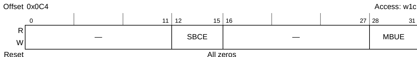
Figure 12-18. Transfer Error ECC Register (LTECCR)
