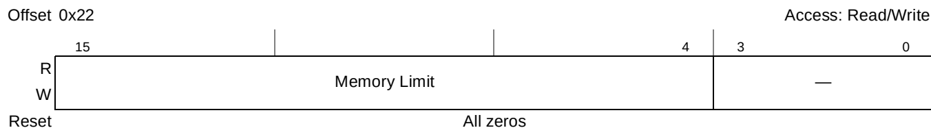
Figure 16-68. PCI Express Memory Limit Register
