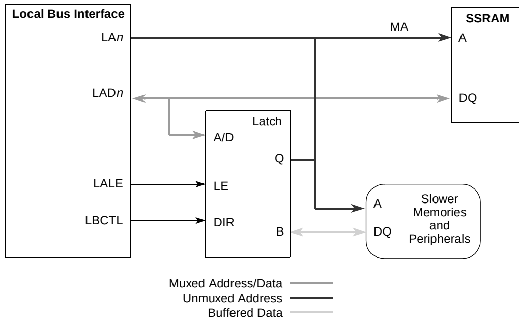
Figure 12-73. Local Bus Peripheral Hierarchy for High Bus Speeds
