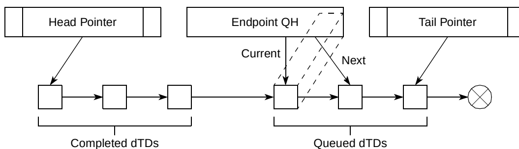
Figure 18-64. Software Link Pointers
