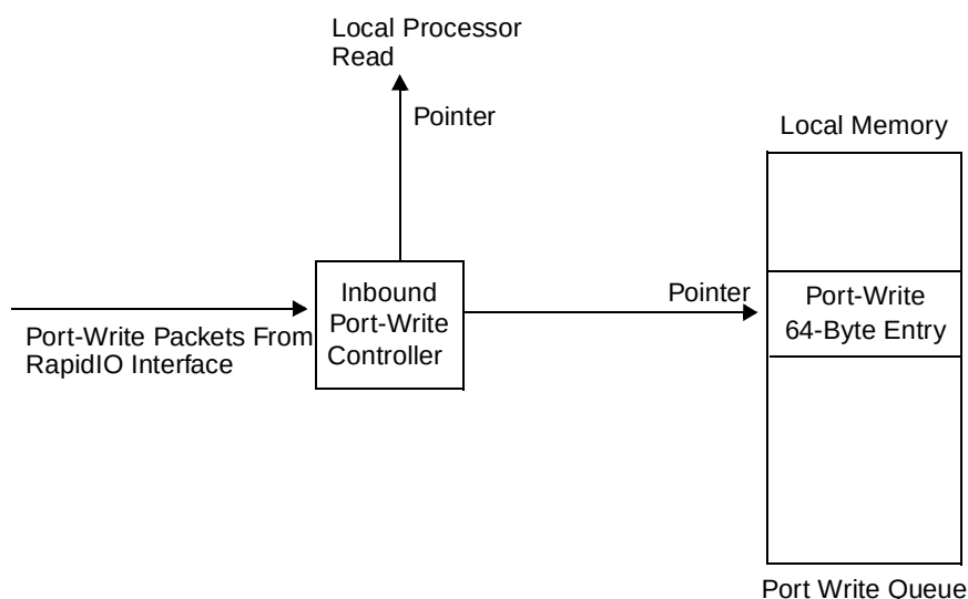
Figure 15-111. Inbound Port-Write Structure
