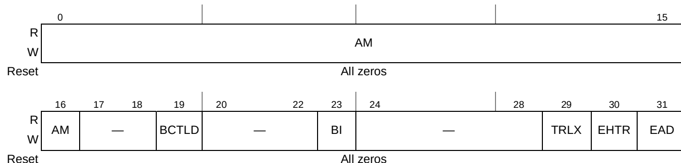
Figure 12-5. Option Registers (OR n ) in UPM Mode
