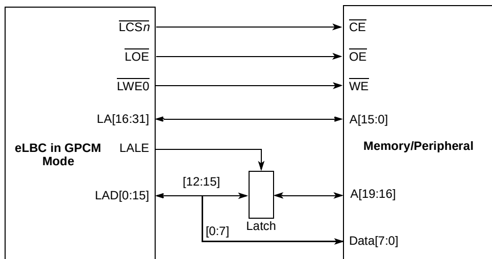
Figure 12-34. Enhanced Local Bus to GPCM Device Interface
