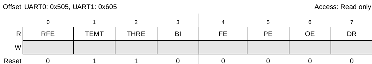
Figure 11-12. Line Status Register (ULSR)
