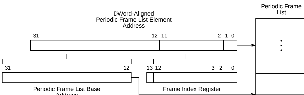
Figure 18-42. Derivation of Pointer into Frame List Array
