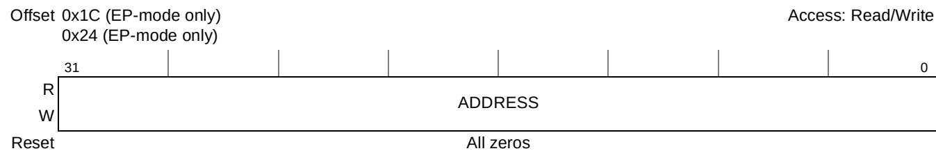
Figure 16-51. 64-Bit High Memory Base Address Register
