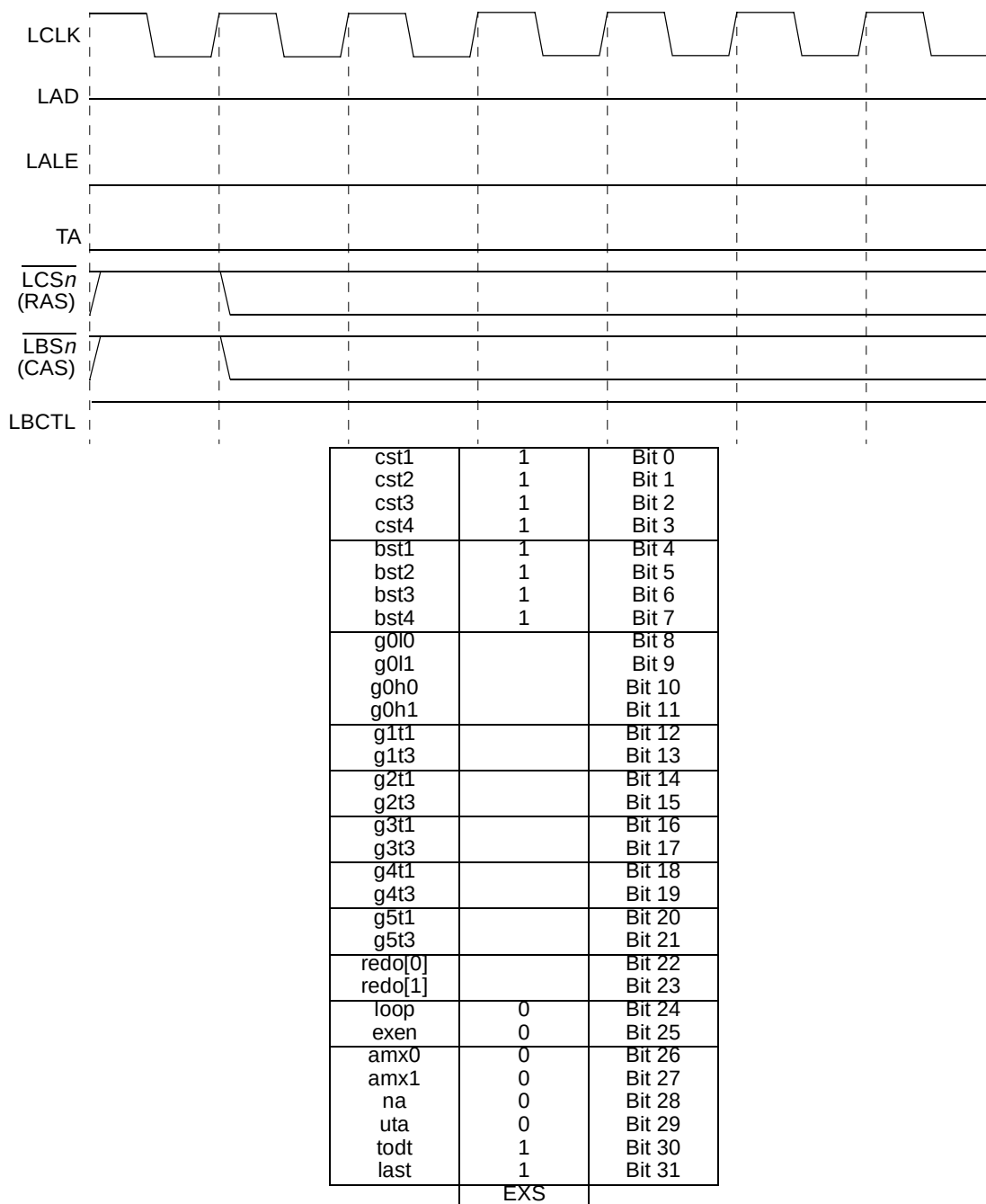
Figure 12-81. Exception Cycle
