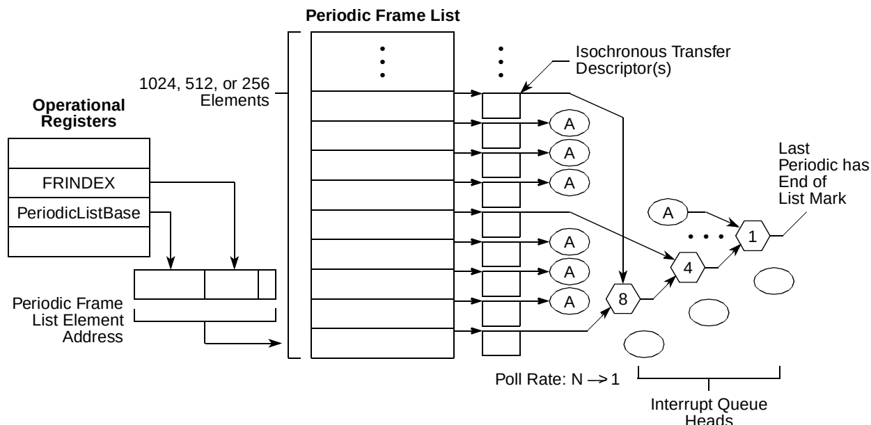
Figure 18-34. Periodic Schedule Organization
