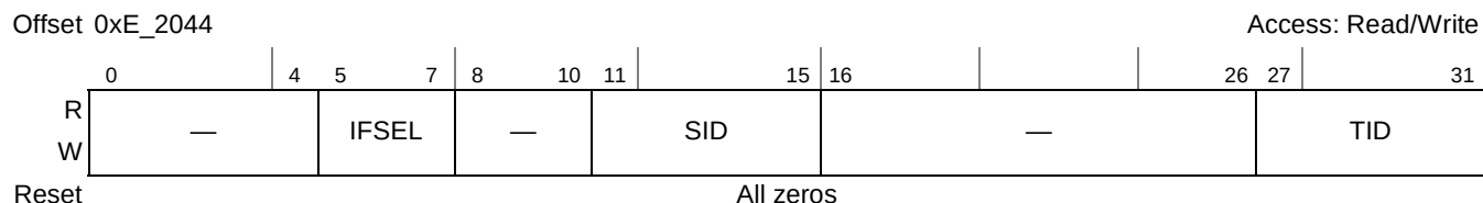
Figure 24-9. Trace Buffer Control Register 1 (TBCR1)
