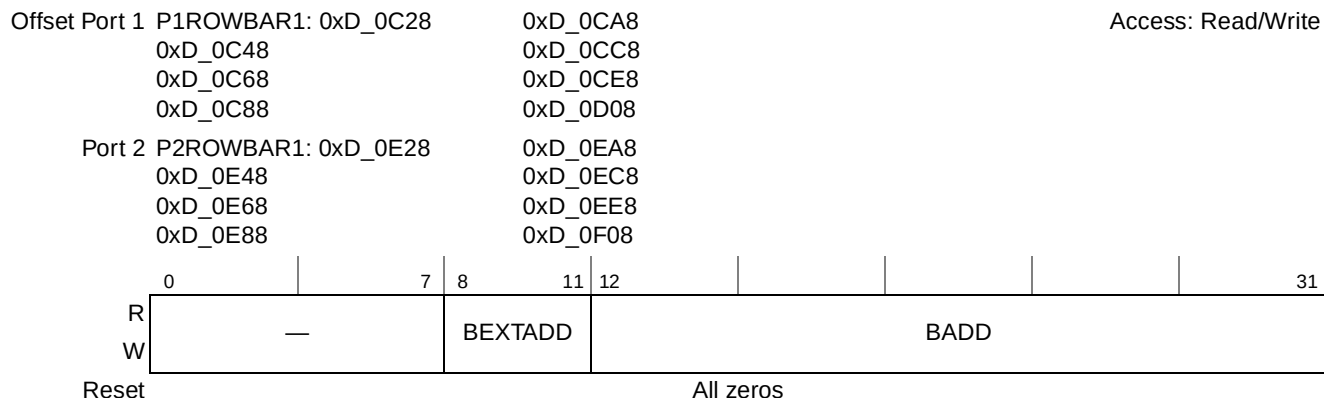
Figure 15-57. Port n RapidIO Outbound Window Base Address Registers 1–8
