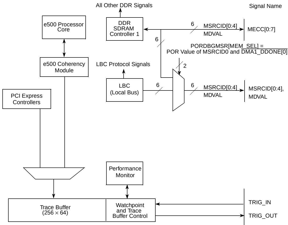
Figure 24-1. Debug and Watchpoint Monitor Block Diagram
