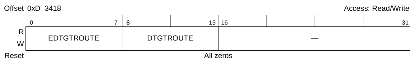
Figure 15-87. Outbound Doorbell Destination Port Registers (ODDPR)
