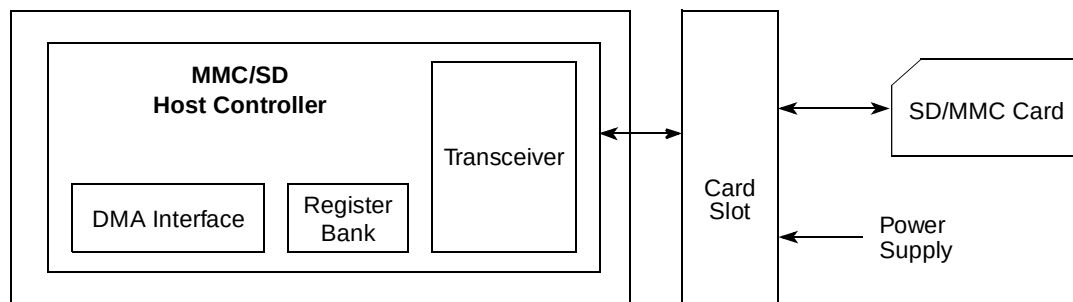
Figure 17-1. System Connection of the eSDHC
