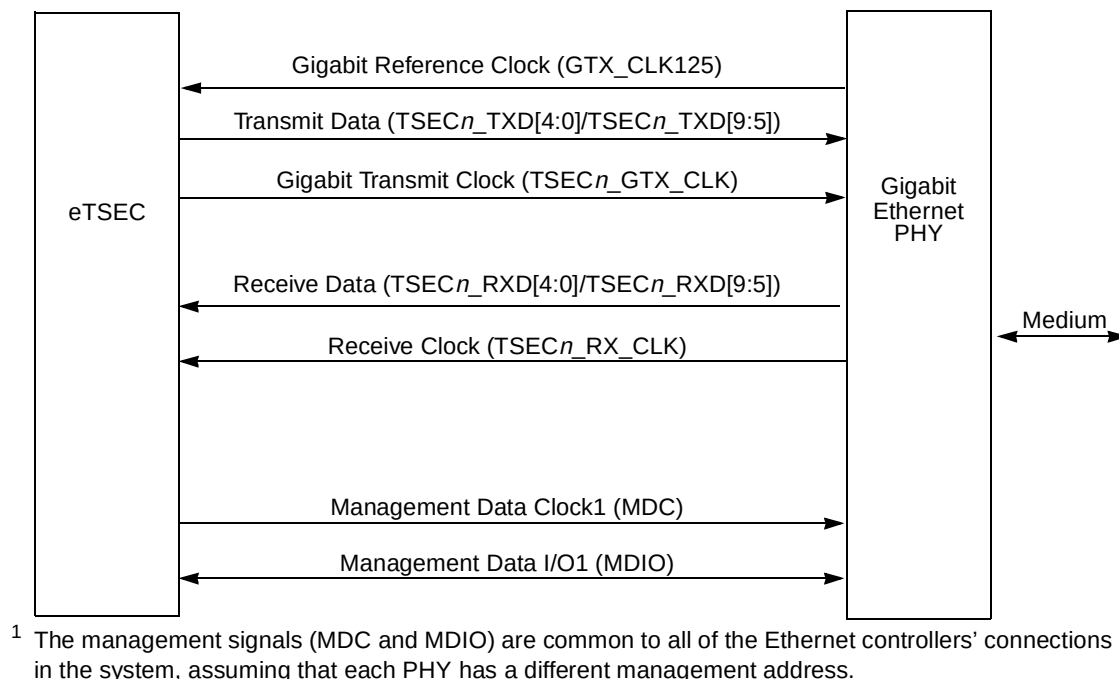
Figure 14-137. eTSEC-RTBI Connection
