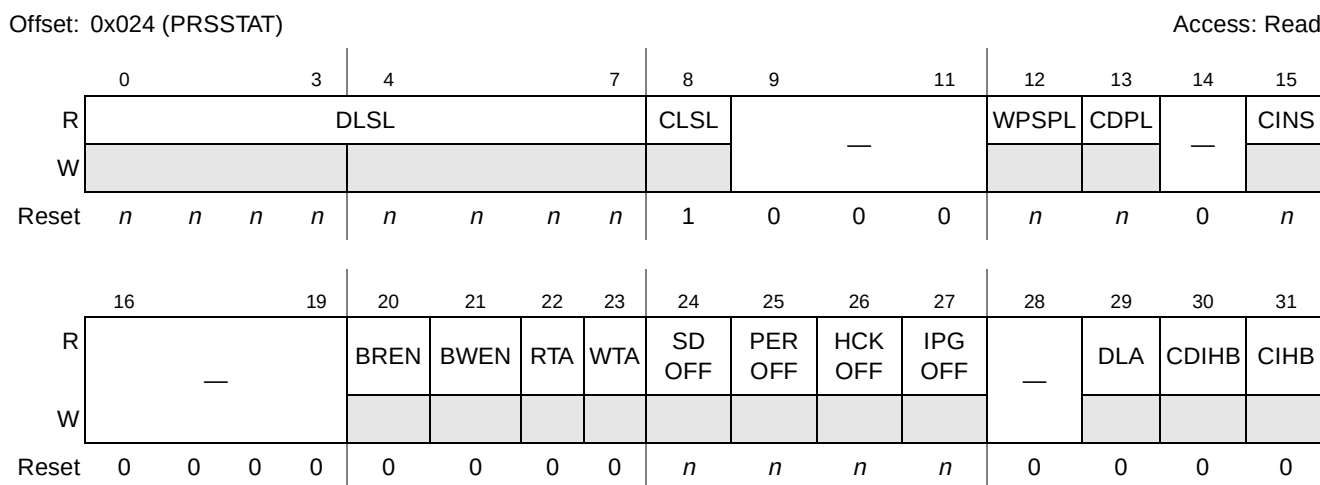
Figure 17-9. Present State Register (PRSSTAT)
