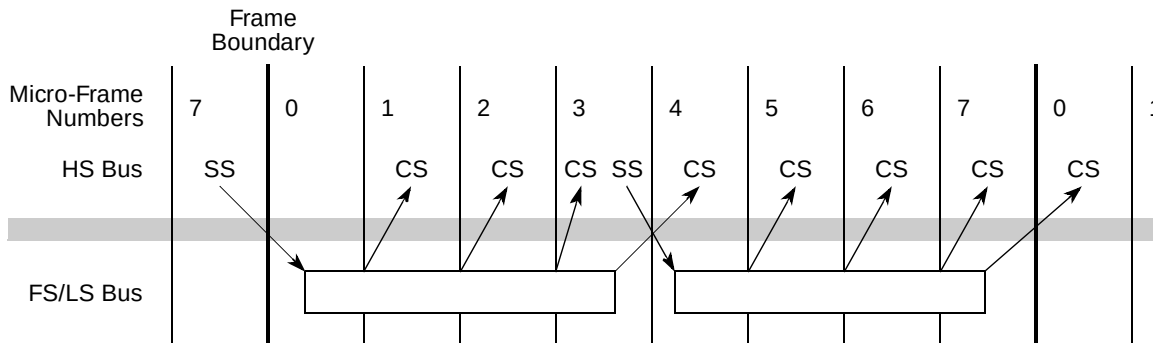
Figure 18-44. Frame Boundary Relationship Between HS Bus and FS/LS Bus
