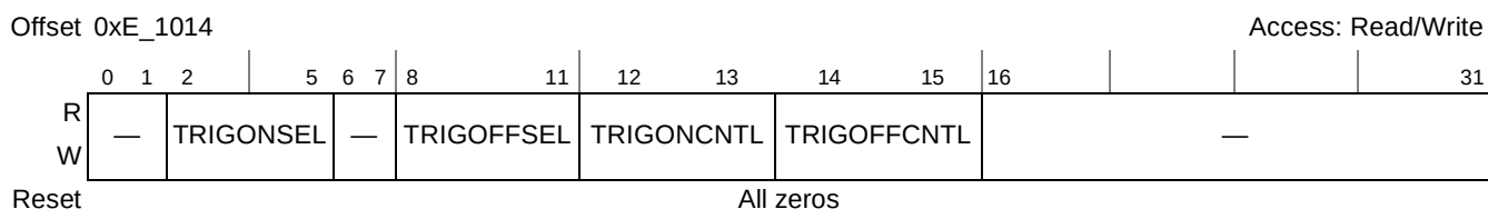
Figure 23-5. Performance Monitor Local Control Register B0 (PMLCB0)
