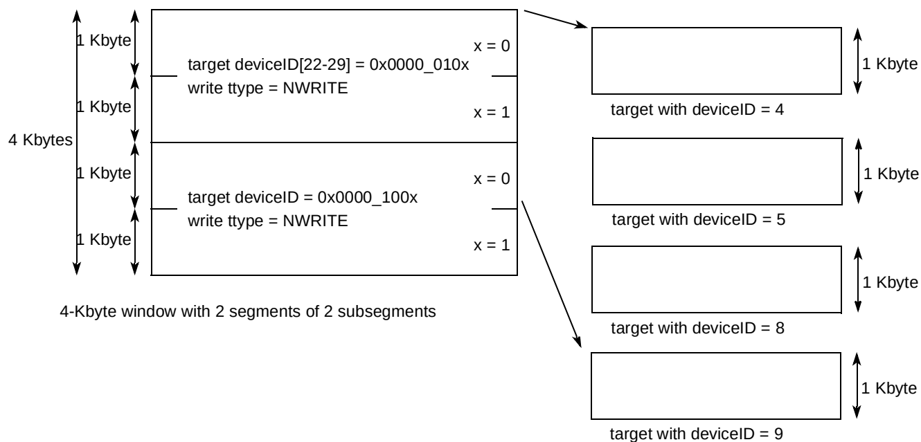
Figure 15-54. Example of Multi-Targeting
