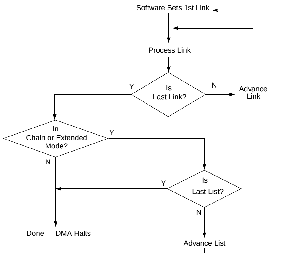
Figure 13-2. DMA Operational Flow Chart
