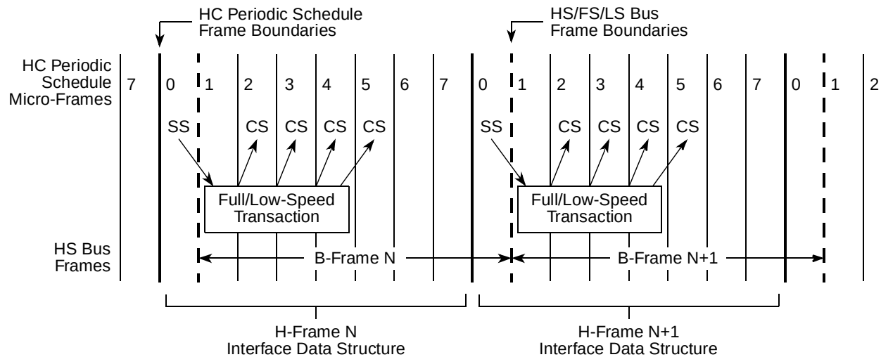
Figure 18-45. Relationship of Periodic Schedule Frame Boundaries to Bus Frame Boundaries
