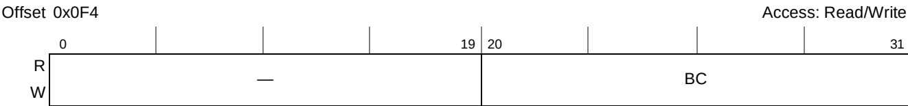
Figure 12-27. Flash Byte Count Register
