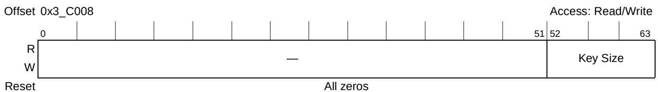
Figure 20-92. PKEU Key Size Register
