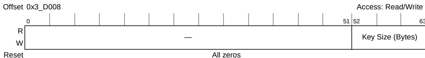
Figure 20-108. STEU Key Size Register
