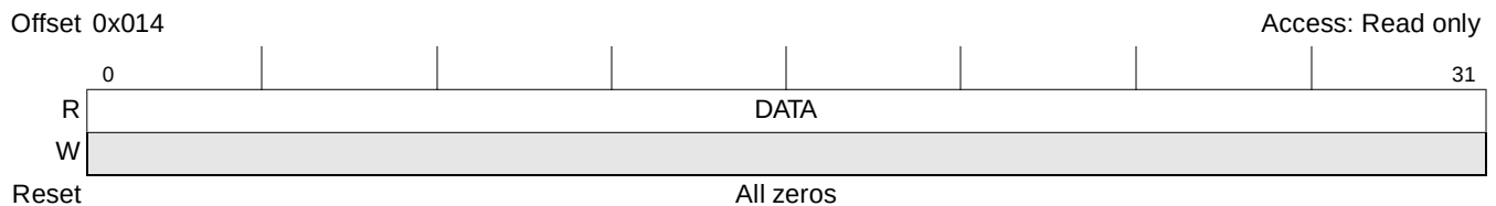
Figure 19-13. eSPI Receive Data Register (SPIRF)
