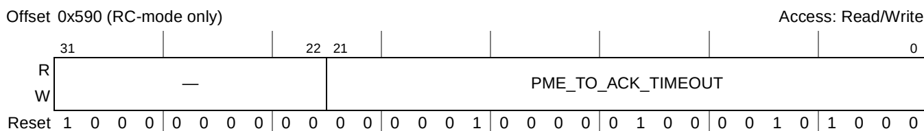
Figure 16-121. PCI Express PME_To_Ack Timeout Register (PEX_PME_TO_ACK_TOR)
