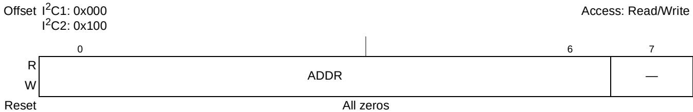
Figure 10-2. I 2 C Address Register (I2CADR)
