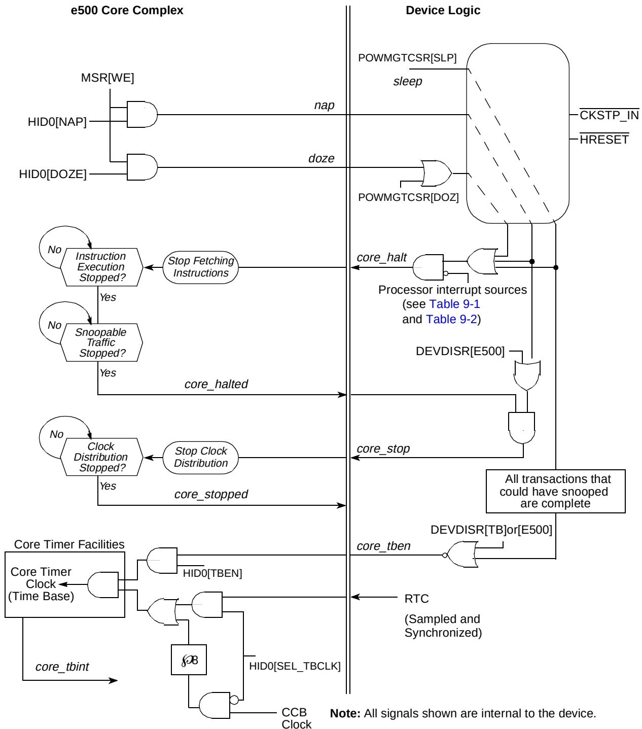
Figure 22-27. P2020 Power Management Handshaking Signals
