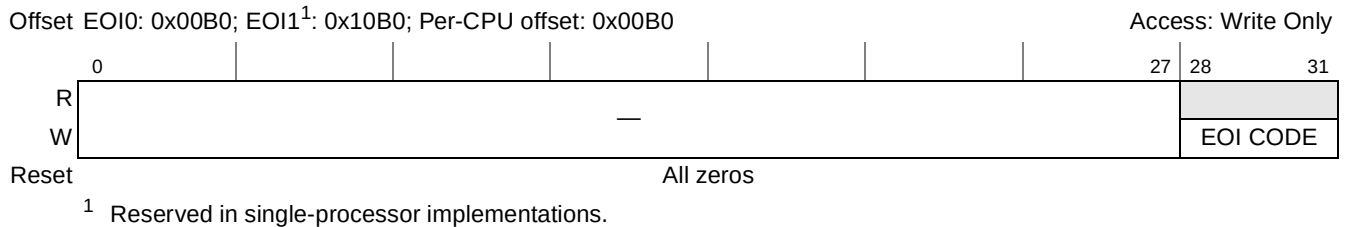
Figure 9-49. End of Interrupt Registers (EOI n )
