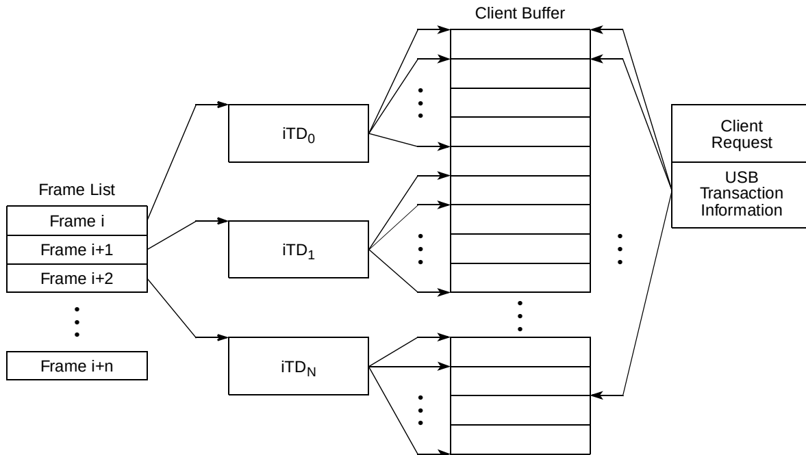
Figure 18-47. Example Association of iTDs to Client Request Buffer
