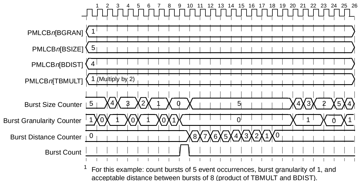
Figure 23-11. Burstiness Counting Timing Diagram
