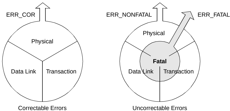
Figure 16-131. PCI Express Error Classification
