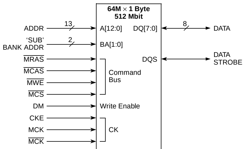
Figure 8-49. Typical DDR SDRAM Interface Signals
