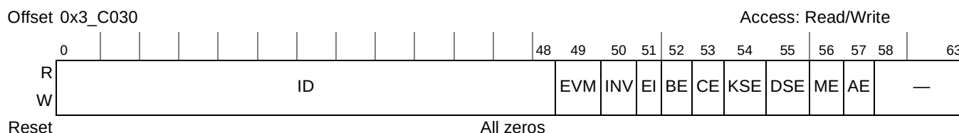
Figure 20-97. PKEU Interrupt Status Register
