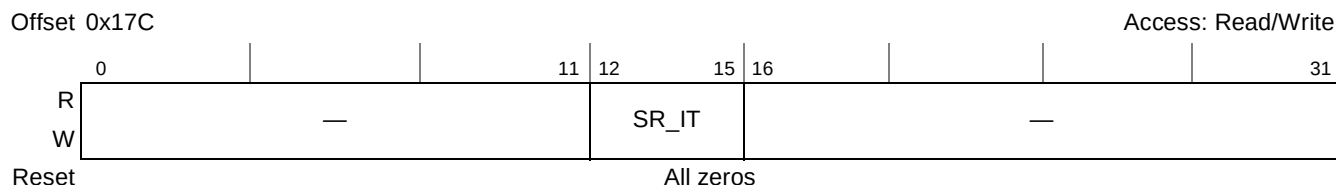
Figure 8-25. DDR Self Refresh Counter Register (DDR_SR_CNTR)
