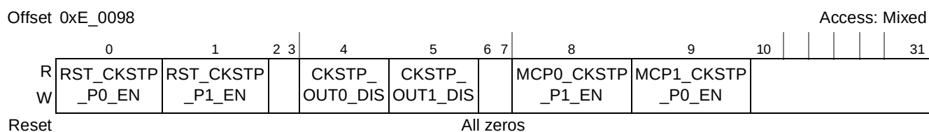
Figure 22-13. Exception Reset Control Register (ECTRSTCR)
