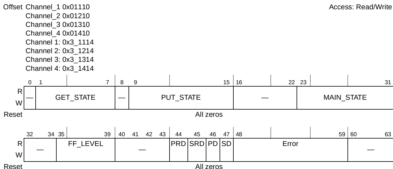
Figure 20-12. Channel Status Register (CSR)
