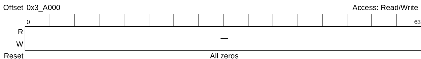
Figure 20-100. RNGU Mode Register
