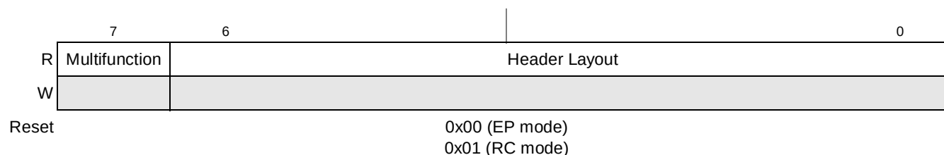
Figure 16-46. PCI Express Bus Latency Timer Register
