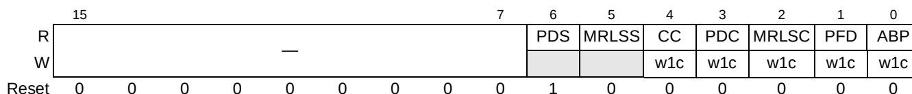
Figure 16-94. PCI Express Slot Status Register
