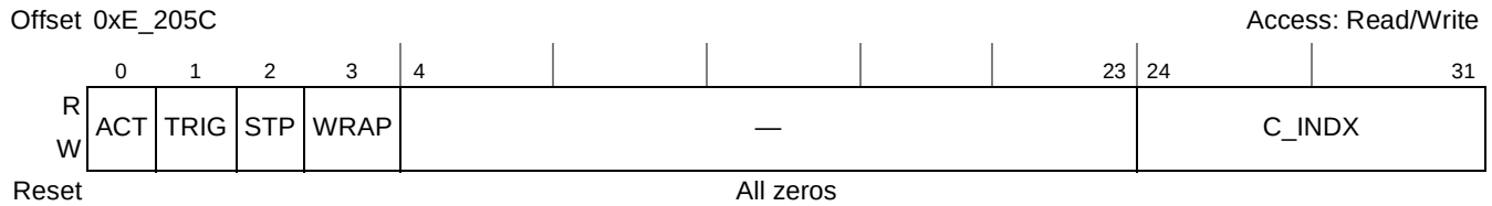
Figure 24-13. Trace Buffer Status Register (TBSR)
