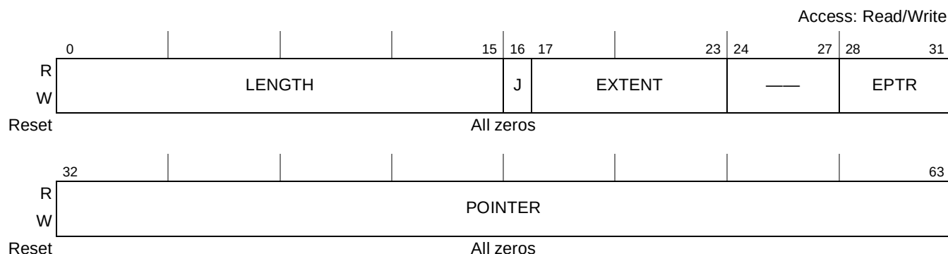
Figure 20-4. Pointer Dword
