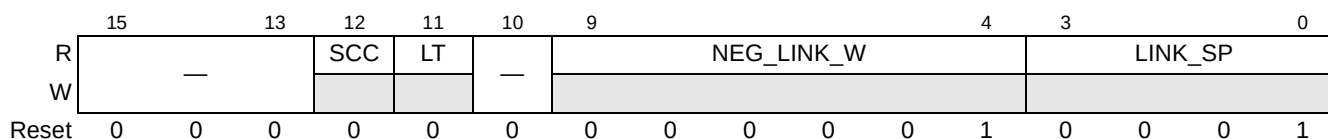
Figure 16-91. PCI Express Link Status Register
