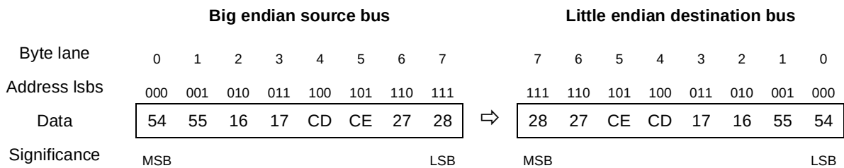
Figure 16-128. Address Invariant Byte Ordering—8 bytes Outbound
