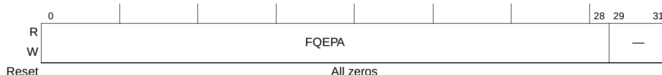
Figure 15-83. Inbound Message n Frame Queue Enqueue Pointer Address Registers (IM n FQEPAR)
