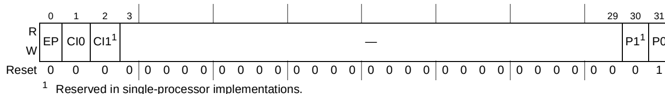
Figure 9-39. External Interrupt Destination Registers (EIDRs)
