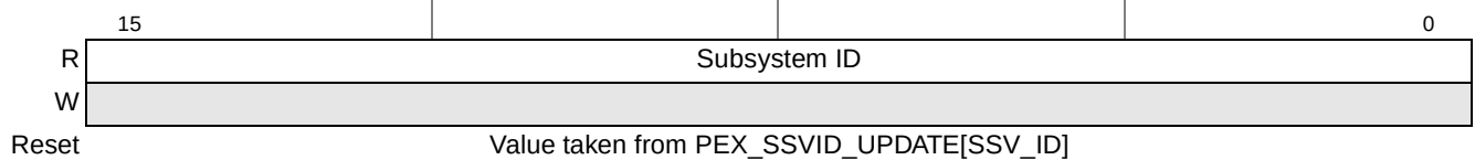
Figure 16-53. PCI Express Subsystem ID Register
