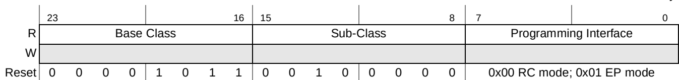
Figure 16-43. PCI Express Class Code Register
