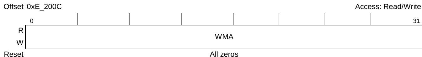
Figure 24-4. Watchpoint Monitor Address Register (WMAR)
