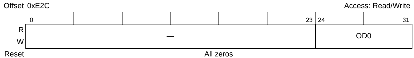
Figure 16-31. PCI Express Error Capture Register 1 (PEX_ERR_CAP_R1) Internal Source, Outbound Transaction
