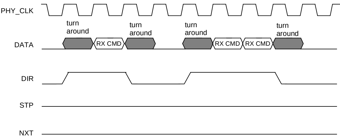
Figure 18-66. Sending of RX CMD
