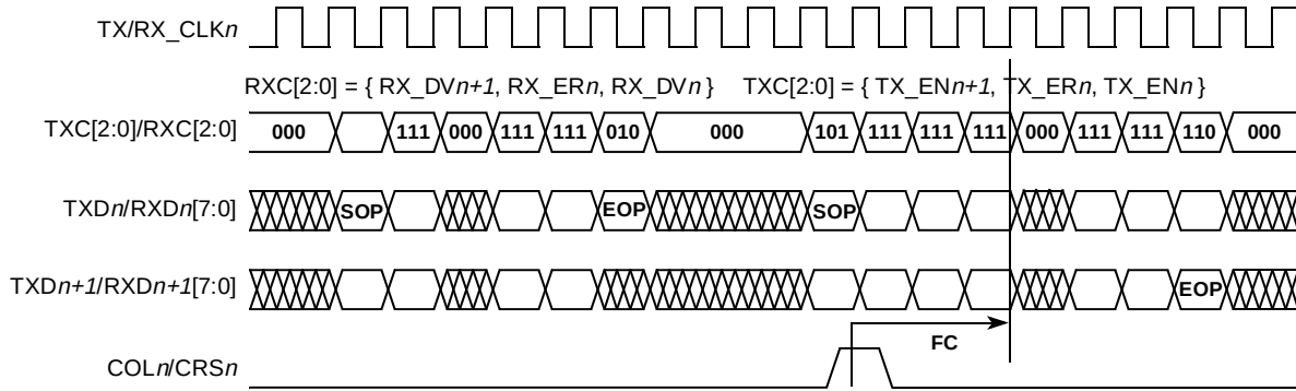
Figure 14-142. 16-Bit Encoded Packet FIFO Timing
