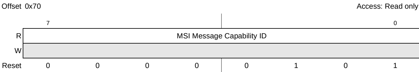
Figure 16-97. PCI Express Capability ID Register
