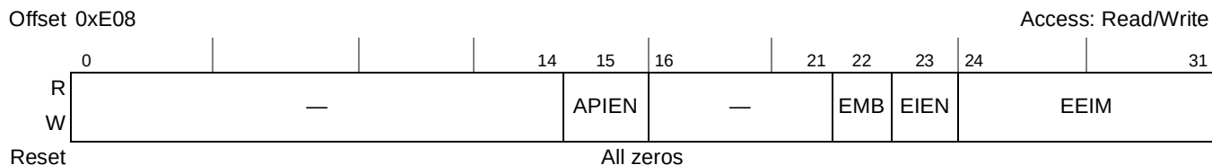
Figure 8-36. Memory Data Path Error Injection Mask ECC Register (ERR_INJECT)
