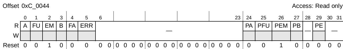
Figure 15-10. Port-Write and Doorbell Command and Status Register (PWDCSR)
