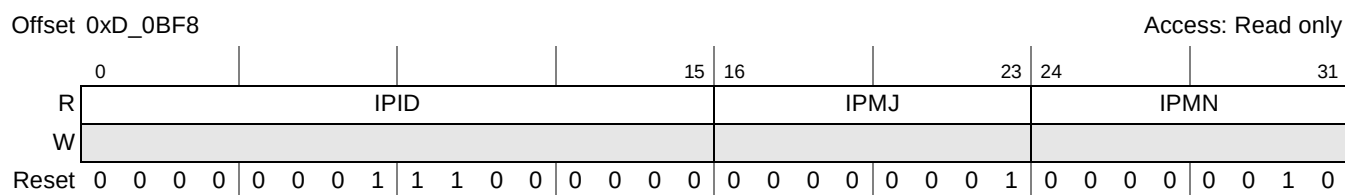
Figure 15-51. IP Block Revision Register 1 (IPBRR1)
