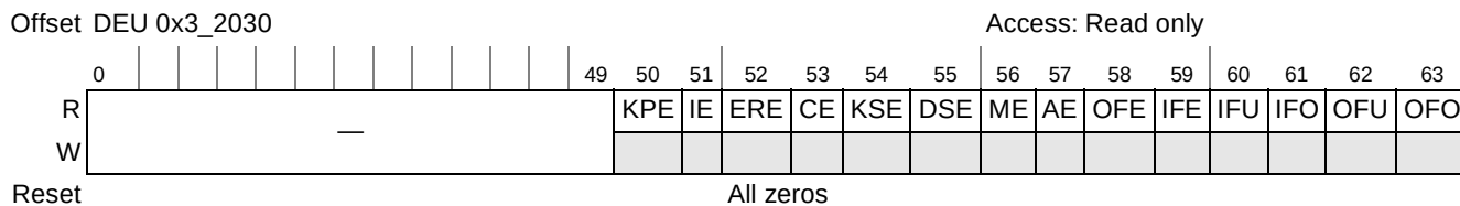
Figure 20-61. DEU Interrupt Status Register
