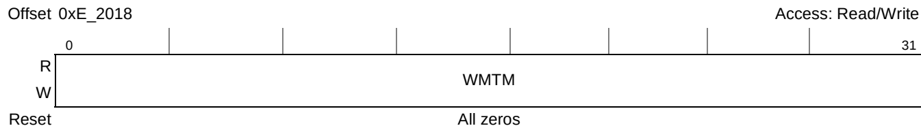
Figure 24-6. Watchpoint Monitor Transaction Mask Register (WMTMR)
