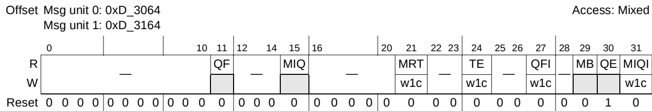
Figure 15-79. Inbound Message n Status Registers (IM n SR)
