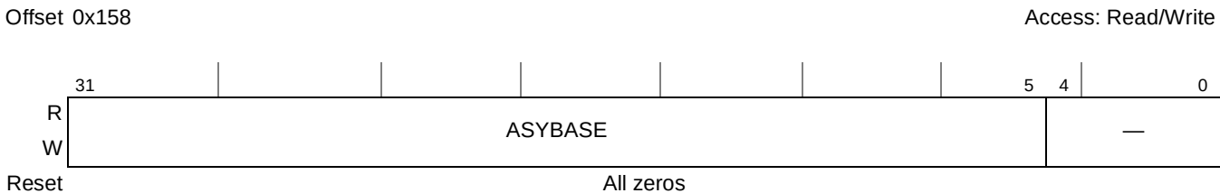
Figure 18-14. Current Asynchronous List Address (ASYNCLISTADDR)
