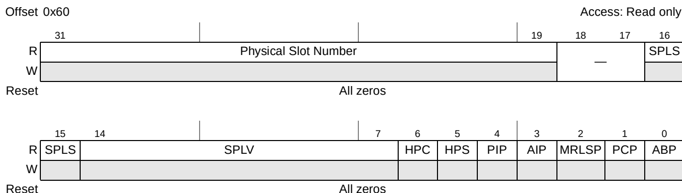
Figure 16-92. PCI Express Slot Capabilities Register
