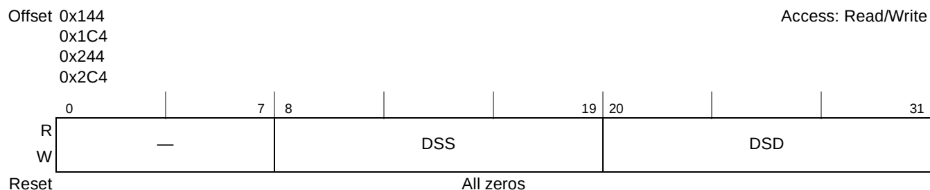
Figure 13-23. Destination Stride Registers (DSR n )
