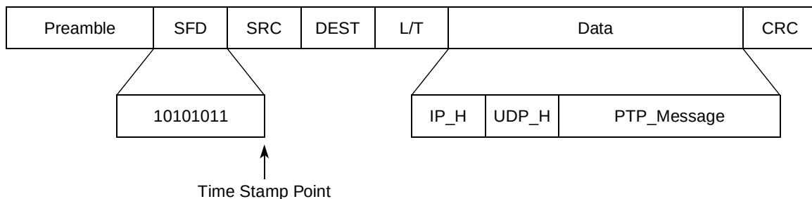
Figure 14-153. PTP Packet Format
