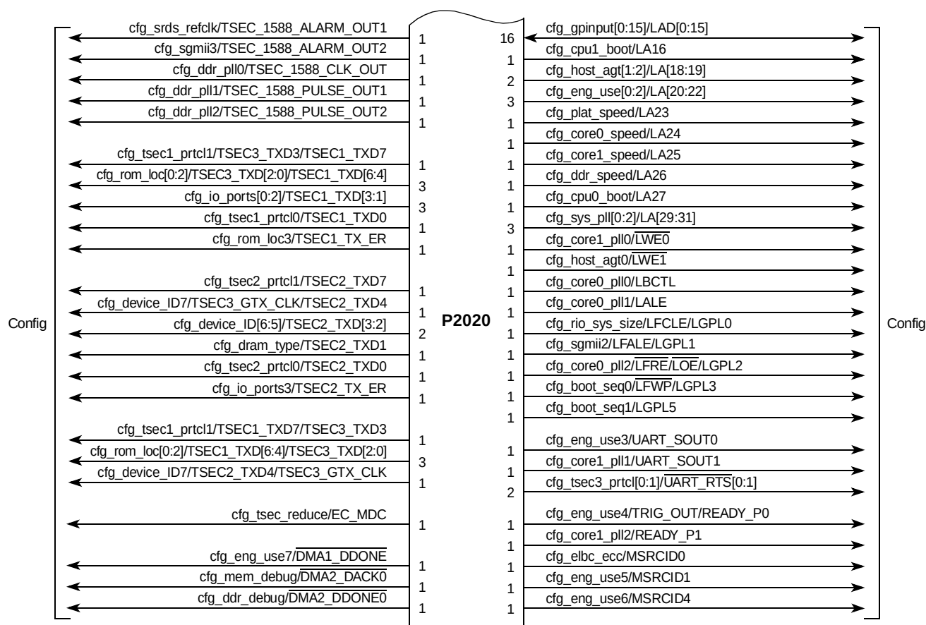
Figure 3-3. P2020 Signal Groupings (3/3) (Continued)
