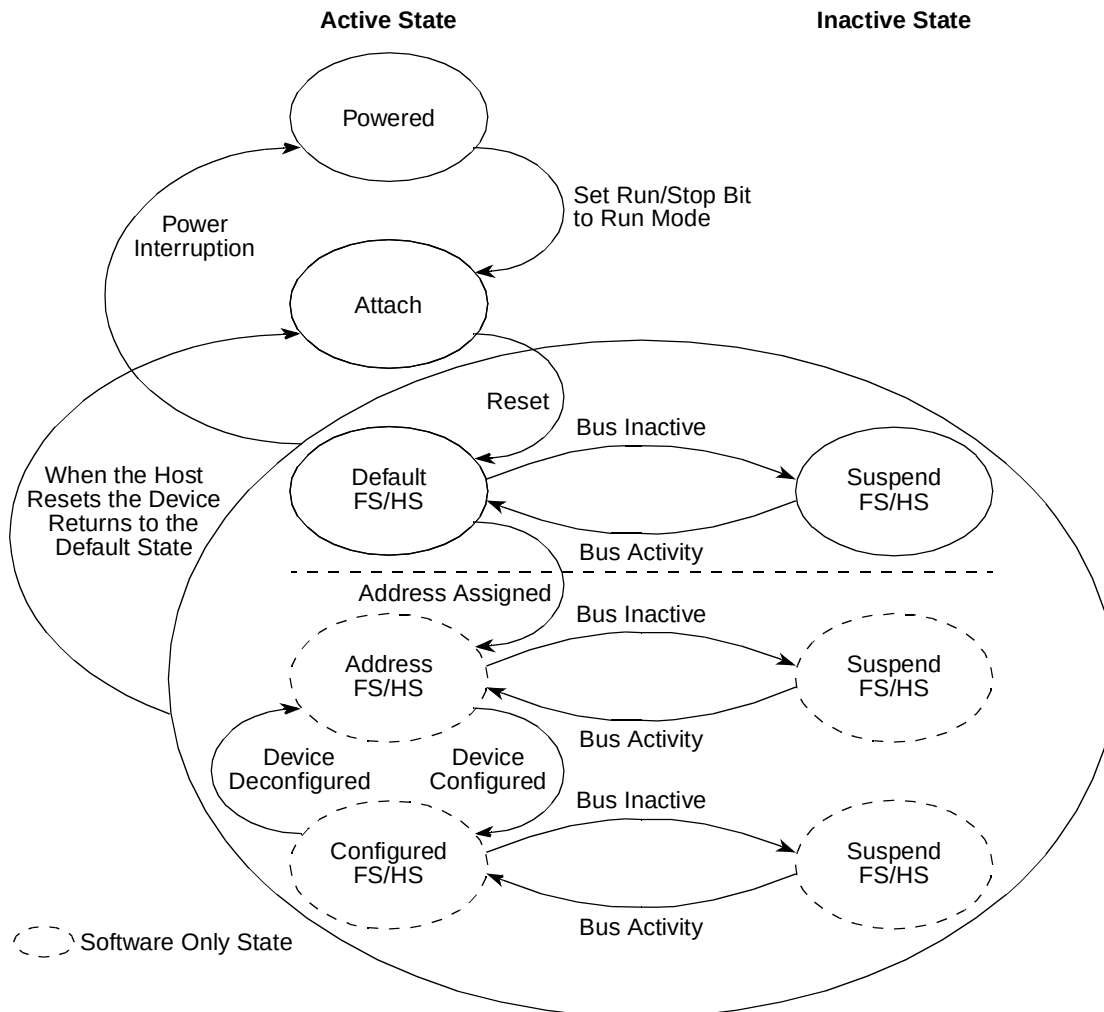
Figure 18-62. USB 2.0 Device States
