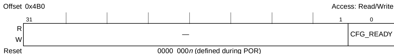
Figure 16-120. PCI Express Configuration Ready Register (PEX_CFG_READY)
