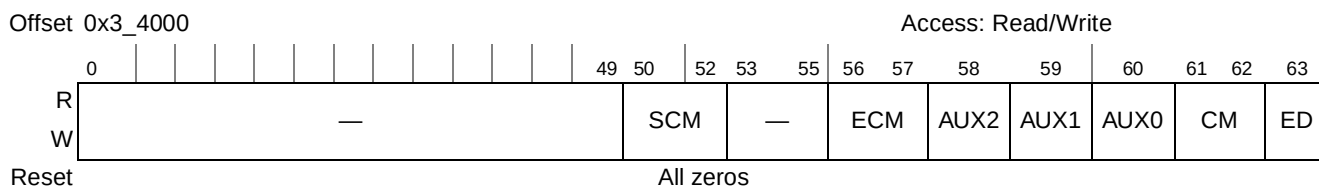
Figure 20-21. AESU Mode Register
