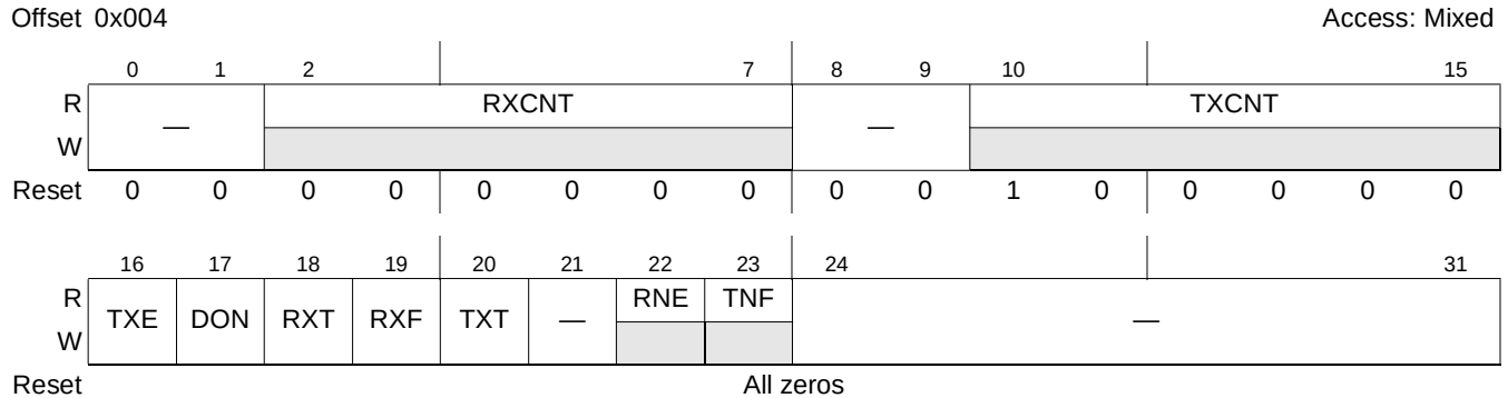
Figure 19-4. eSPI Event Register (SPIE)
