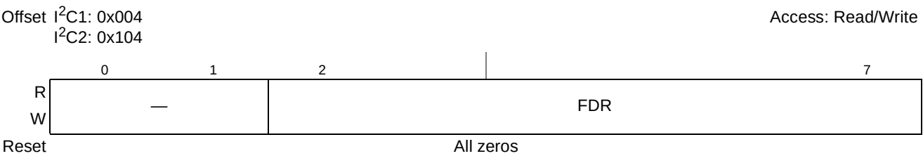
Figure 10-3. I 2 C Frequency Divider Register (I2CFDR)
