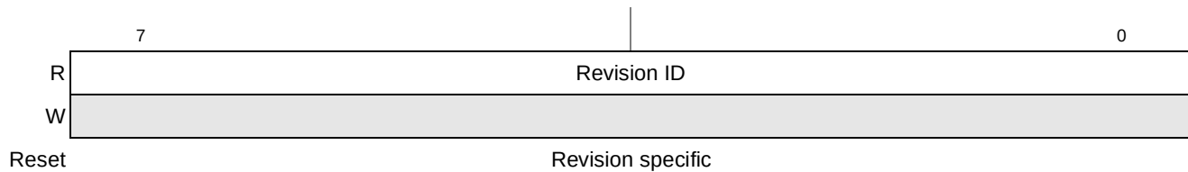
Figure 16-42. PCI Express Revision ID Register
