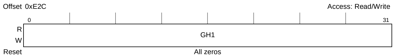
Figure 16-32. PCI Express Error Capture Register 1 (PEX_ERR_CAP_R1) External Source, Inbound Transaction
