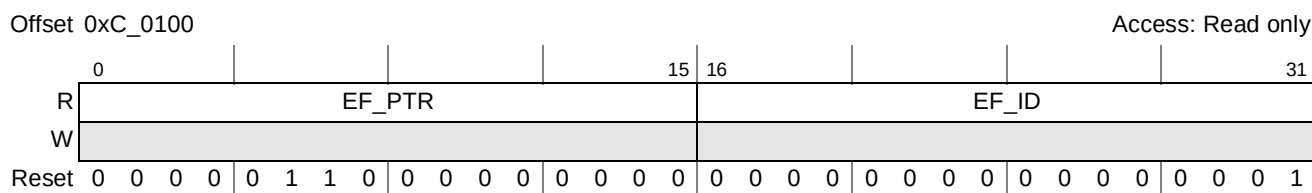
Figure 15-16. Port Maintenance Block Header 0 (PMBH0)
