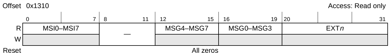
Figure 9-19. IRQ_OUT Summary Register 0 (IRQSR0)
