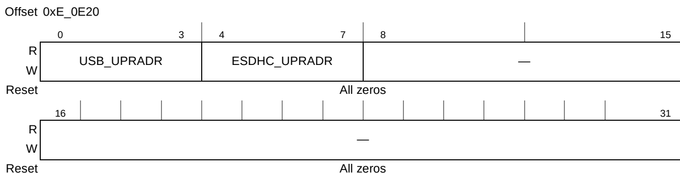
Figure 22-21. ECM Control Register (ECMCR)
