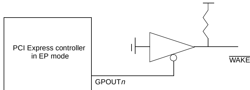
Figure 16-133. \overline{\text{WAKE}} Generation Example
