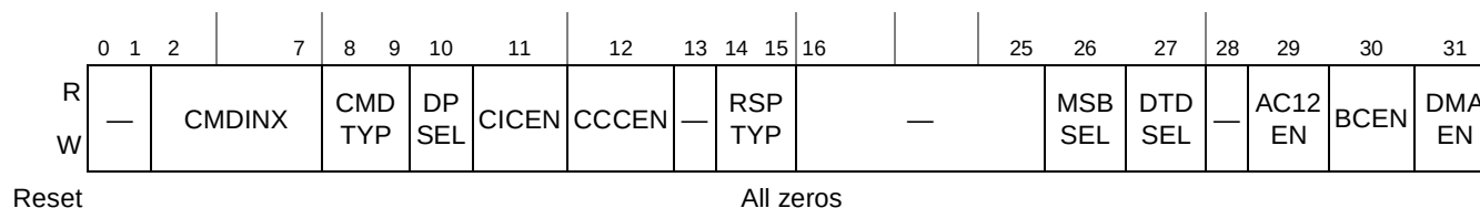
Figure 17-6. Transfer Type Register (XFERTYP)
