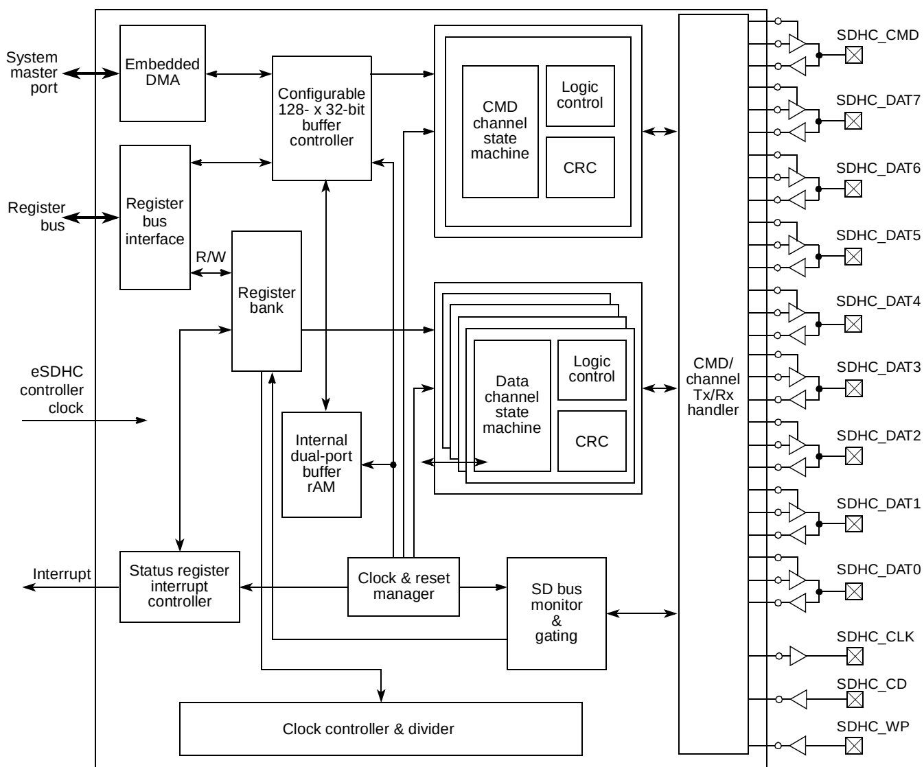
Figure 17-2. eSDHC Block Diagram
