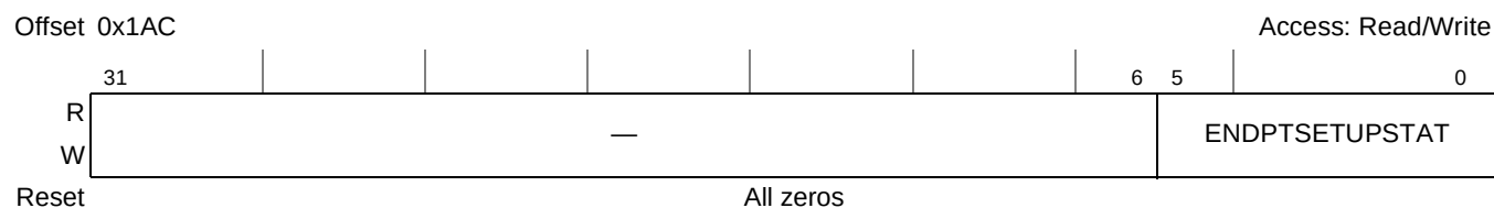
Figure 18-22. Endpoint Setup Status (ENDPTSETUPSTAT)
