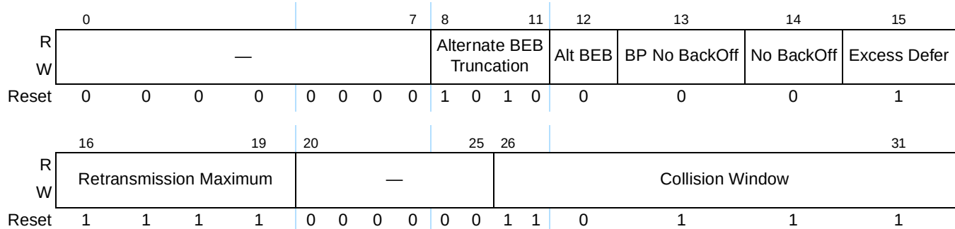
Figure 14-42. Half-Duplex Register Definition
