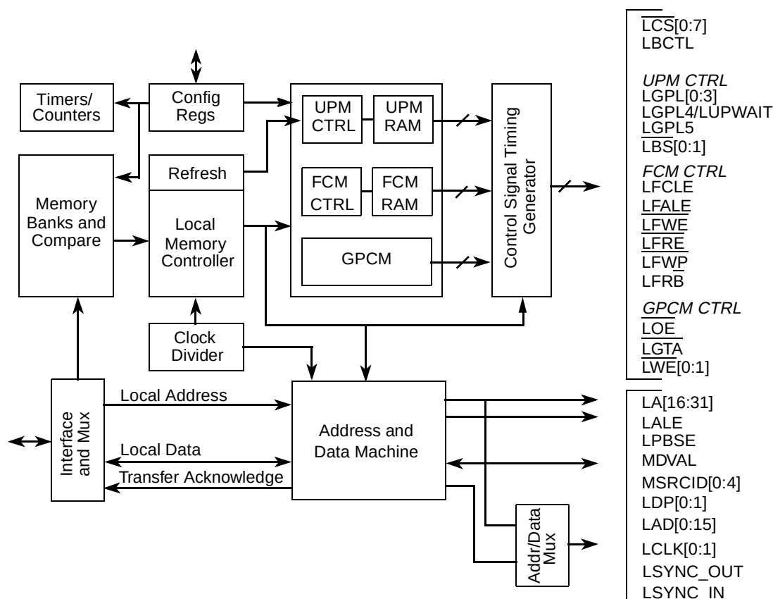
Figure 12-1. Enhanced Local Bus Controller Block Diagram
