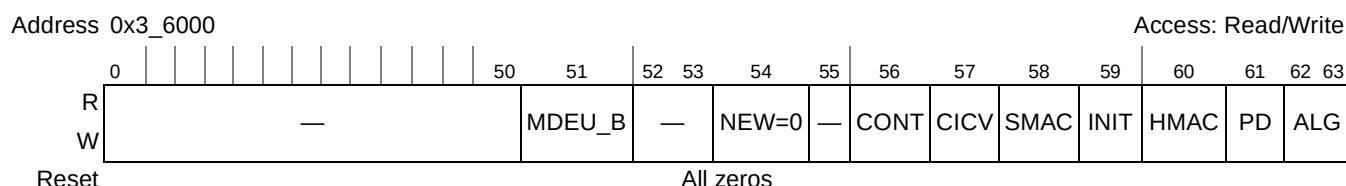
Figure 20-79. MDEU Mode Register in Old Configuration
