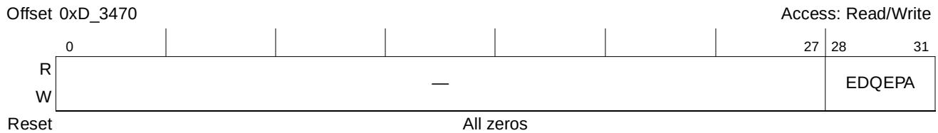
Figure 15-94. Extended Inbound Doorbell Queue Enqueue Pointer Address Register (EIDQEPAR)
