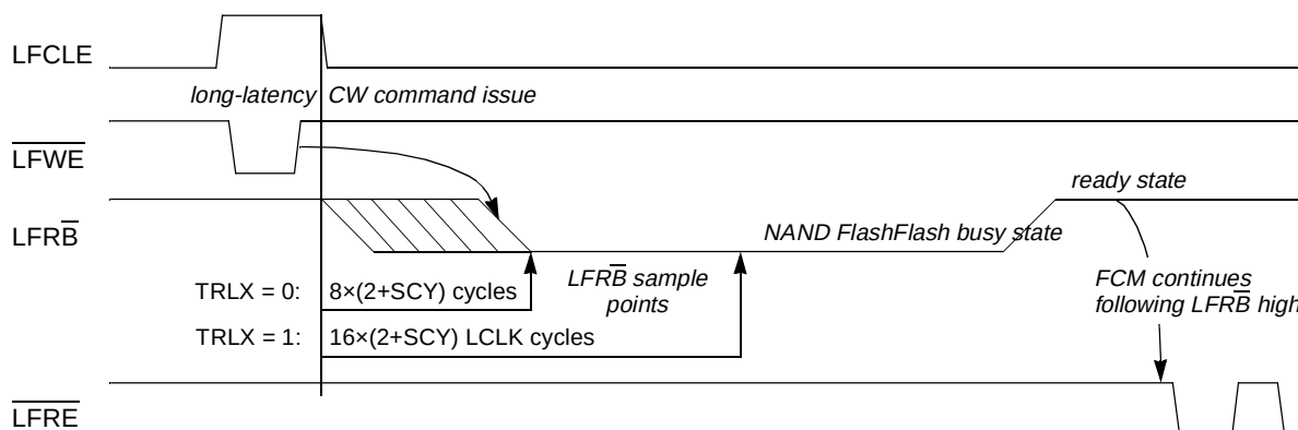
Figure 12-57. FCM Delay Prior to Sampling LFR\bar{B} State
