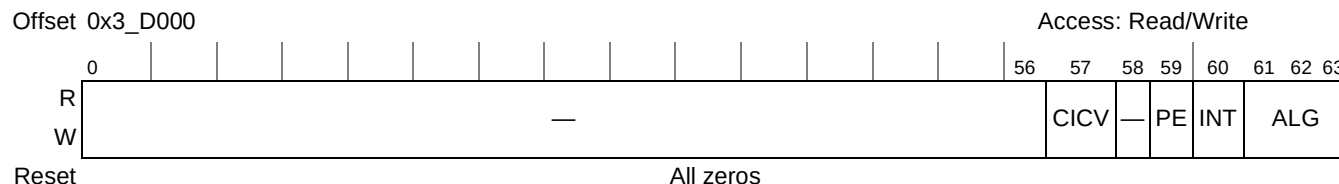
Figure 20-107. STEU Mode Register
