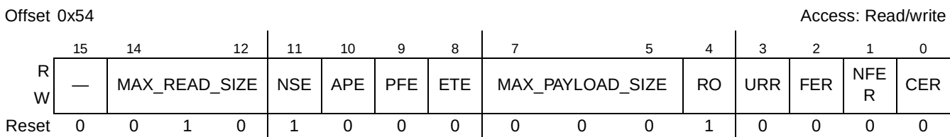
Figure 16-87. PCI Express Device Control Register
