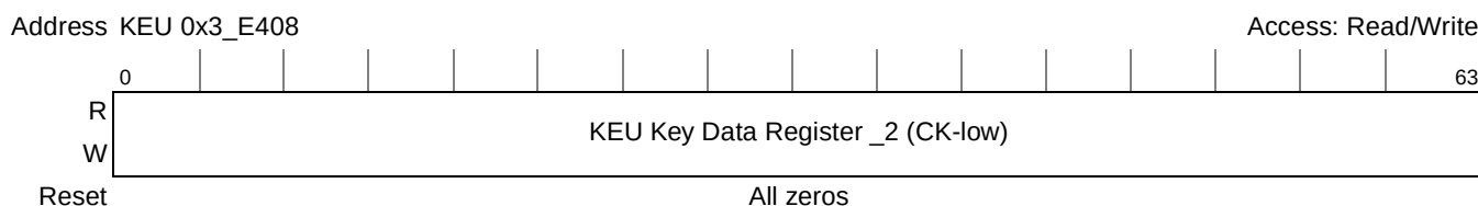
Figure 20-76. KEU Key Data Register _2 (CK-Low)
