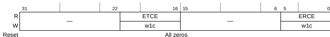
Figure 18-26. Endpoint Complete (ENDPTCOMPLETE)
