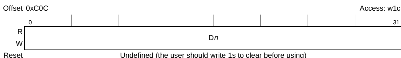
Figure 21-5. GPIO Interrupt Event Register (GPIER)
