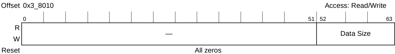
Figure 20-34. AFEU Context/Data Size Register
