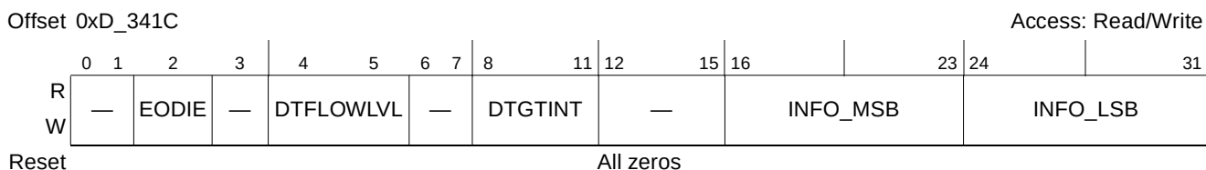
Figure 15-88. Outbound Doorbell Destination Attributes Register (ODDATR)
