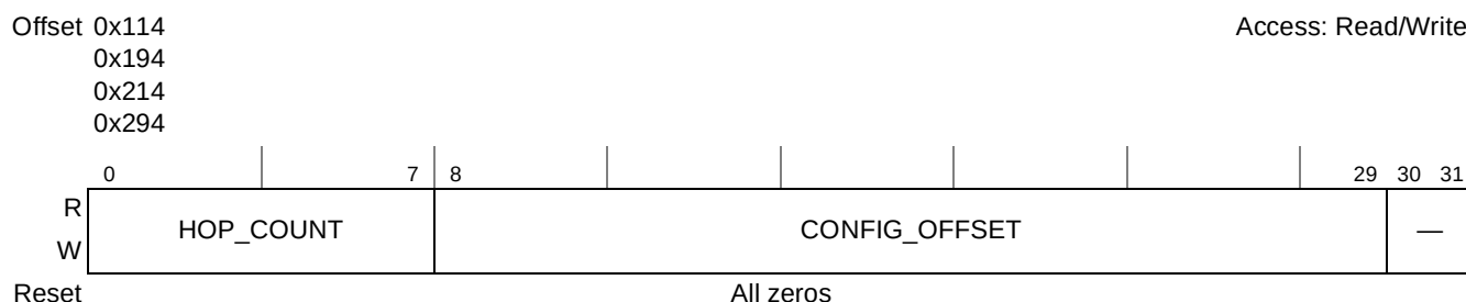
Figure 13-11. Source Address Registers for RapidIO Maintenance Reads (SAR n )
