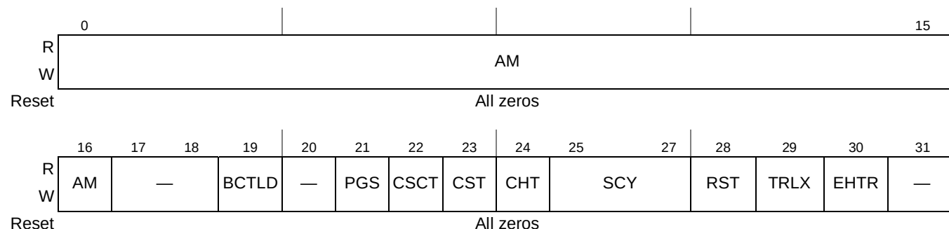
Figure 12-4. Option Registers (OR n ) in FCM Mode
