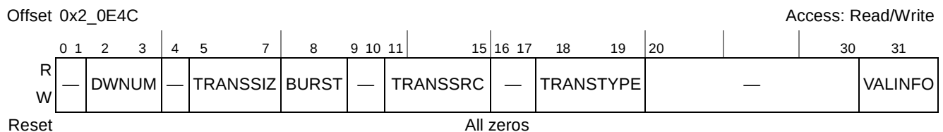
Figure 6-22. L2 Error Attributes Capture Register (L2ERRATTR)
