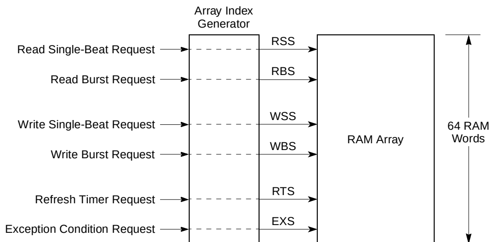
Figure 12-62. RAM Array Indexing
