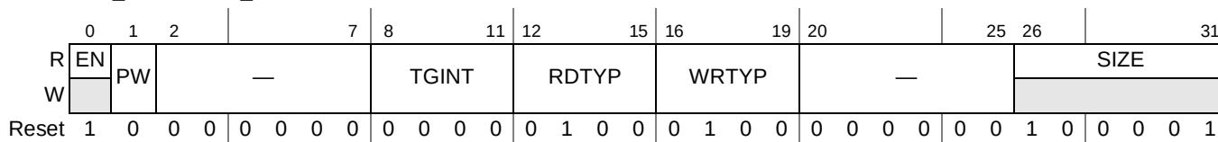
Figure 15-63. Port n RapidIO Inbound Window Attributes Register 0
