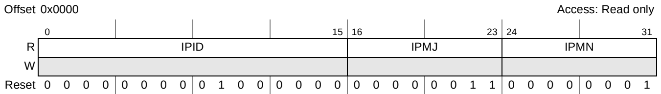
Figure 9-3. Block Revision Register 1 (BRR1)
