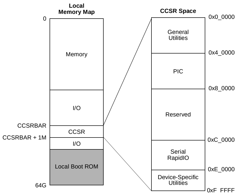
Figure 2-4. CCSR Space
