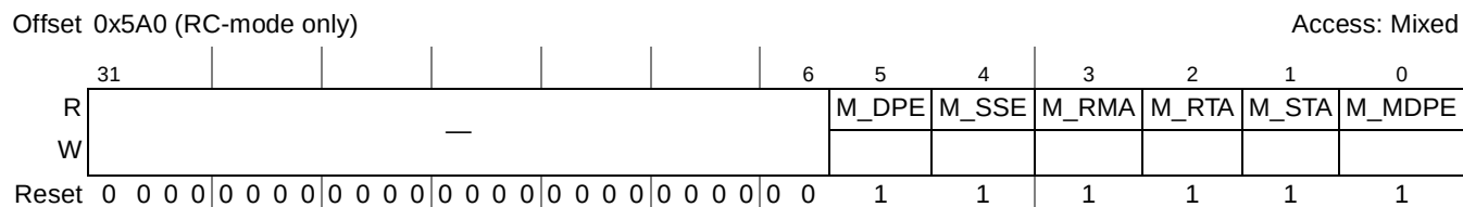
Figure 16-122. PCI Express PCI Interrupt Mask Register (PEX_SS_INTR_MASK)
