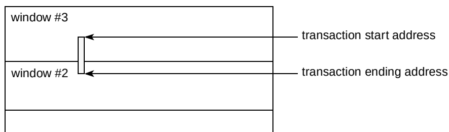
Figure 15-103. Window Boundary Crossing Error—Case 1
