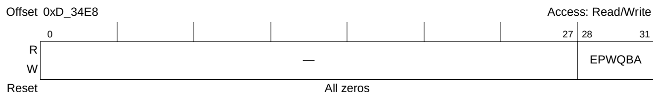
Figure 15-99. Extended Port-Write Queue Base Address Register (EIPWQBAR)
