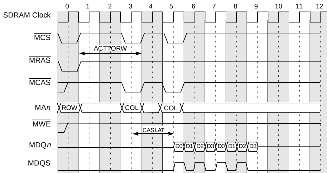
Figure 8-51. DDR SDRAM Burst Read Timing—ACTTORW = 3, MCAS Latency = 2
