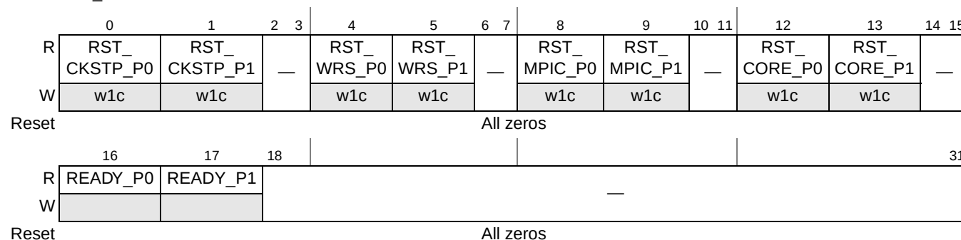
Figure 22-14. Automatic Reset Status Register (AUTORSTSR)
