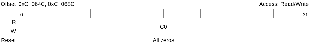
Figure 15-34. Port n Packet/Control Symbol Error Capture Command and Status Register 0 ( PnPCSECCSR0 )
