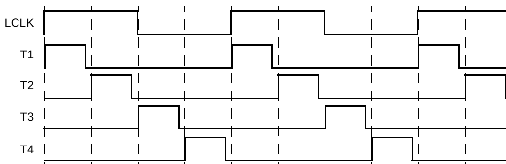
Figure 12-64. UPM Clock Scheme
