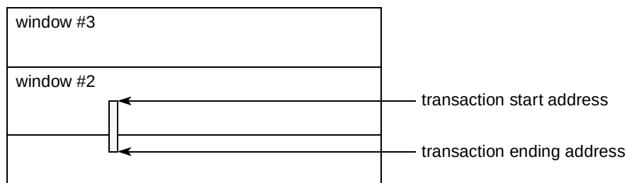
Figure 15-104. Window Boundary Crossing Error—Case 2
