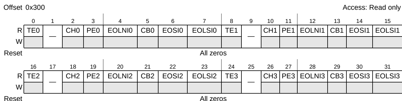
Figure 13-24. DMA General Status Register (DGSR)
