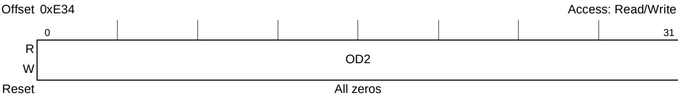
Figure 16-35. PCI Express Error Capture Register 3 (PEX_ERR_CAP_R3) Internal Source, Outbound Transaction
