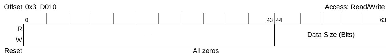
Figure 20-109. STEU Data Size Register
