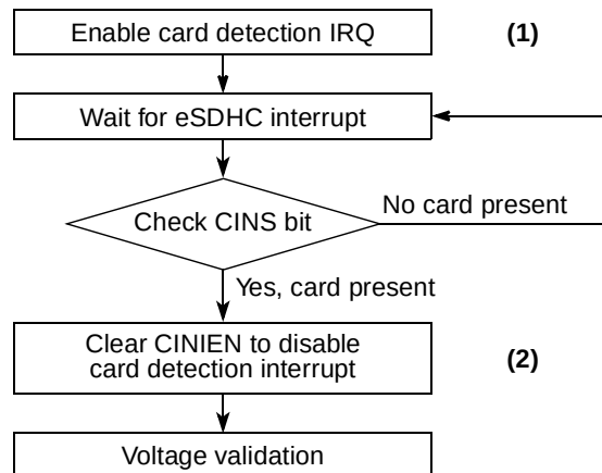
Figure 17-25. Flow Diagram for Card Detection
