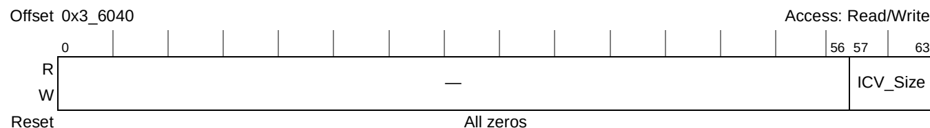
Figure 20-88. MDEU ICV Size Register
