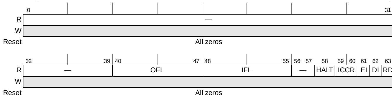
Figure 20-68. KEU Status Register
