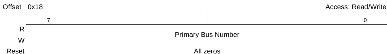
Figure 16-61. PCI Express Primary Bus Number Register
