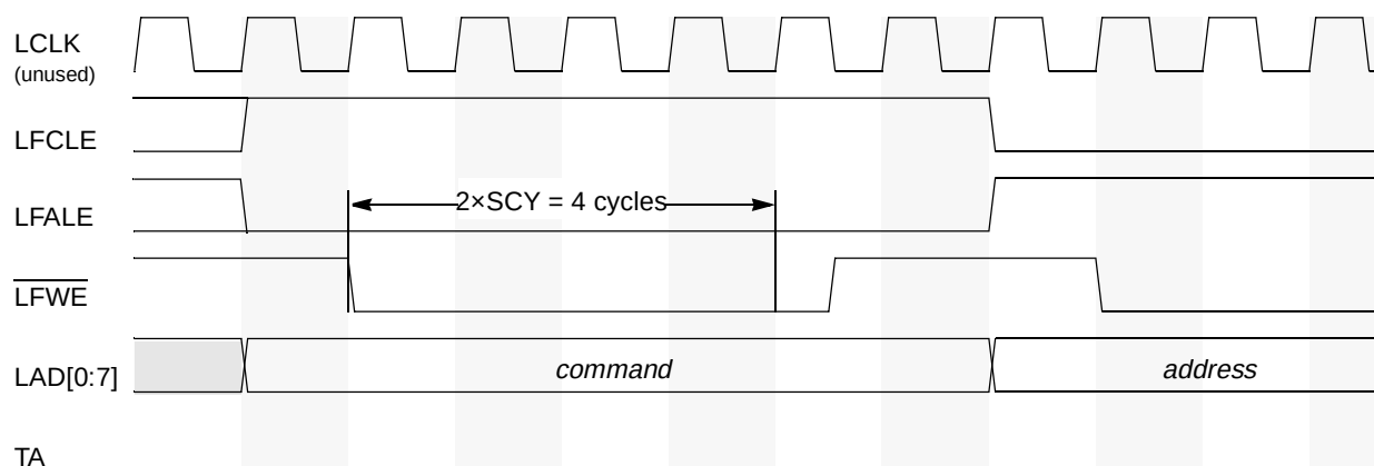
Figure 12-56. Example of FCM Command and Address Timing with Relaxed Parameters (for TRLX = 1 , CHT = 0 , CST = 1 , SCY = 2 )
