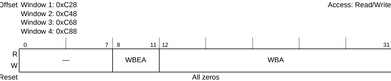
Figure 16-16. PCI Express Outbound Window Base Address Registers (PEXOWBAR n )
