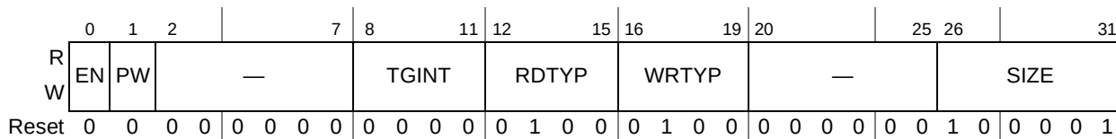
Figure 15-62. Port n RapidIO Inbound Window Attributes Register 1–4
