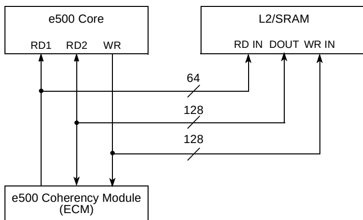
Figure 6-5. Data Bus Connection of CCB
