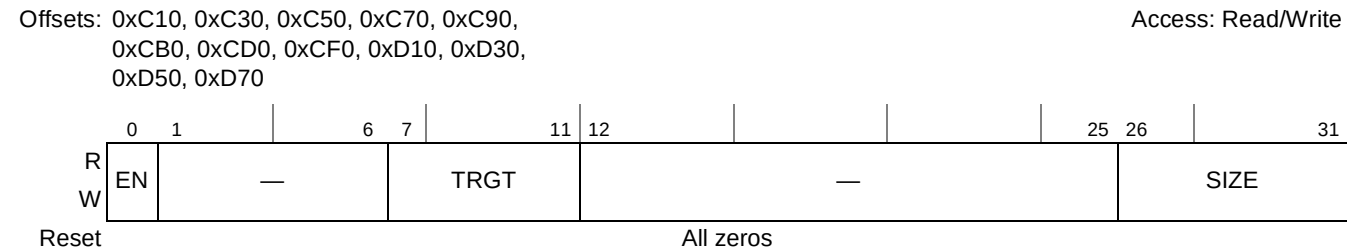
Figure 2-2. Local Access Window Attributes Registers (LAWAR0 to LAWAR9)
