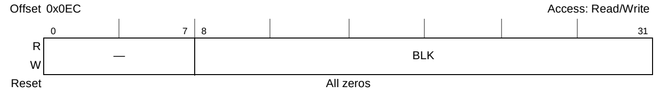
Figure 12-24. Flash Block Address Register
