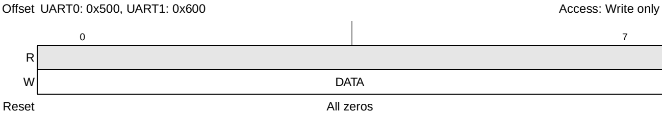
Figure 11-3. Transmitter Holding Registers (UTHR n )
