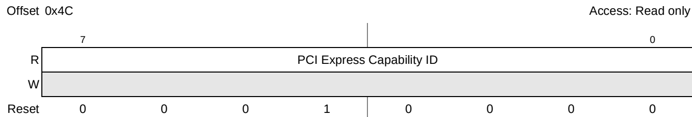
Figure 16-84. PCI Express Capability ID Register
