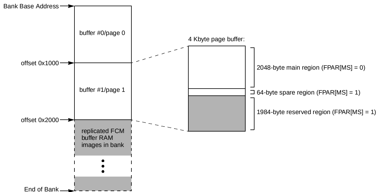
Figure 12-49. FCM Buffer RAM Memory Map for Large-Page (2-Kbyte page) NAND Flash Devices
