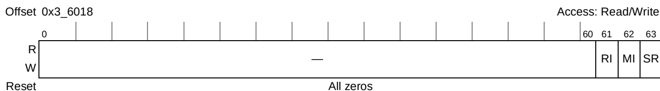
Figure 20-84. MDEU Reset Control Register
