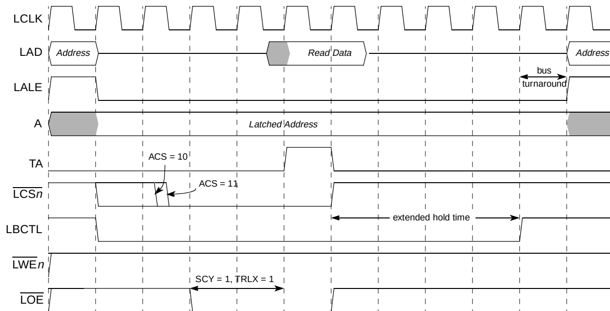
Figure 12-39. GPCM Relaxed Timing Back-to-Back Reads (XACS = 0, ACS = 1x, SCY = 1, CSNT = 0, TRLX = 1, EHTR = 0)
