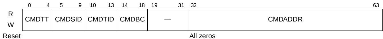
Figure 24-20. e500 Coherency Module Dispatch (CMD) Trace Buffer Entry
