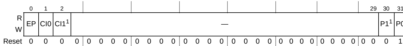
Figure 9-41. Internal Interrupt Destination Registers (IIDRs)
