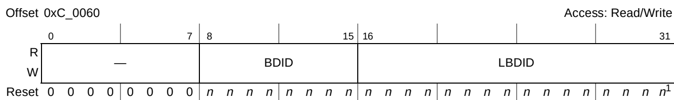
Figure 15-13. Base Device ID Command and Status Register (BDIDCSR)
