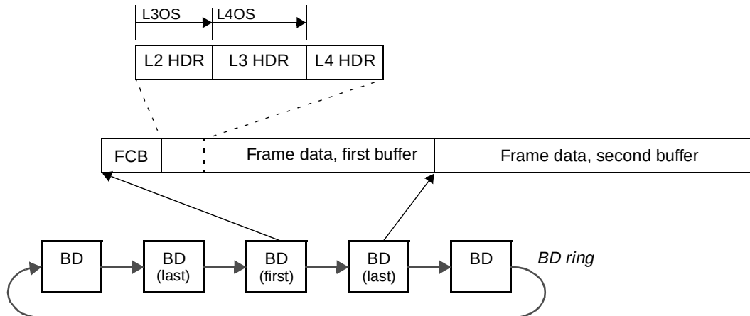
Figure 14-147. Location of Frame Control Blocks for TOE Parameters
