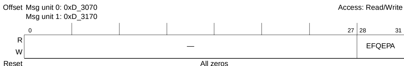
Figure 15-82. Extended Inbound Message n Frame Queue Enqueue Pointer Address Registers (EIMnFQEPAR)
