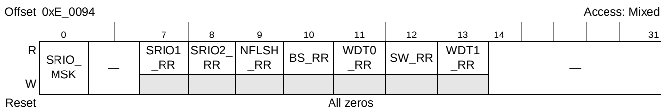
Figure 22-12. Reset Request Status and Control Register (RSTRSCR)
