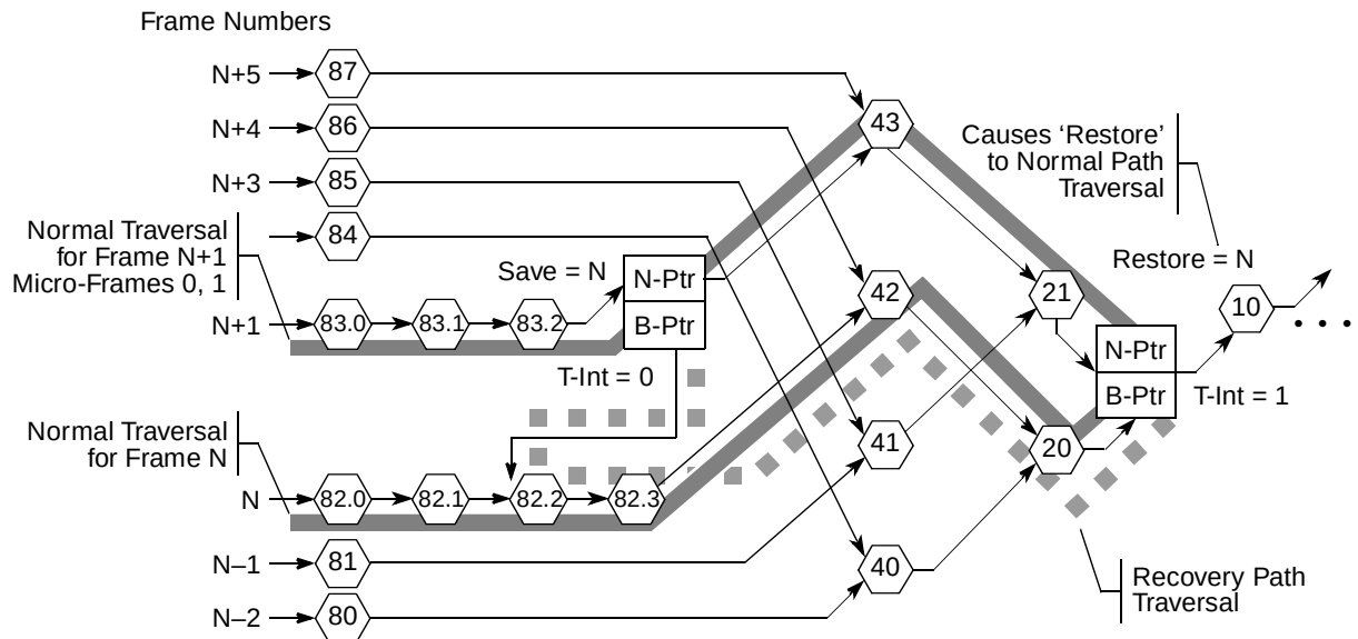
Figure 18-54. Example Host Controller Traversal of Recovery Path via FSTNs
