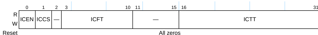
Figure 14-26. RXIC Register Definition
