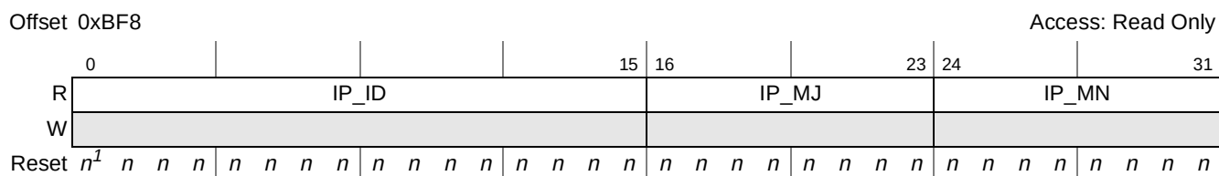
Figure 8-32. DDR IP Block Revision 1 (DDR_IP_REV1)
