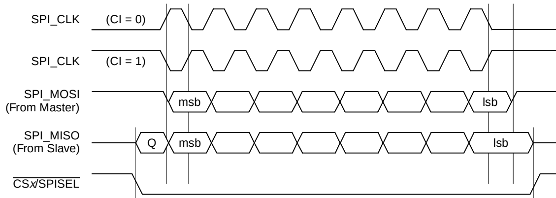
Figure 19-25. eSPI Transfer Format with SPMODEx[CPx] = 1
