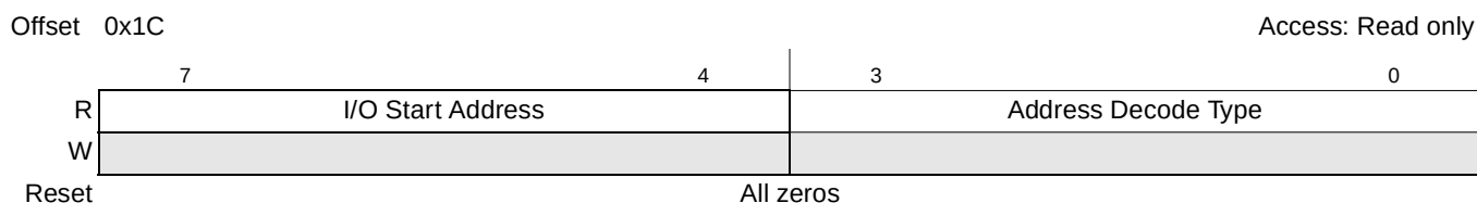
Figure 16-64. PCI Express I/O Base Register
