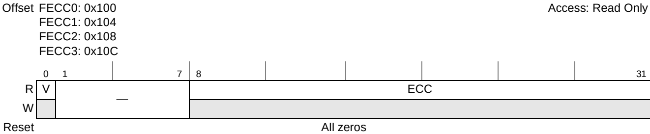
Figure 12-28. Flash ECC Blockn Register (FECC0–FECC3)
