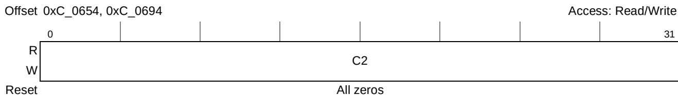
Figure 15-36. Port n Packet Error Capture Command and Status Register 2 ( PnPECCSR2 )
