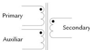
FLYBACK
