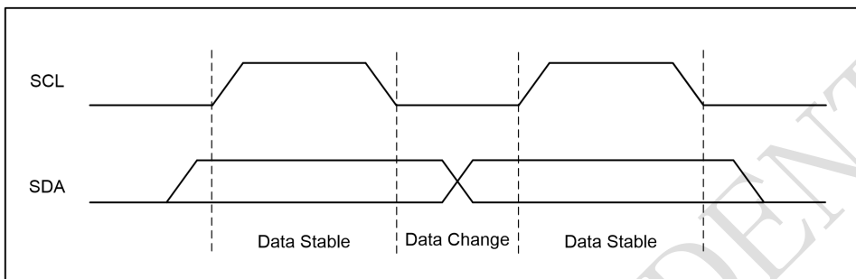
Figure 4-1 Data Validity
