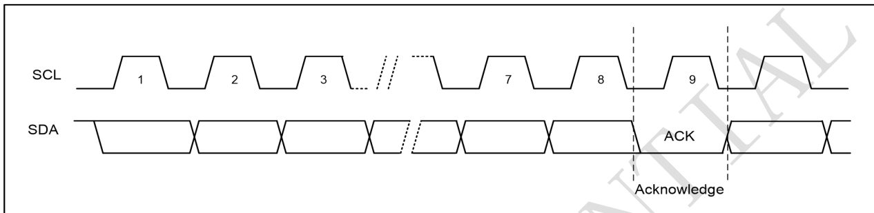
Figure 4-3 Output Acknowledge
