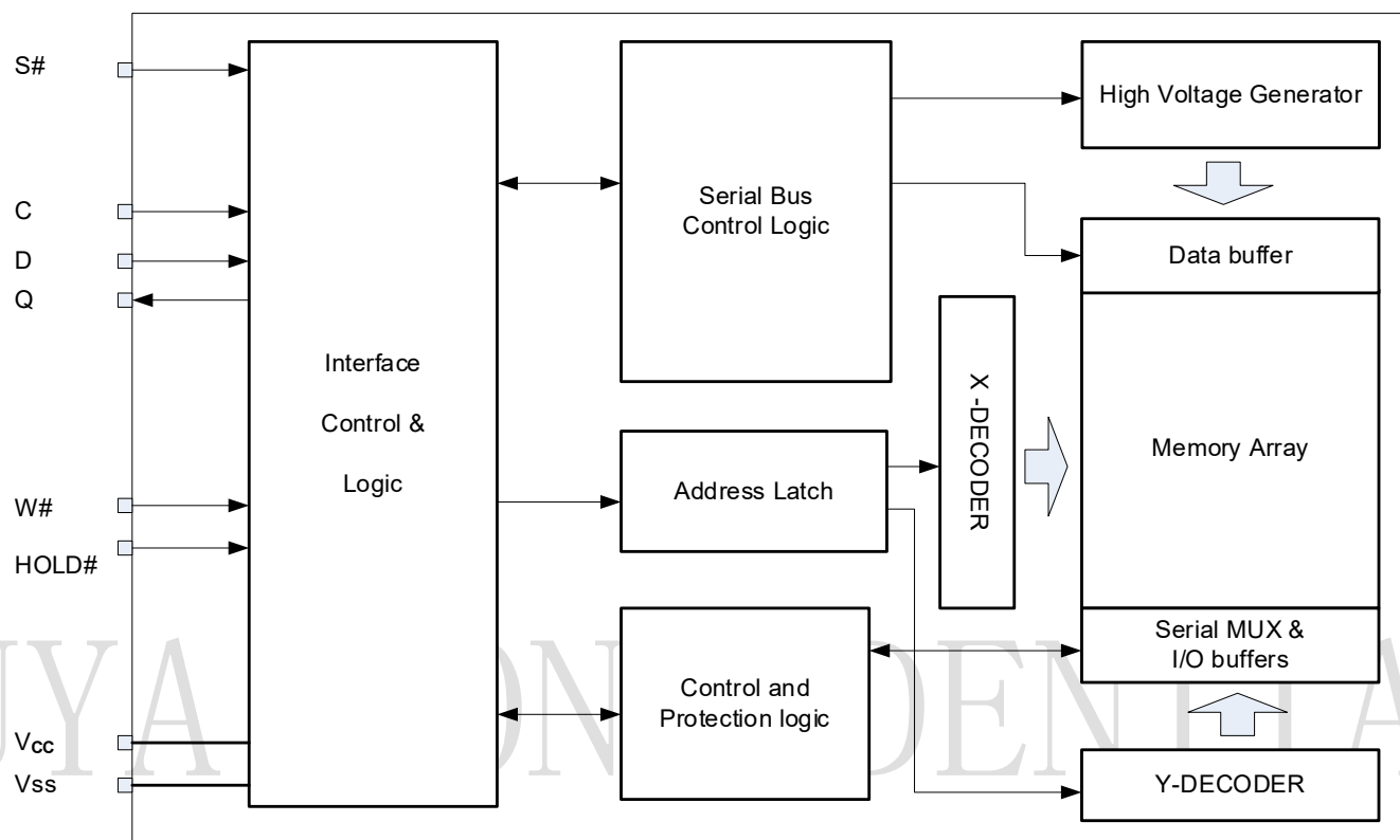
Figure 2-1 Block Diagram
