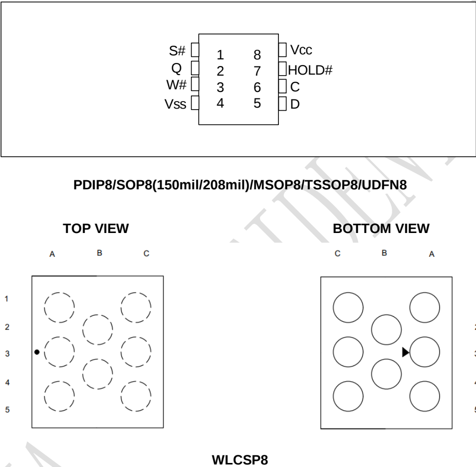
Figure 1-1 Pin Configuration
