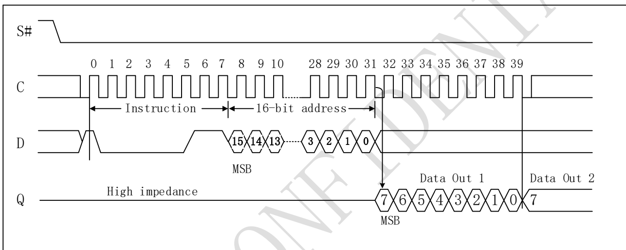
Figure 6-13. Read Lock Status sequence
