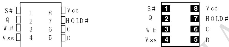
Figure 1-1 8-pin package
