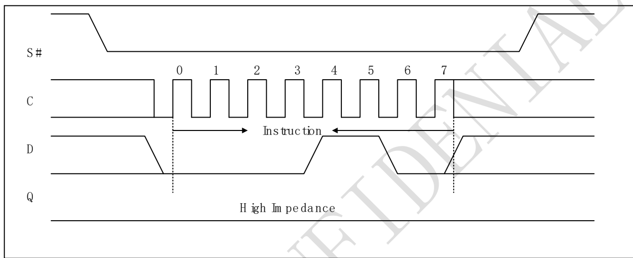
Figure 6-3. Write Enable (WREN) sequence
