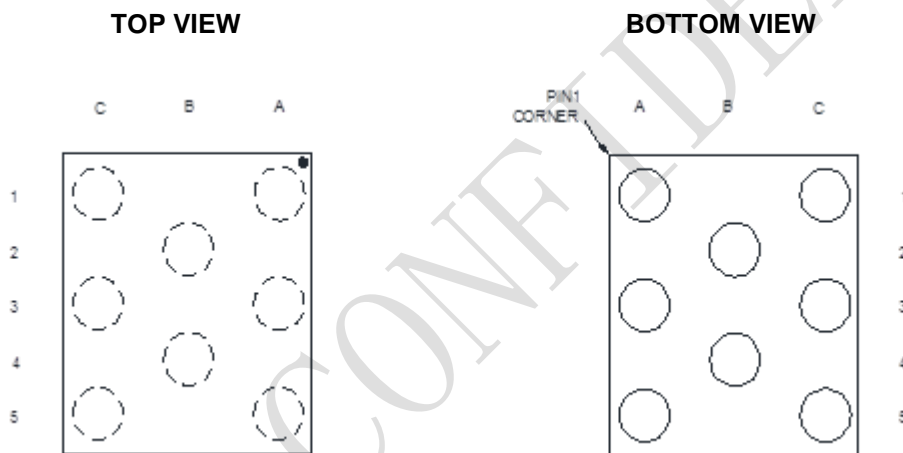
Figure 1-2 WLCSP8
