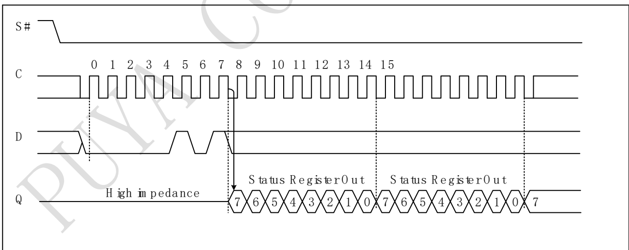
Figure 6-5. Read Status Register (RDSR) sequence
