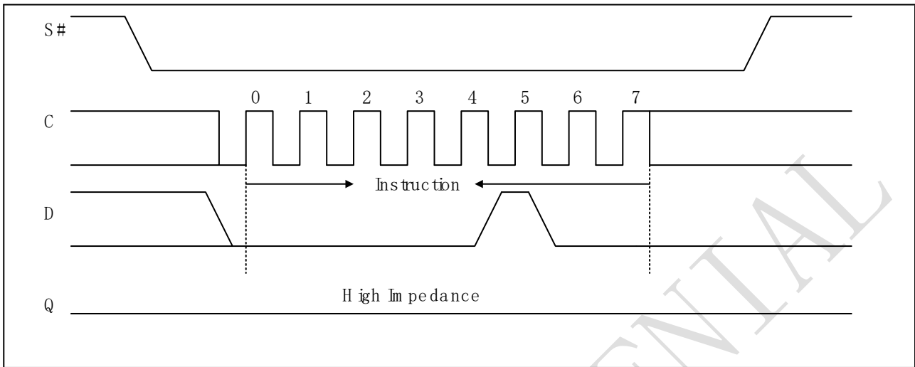
Figure 6-4. Write Disable (WRDI) sequence
