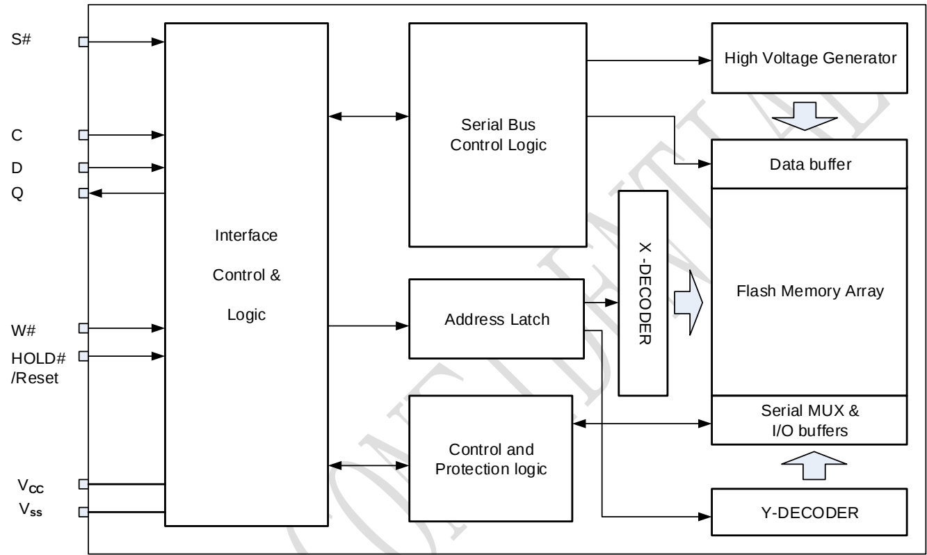
Figure 2-1 Block Diagram
