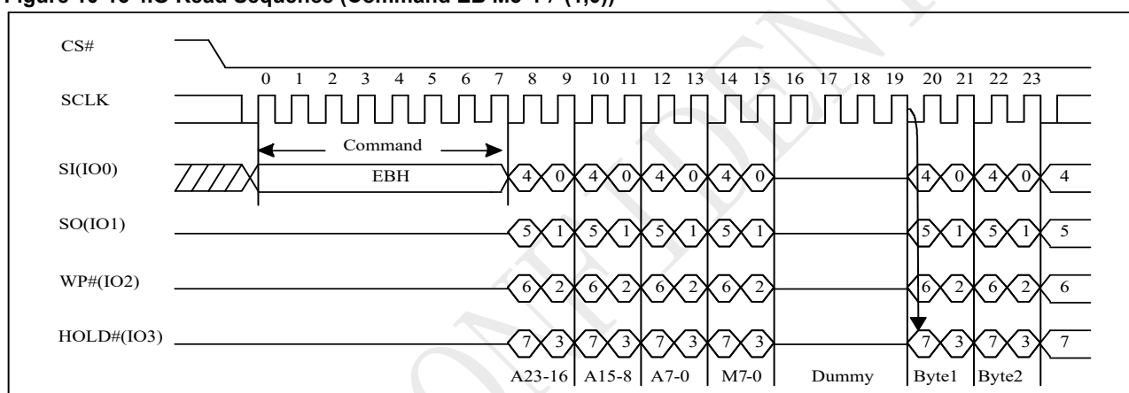
Figure 10-16 4IO Read Sequence (Command EB M5-4 ≠ (1,0))
