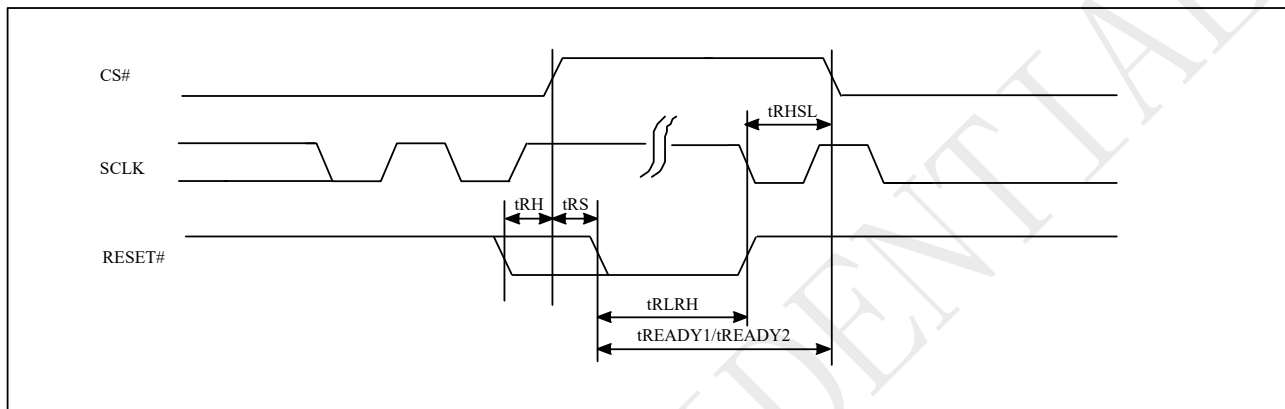
Figure 10-57 RESET Timing
