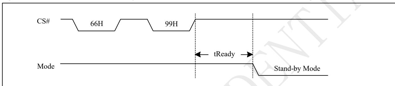
Figure 10-56a Reset Sequence
