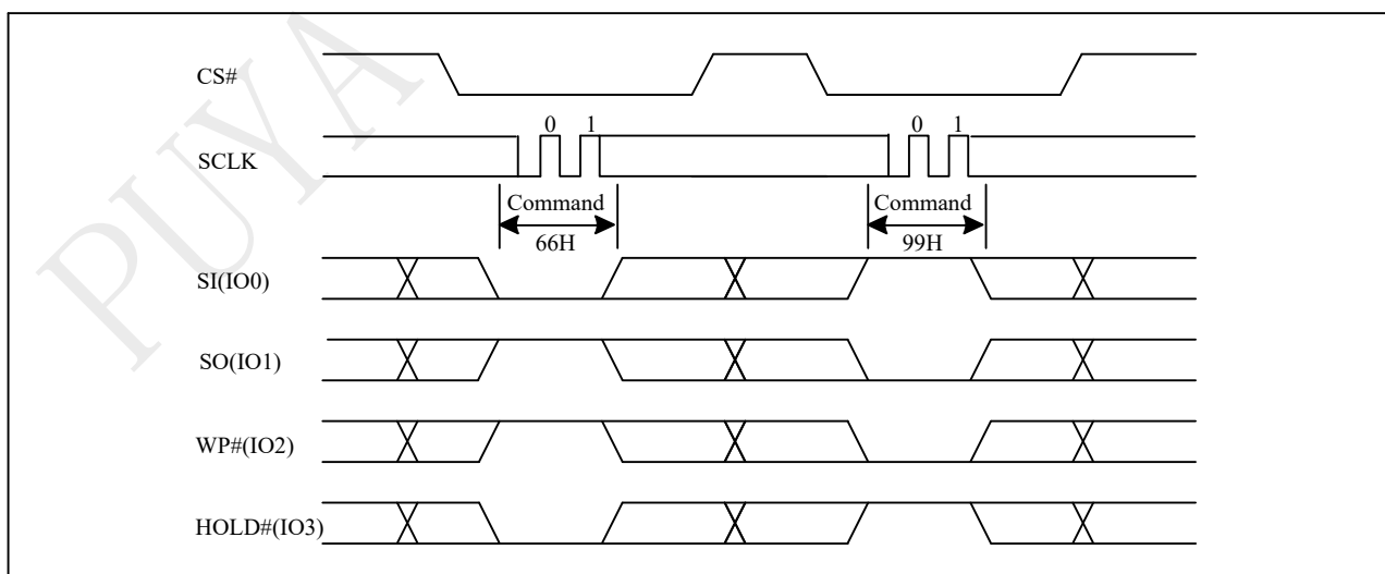
Figure 10-56b Reset Sequence(QPI)
