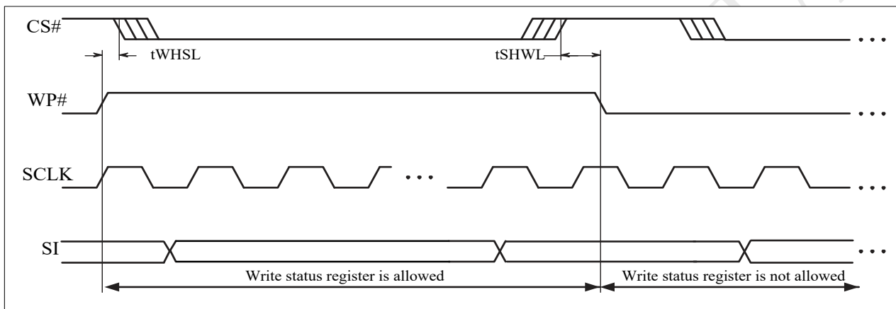
Figure 5-7 WP Timing
