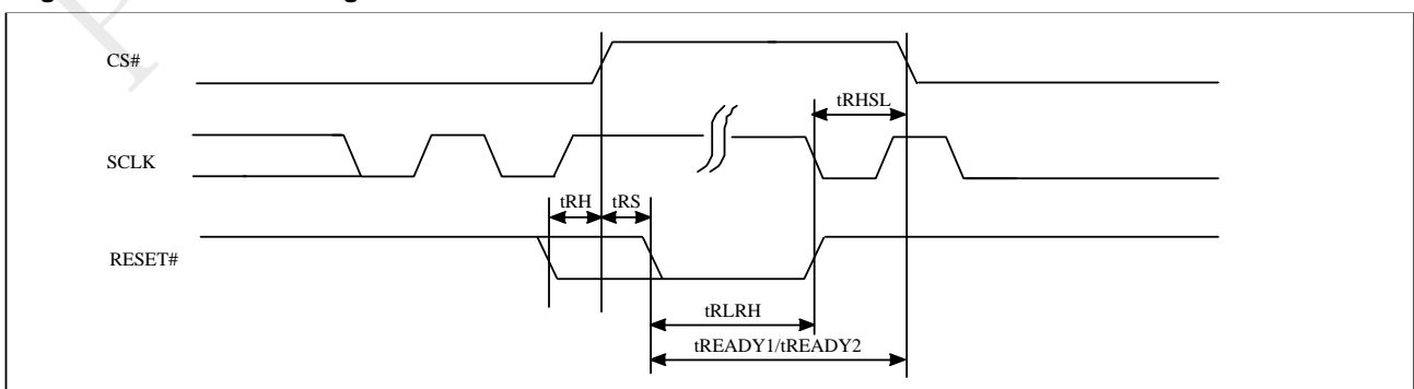
Figure 10-54 RESET Timing
