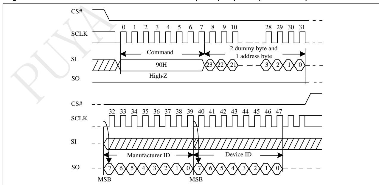
Figure 10-40 Read Electronic Manufacturer &amp; Device ID (REMS) Sequence (Command 90)
