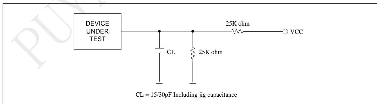
Figure 5-3 Output Loading
