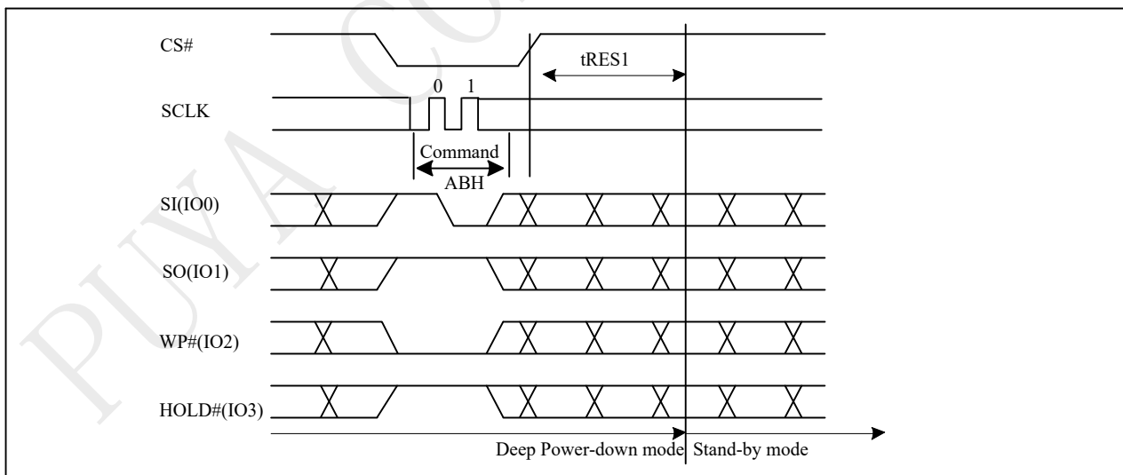
Figure 10-42c Release from Deep Power-down (RDP) Sequence (QPI)
