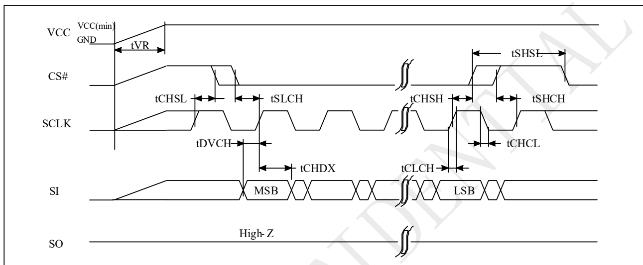
Figure 5-9 Power-up Timing
