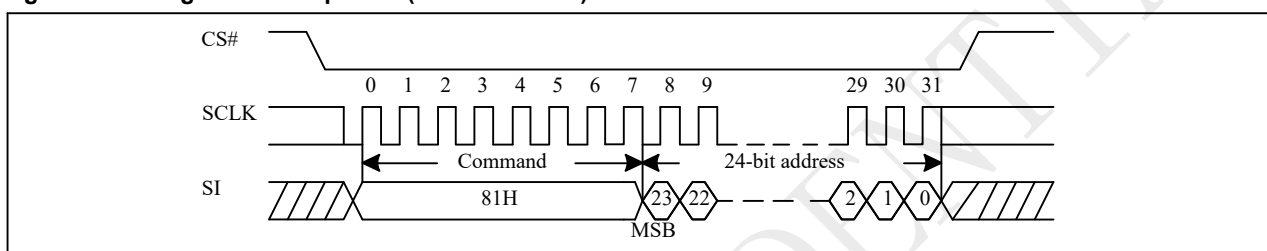
Figure 10-26 Page Erase Sequence (Command 81h)
