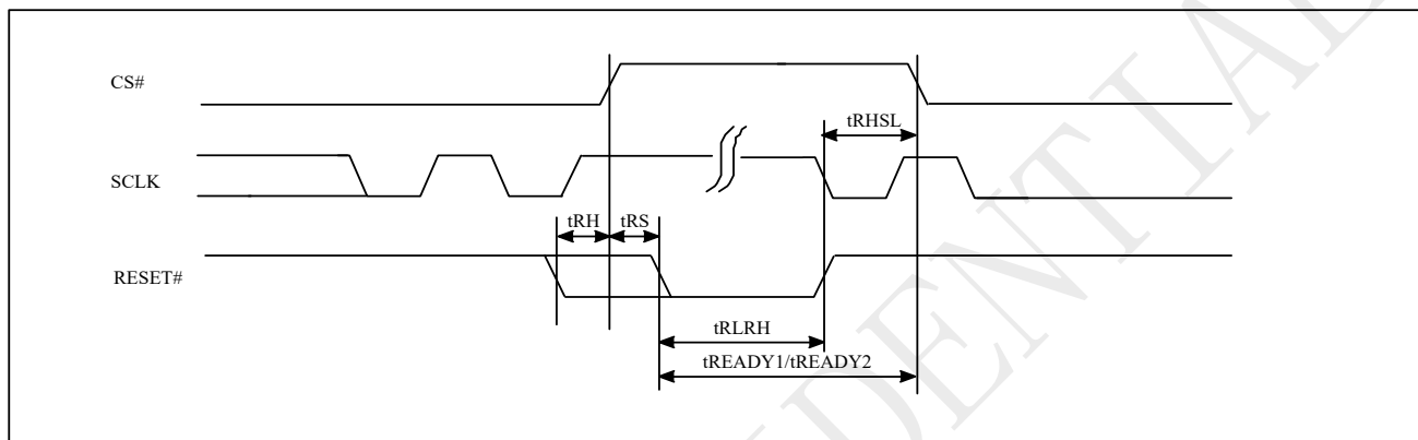
Figure 10-57 RESET Timing
