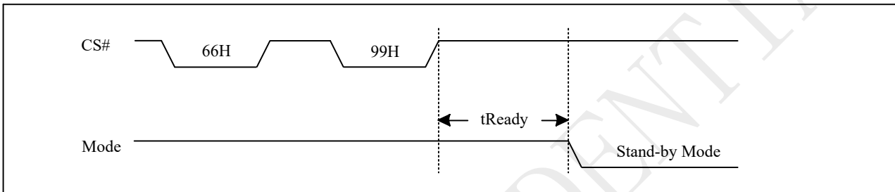
Figure 10-56a Reset Sequence
