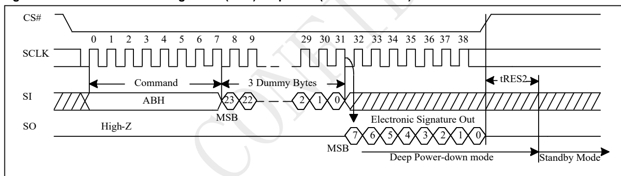
Figure 10-42 Read Electronic Signature (RES) Sequence (Command ABh)
