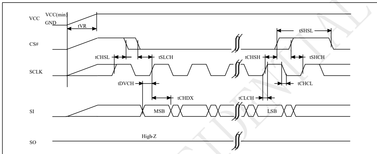
Figure 5-9 Power-up Timing
