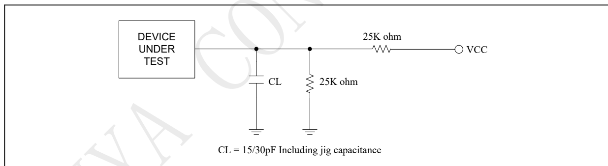
Figure 5-2 Output Loading
