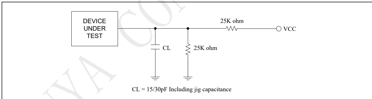
Figure 5-2 Output Loading
