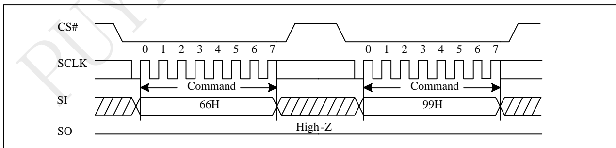
Figure 10-41 Reset Sequence
