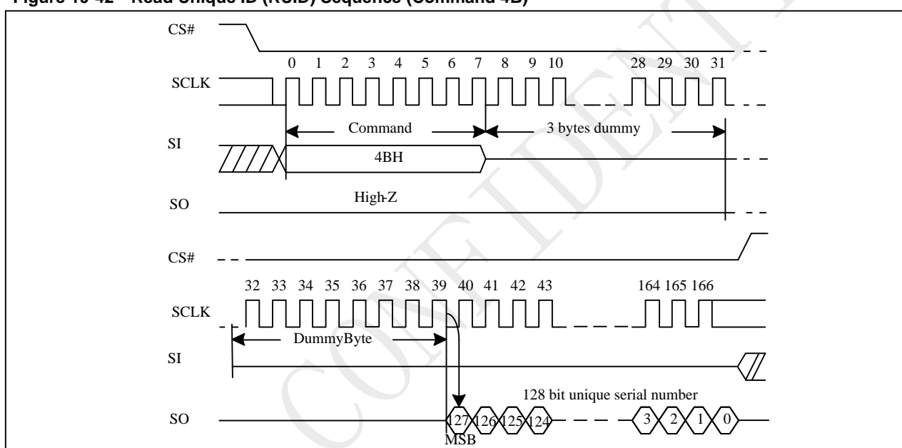
Figure 10-42 Read Unique ID (RUID) Sequence (Command 4B)
