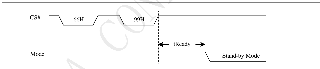
Figure 10-41 Reset Sequence
