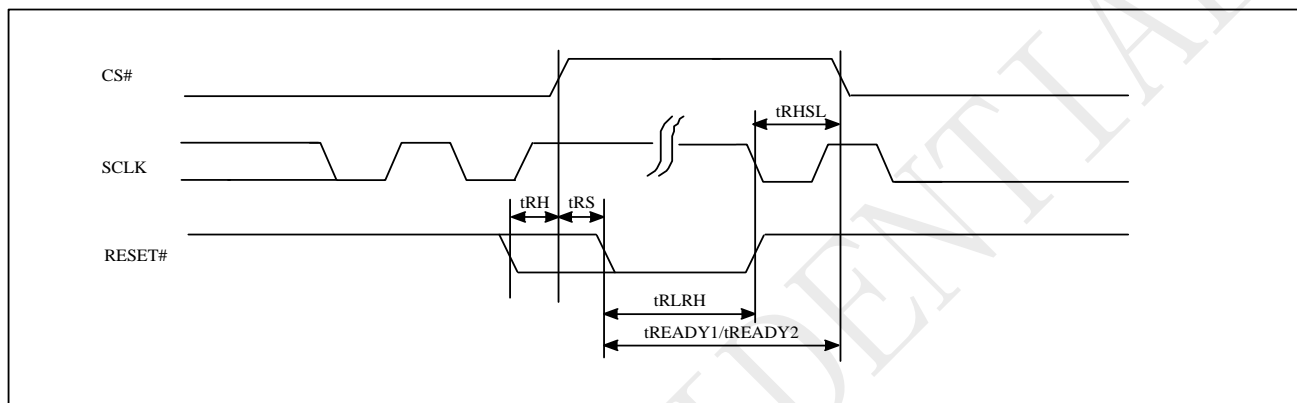
Figure 10-57 Reset Timing
