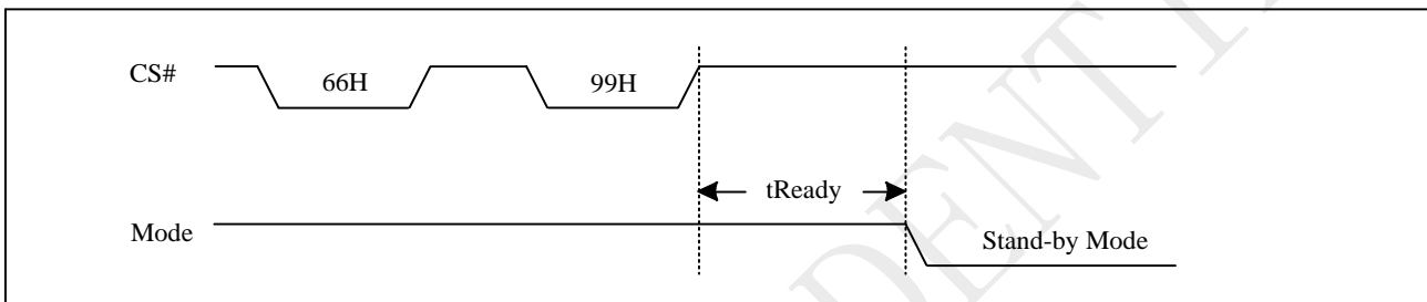
Figure 10-56a Reset Sequence
