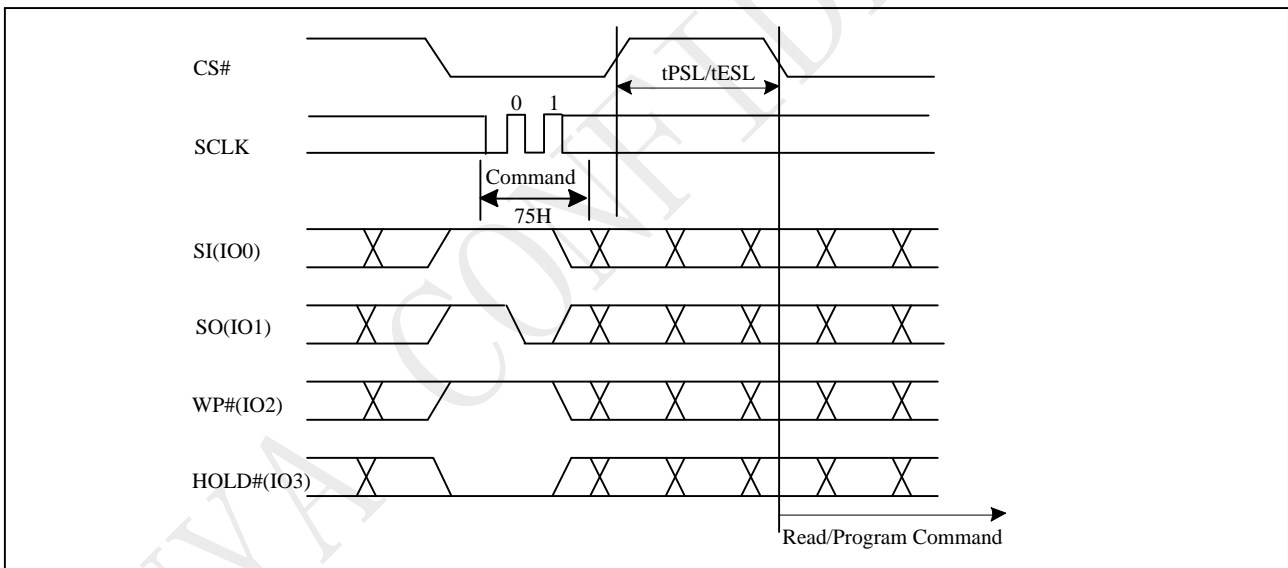
Figure 10-48a Suspend to Read/Program Latency(QPI)
