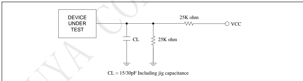
Figure 5-2 Output Loading
