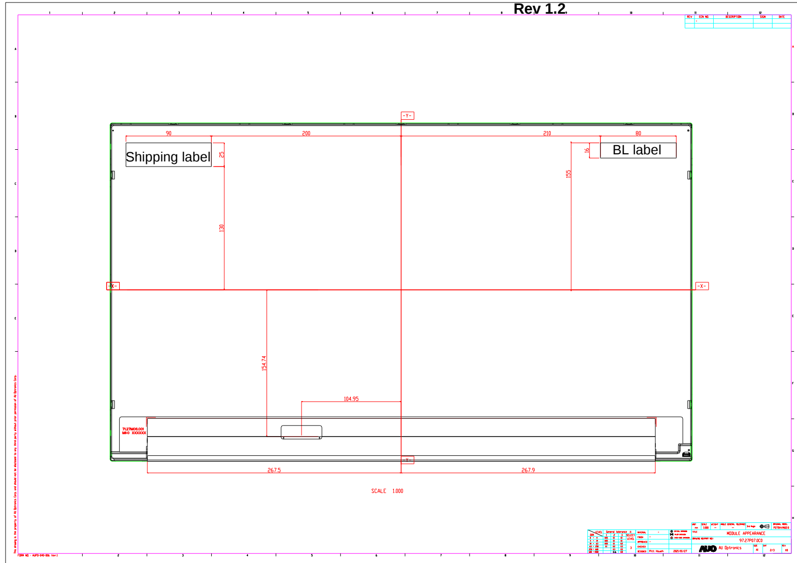
Back View
