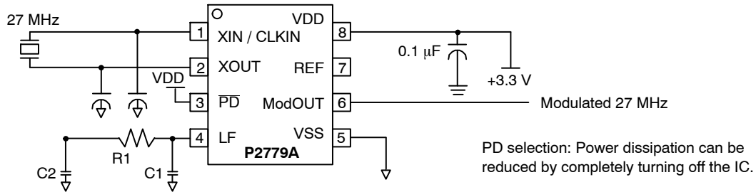
Figure 2. Application Schematic
