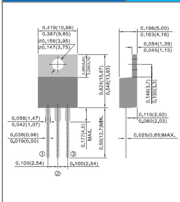
TO-220AB Dimension
