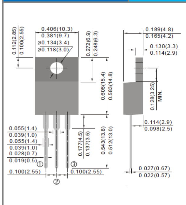
ITO-220AB Dimension
