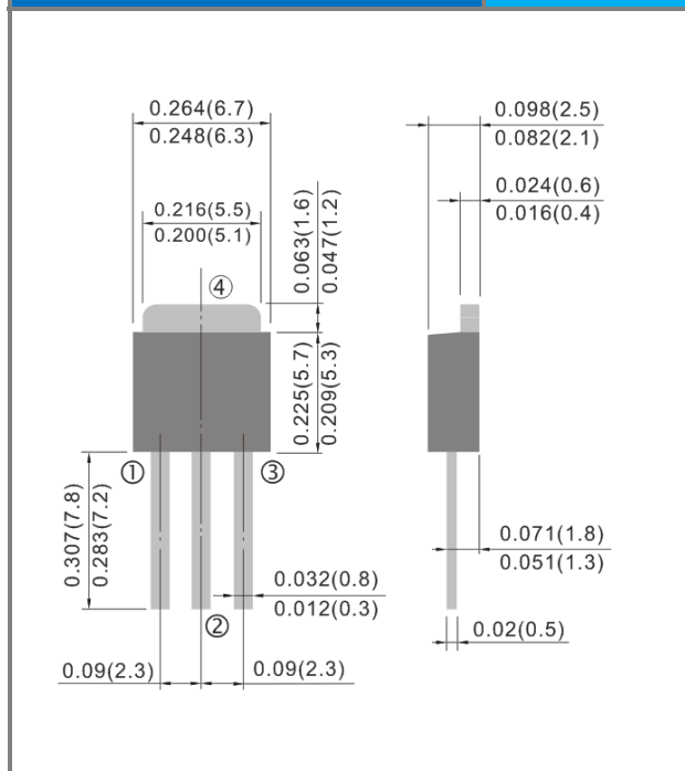
TO-251AB Dimension
