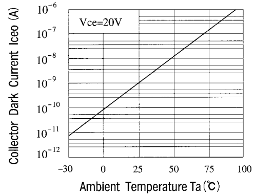
Fig 3 Collector Dark Current vs. Ambient Temperature
