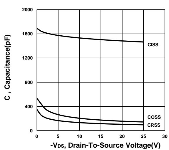
Capacitance Characteristic
