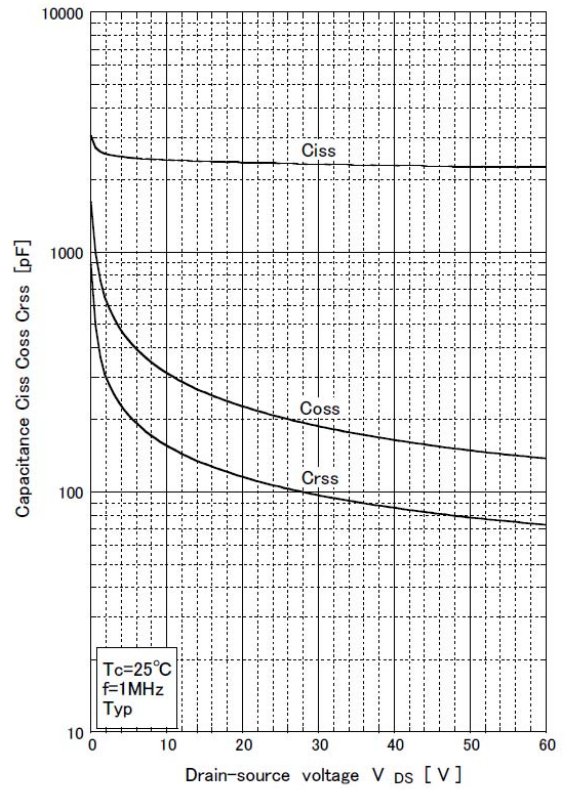
Capacitance characteristics
