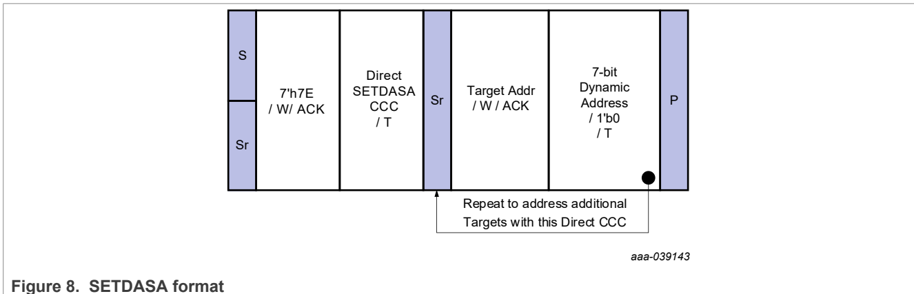
Figure 8. SETDASA format
