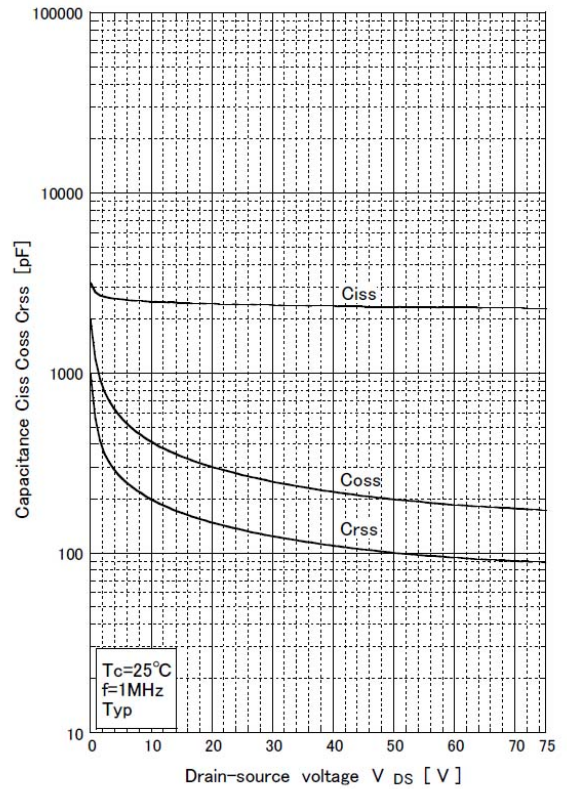
Capacitance characteristics
