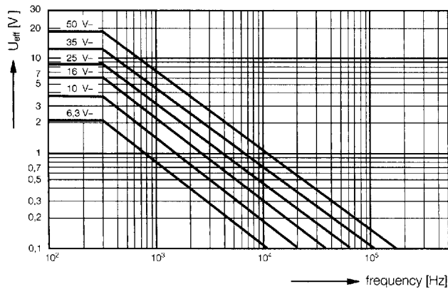
Diagram 17: Permissible superimposed AC voltage versus rated voltage and frequency at +20°C ETPW 3
