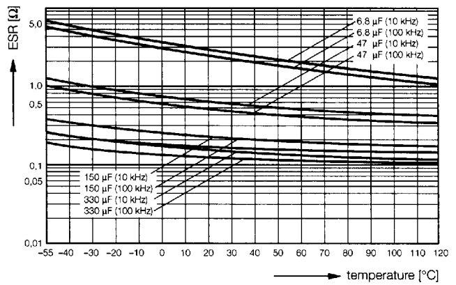
Diagram 11: ESR at 10 and 100 kHz versus temperature (standard value) ETPW with 35 V-
