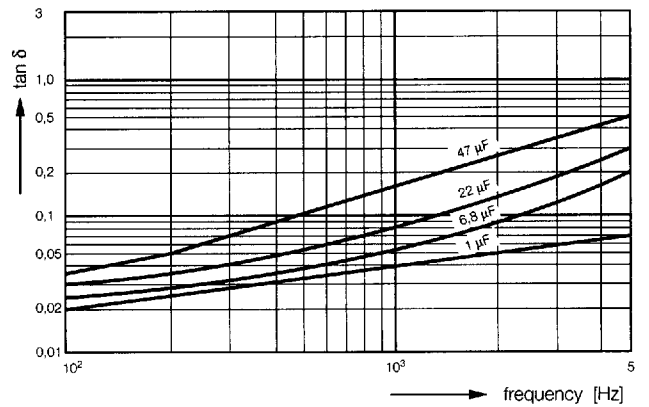
Diagram 6: Dissipation factor versus frequency (standard value) ETPW with 35 V-
