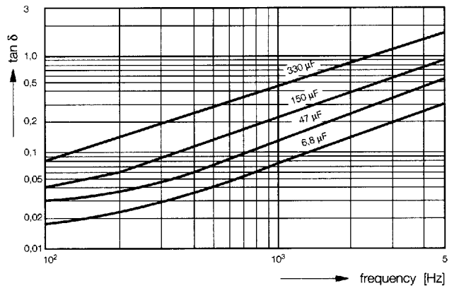
Diagram 5: Dissipation factor versus frequency (standard value) ETPW with 6,3 V-
