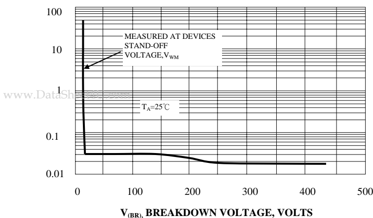
FIG. 6 - TYPICAL REVERSE LEAKAGE CHARACTERISTICS
