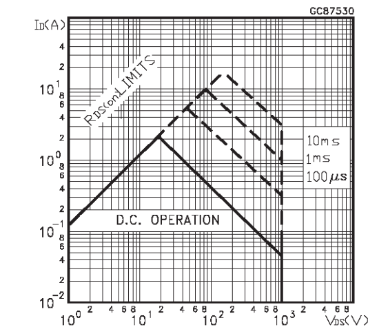
Safe Operating Area for TO-220FP
