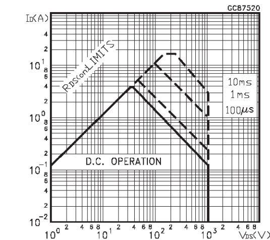
Safe Operating Area for TO-220
