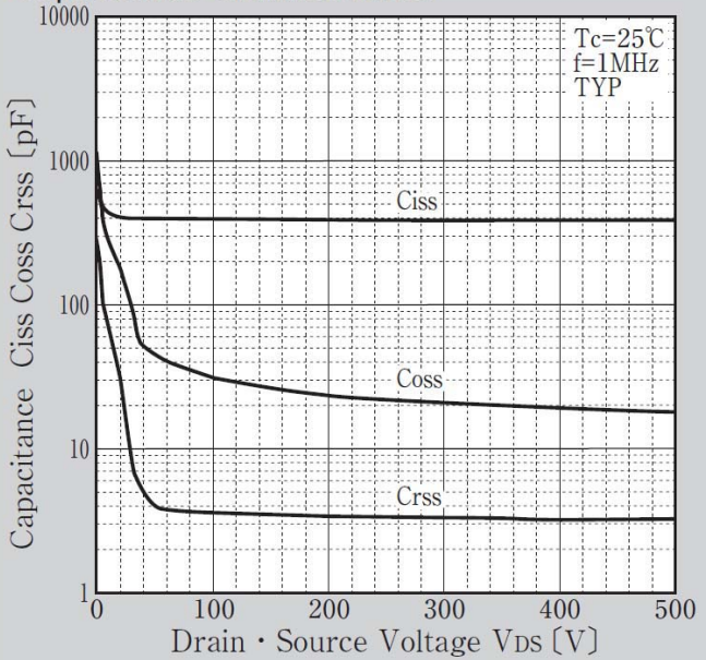
Capacitance Characteristics
