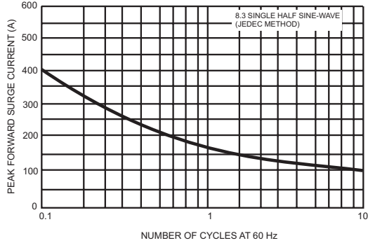
FIG.3- MAXIMUM REPETITIVE FORWARD SURGE CURRENT
