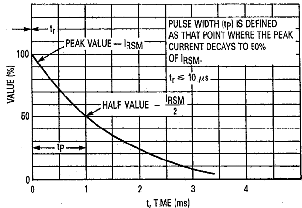
Figure 2. Pulse Waveform
