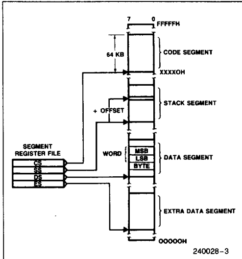
Figure 3. Memory Organization
