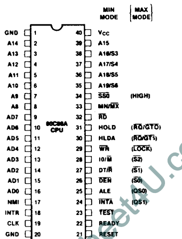
Figure 2. 80C88A 40-Lead DIP Configuration
