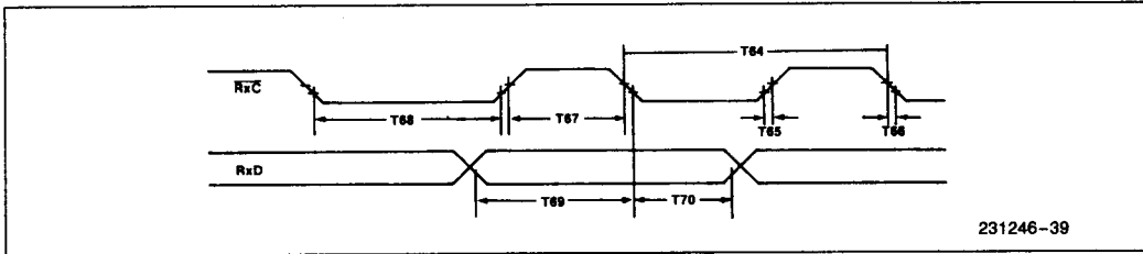
Figure 37. RxD Timing Relative to \overline{RxC}
