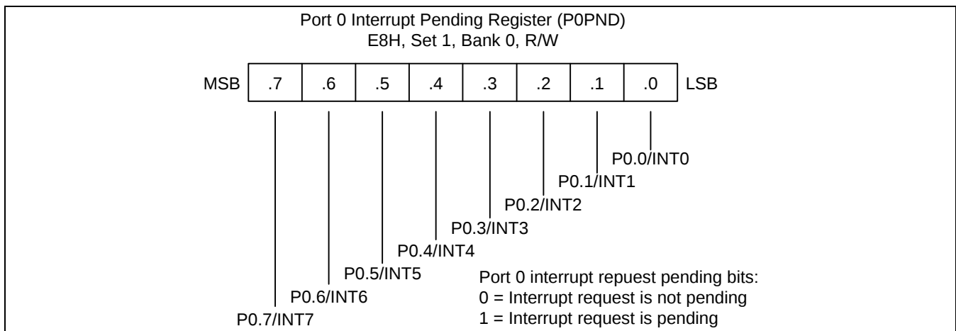
Figure 9-5. Port 0 Interrupt Pending Register (P0PND)
