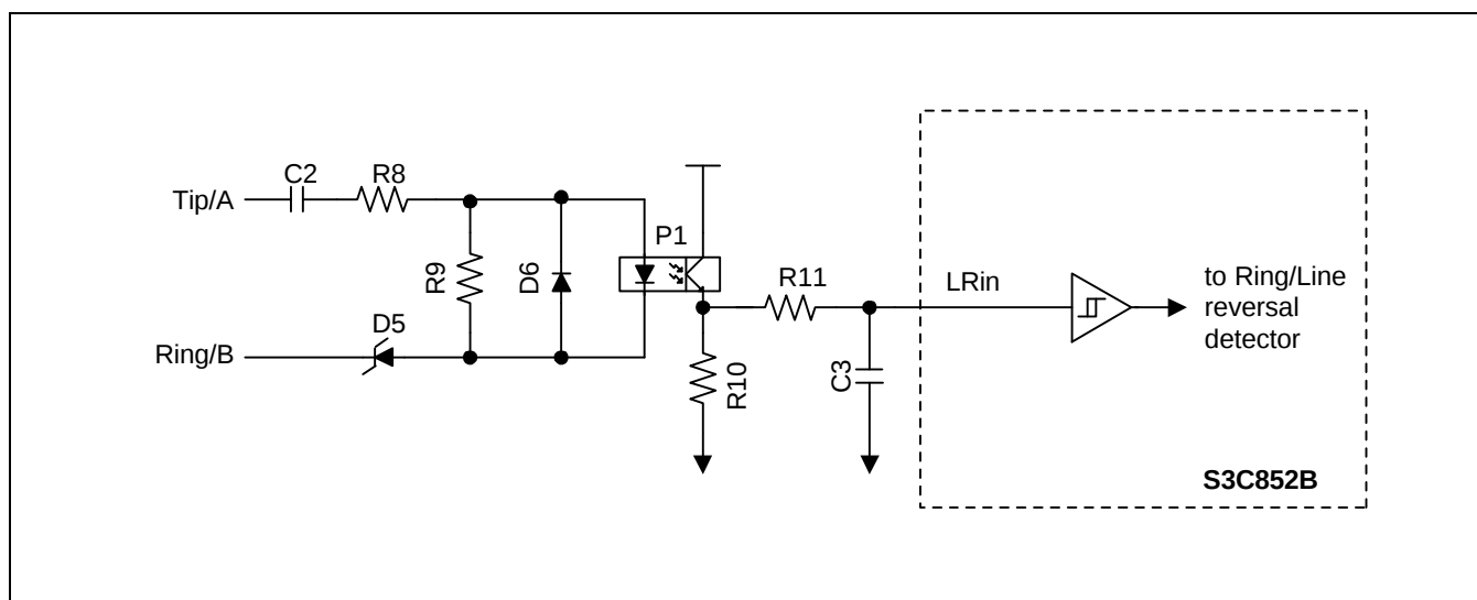
Figure 14-9. External Component to Generate LRin
