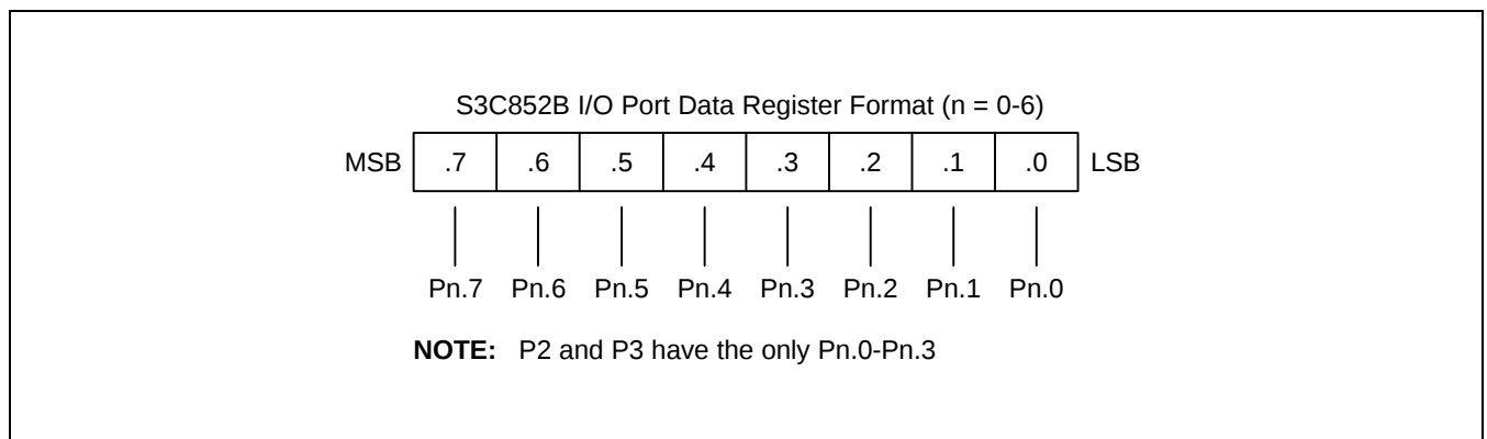
Figure 9-1. S3C852B I/O Port Data Register Format
