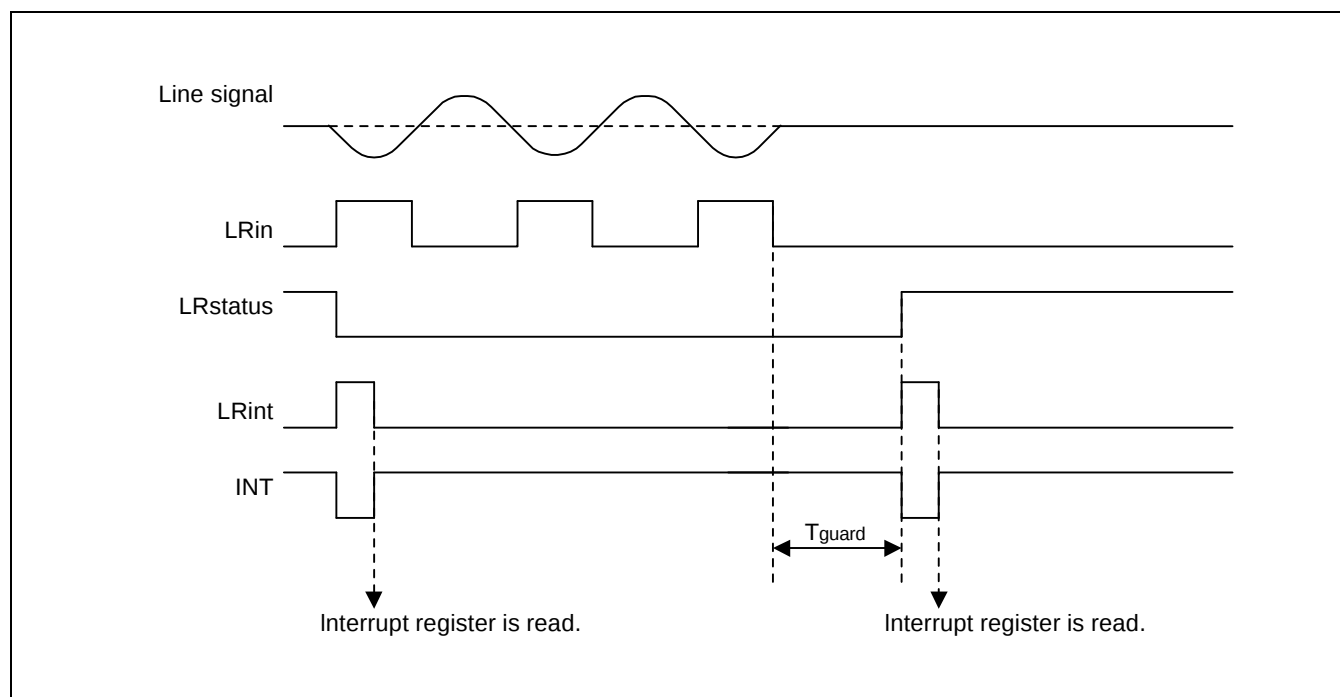
Figure 14-11. Behavior of Signals During Ring
