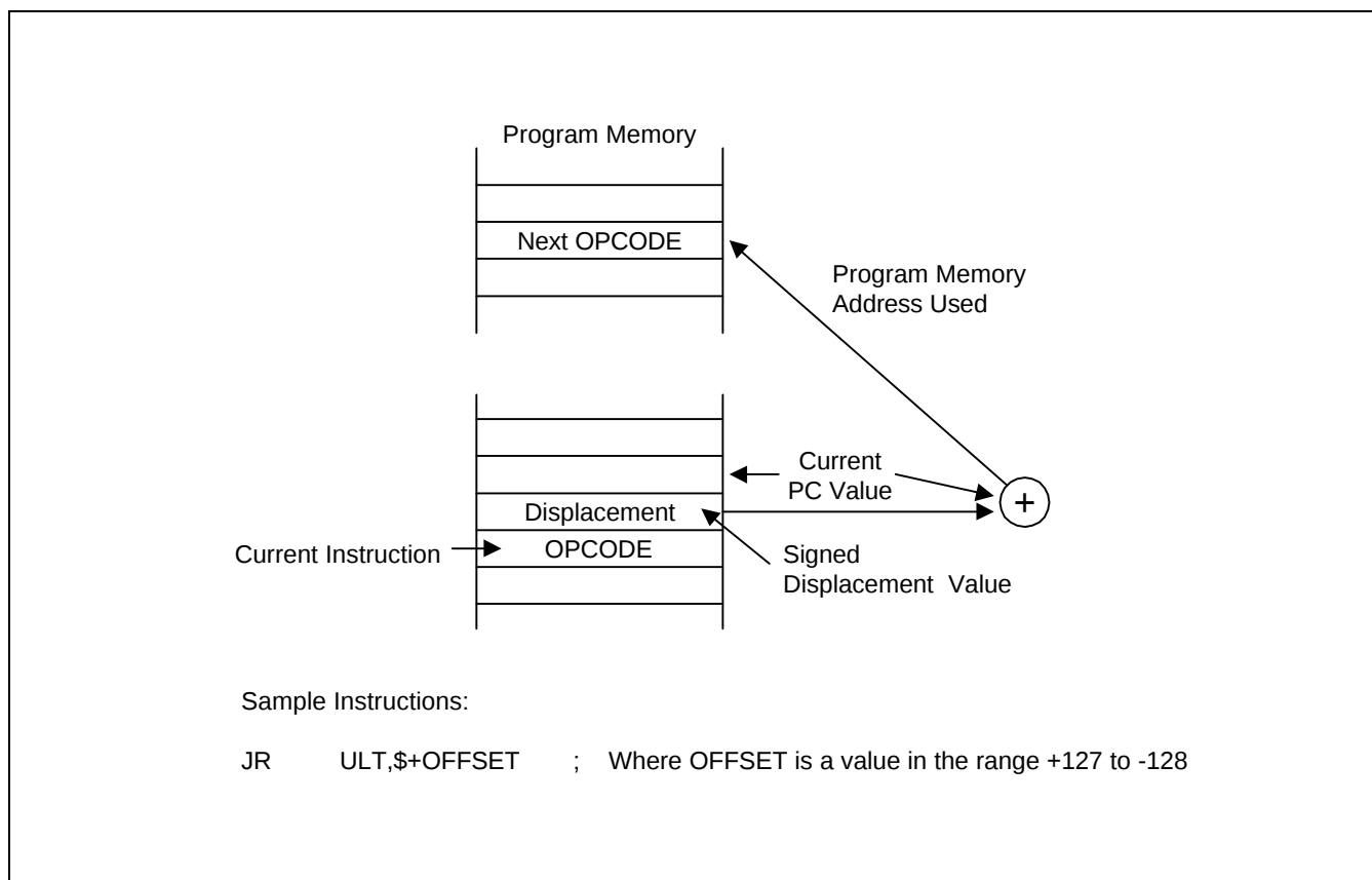
Figure 3-13. Relative Addressing
