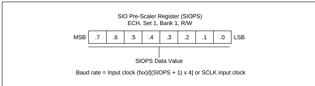
Figure 13-2. SIO Prescaler Register (SIOPS)
