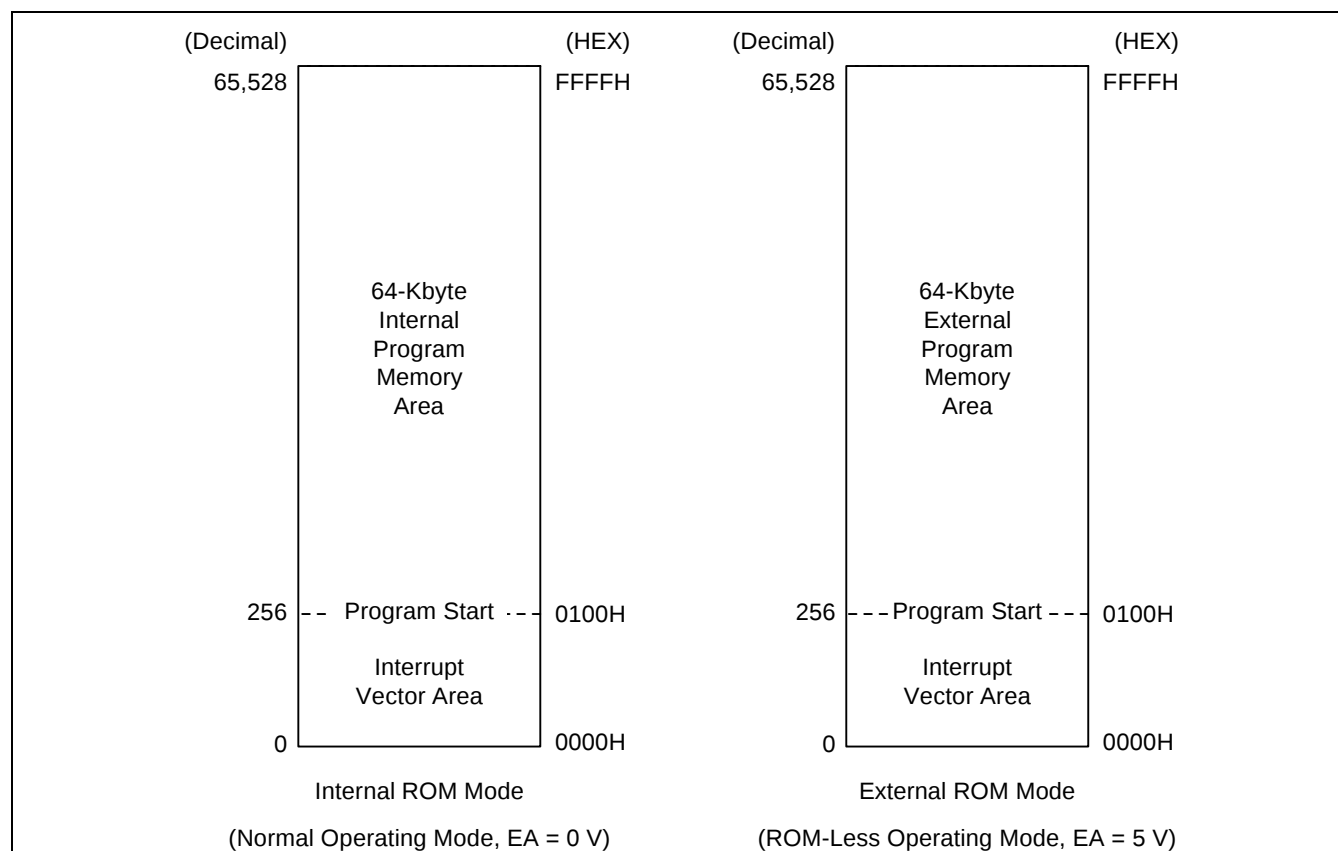
Figure 16-2. Internal and External Program Memory Options
