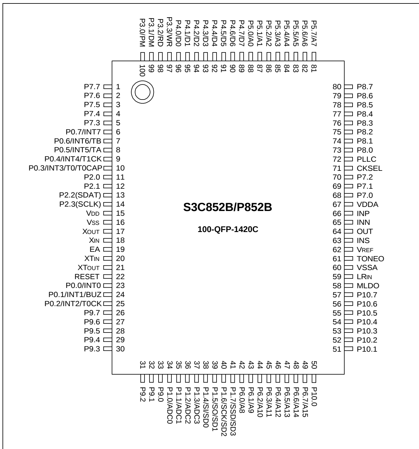
Figure 1-2. Pin Assignment (100-Pin QFP Package)
