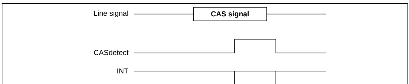
Figure 14-4. CASdetect, CASint and INT Related to the CAS Tone
