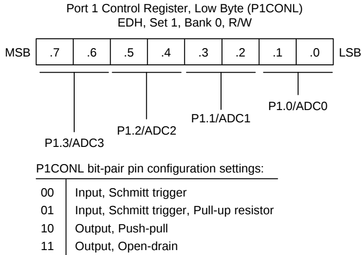
Figure 9-8. Port 1 Low-Byte Control Register (P1CONL)
