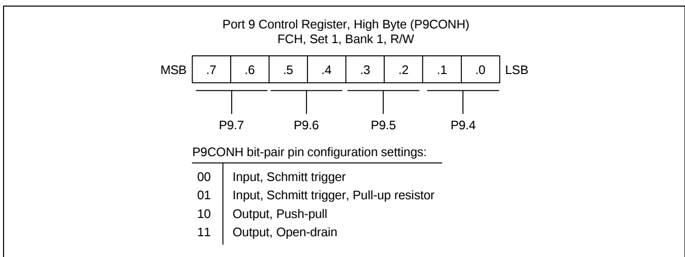
Figure 9-20. Port 9 High-Byte Control Register (P9CONH)
