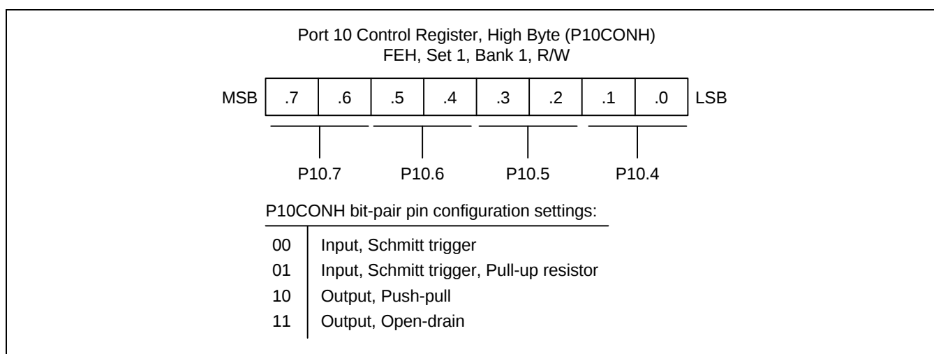
Figure 9-22. Port 10 High-Byte Control Register (P10CONH)
