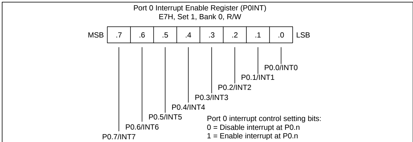
Figure 9-4. Port 0 Interrupt Enable Register (P0INT)
