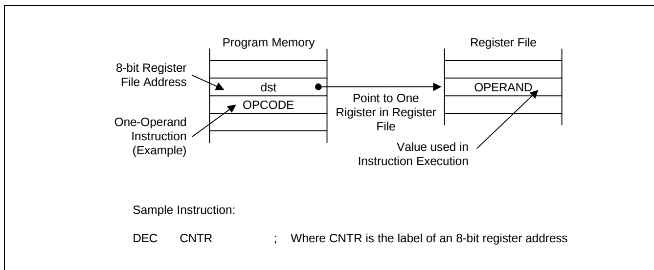
Figure 3-1. Register Addressing
