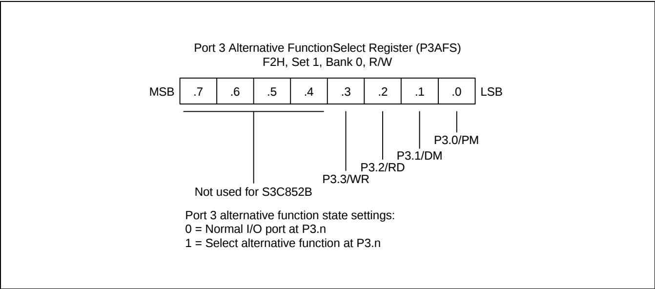
Figure 9-12. Port 3 Alternative Function Select Register (P3AFS)
