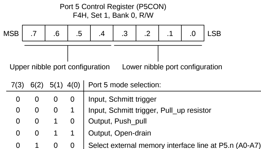
Figure 9-14. Port 5 Control Register (P5CON)
