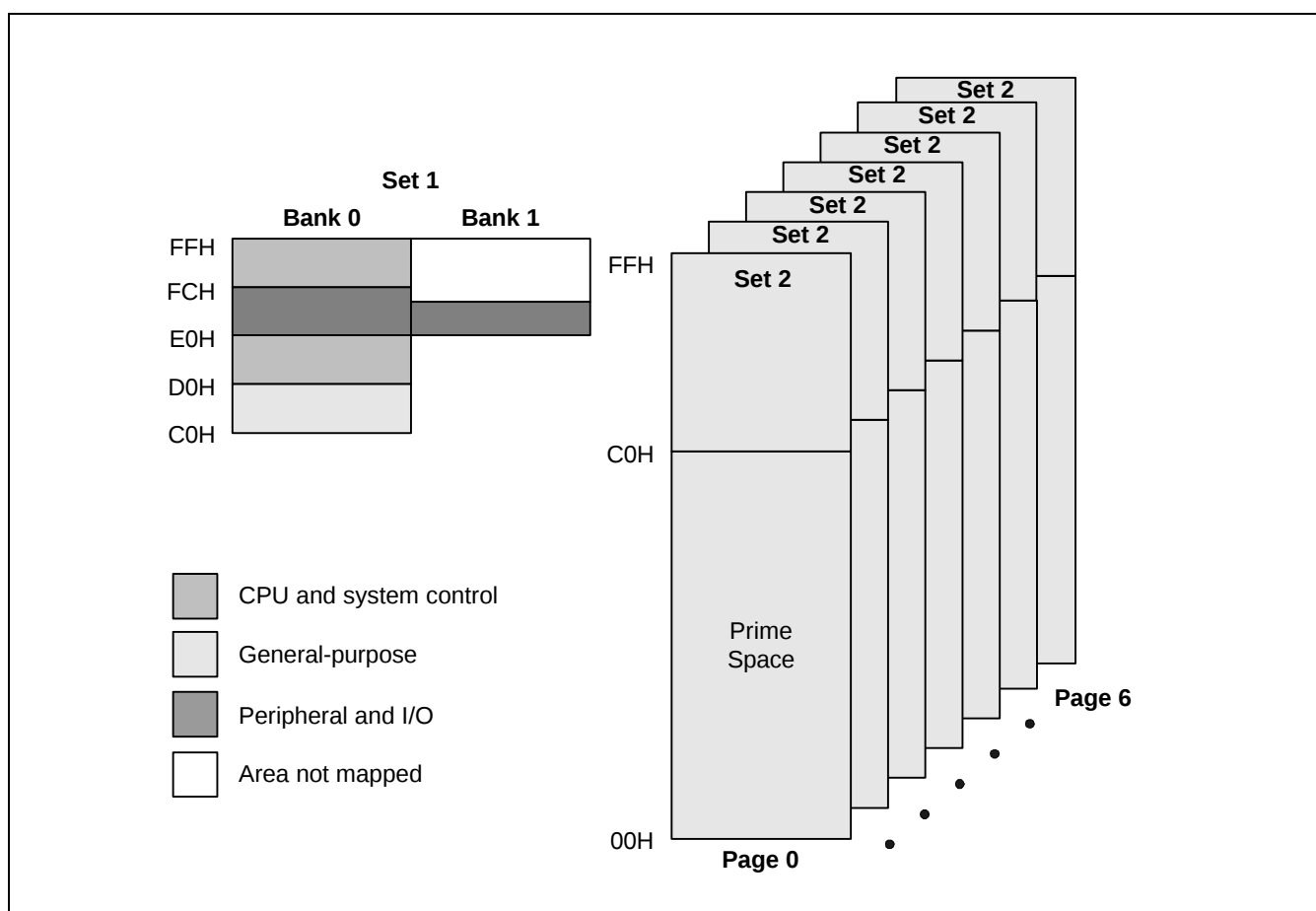
Figure 2-4. Map of Set 1, Set 2, and Prime Register Spaces
