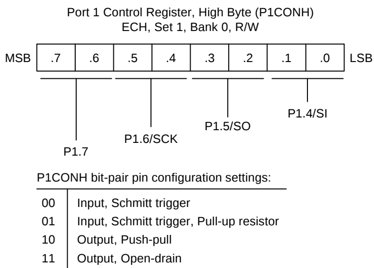
Figure 9-7. Port 1 High-Byte Control Register (P1CONH)
