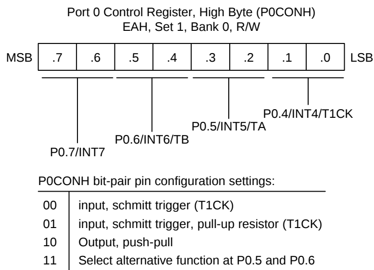
Figure 9-2. Port 0 Control Register (P0CONH)
