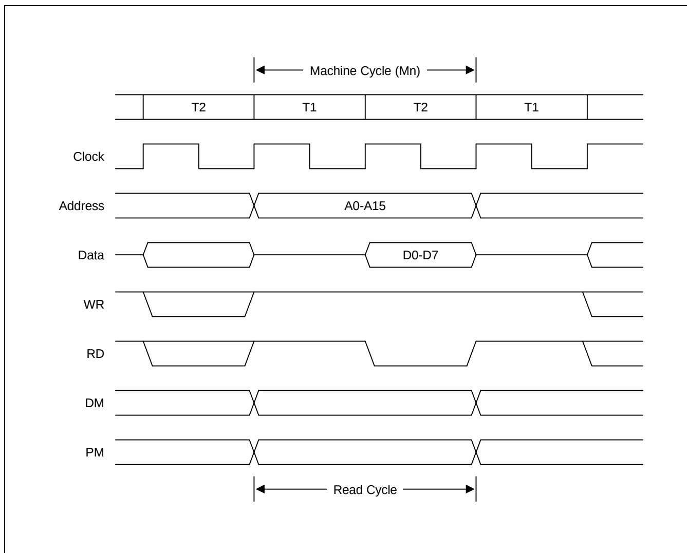
Figure 16-6. External Bus Read Cycle Timing Diagram
