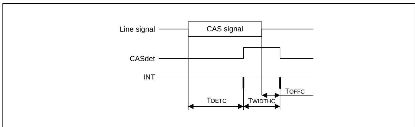
Figure 17-8. Waveform for CAS Timing Characteristics
