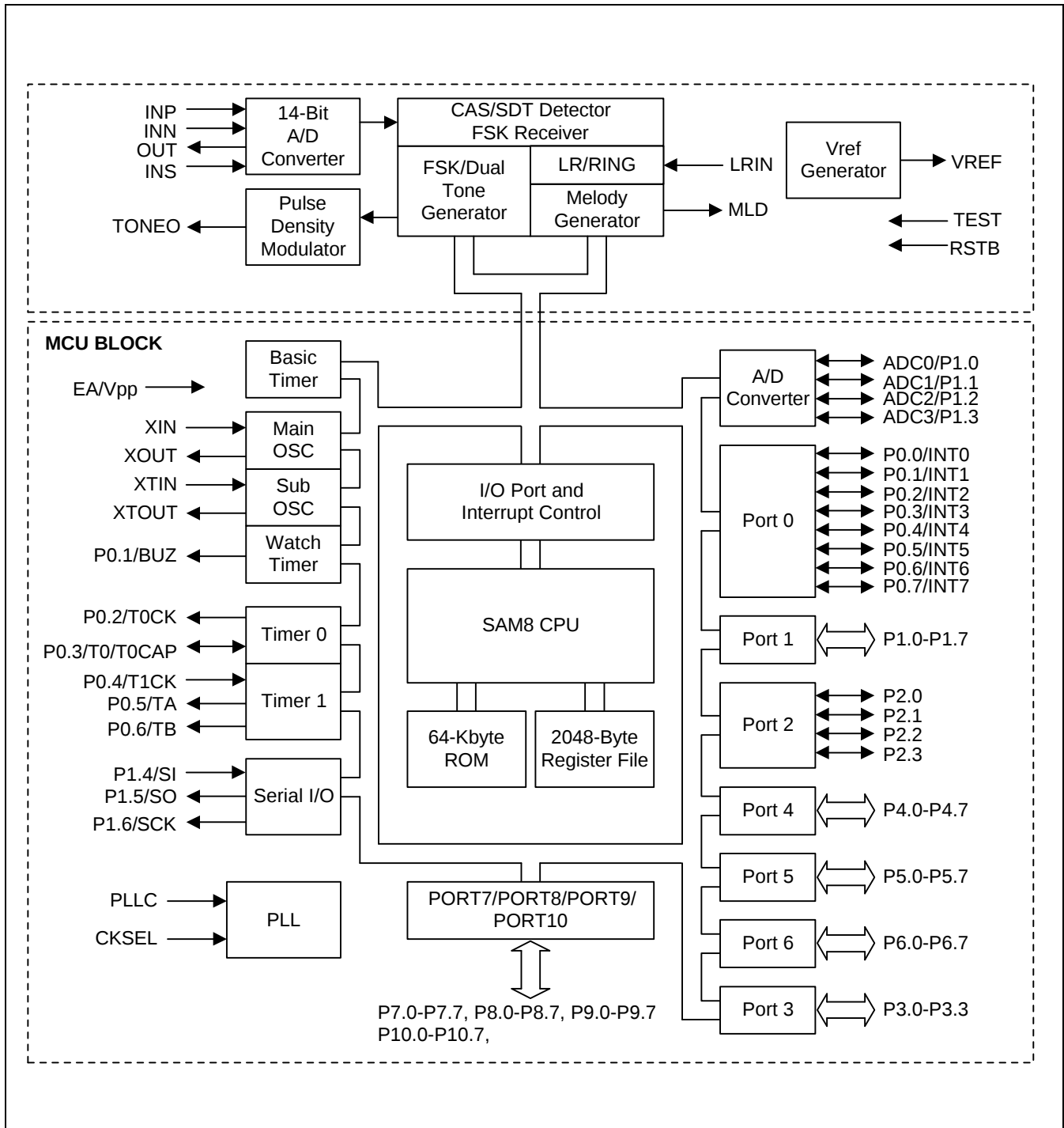
Figure 1-1. Block Diagram
