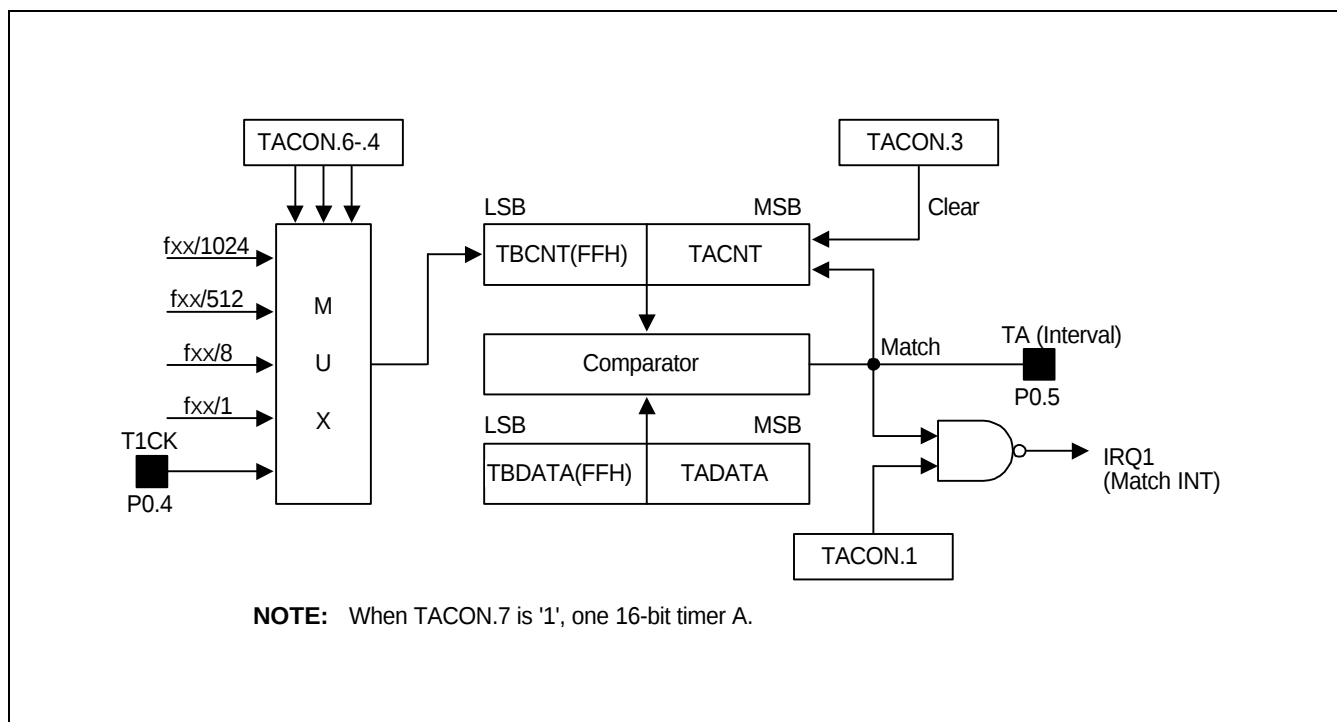
Figure 11-2. Timer 1 Functional Block Diagram
