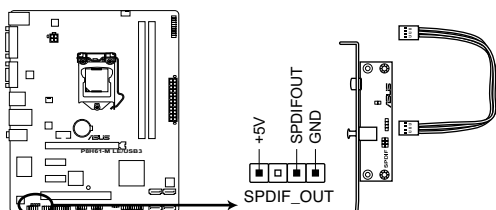
P8H61-M LE/USB3 Digital audio connector
