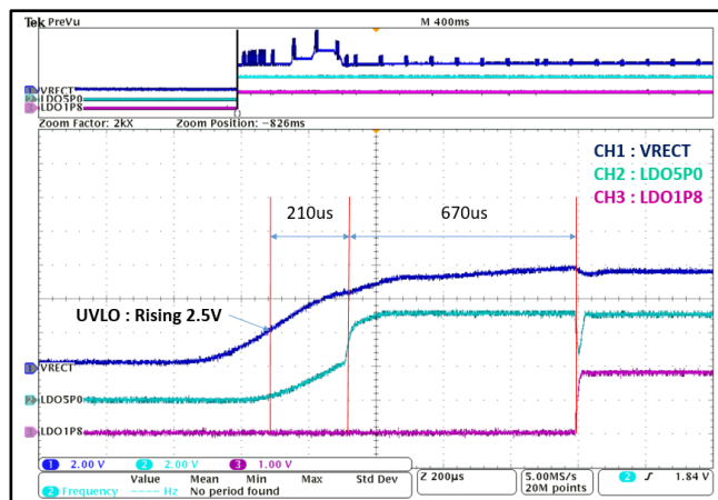
Figure 9. Initial Startup
