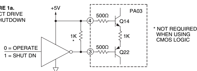
FIGURE 1b. HIGH VOLTAGE LOGIC INTERFACE
