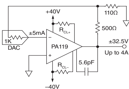
PA119 as a Fast Power Driver
