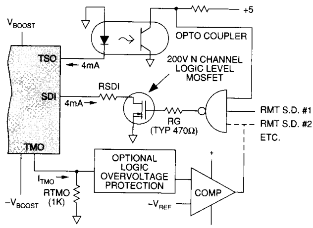
FIGURE 9. EXTERNALLY CONTROLLED THERMAL PROTECTION
