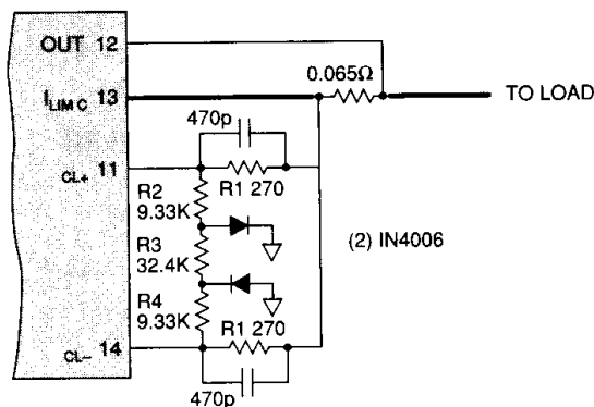
FIGURE 4. FOLDOVER CURRENT LIMIT
