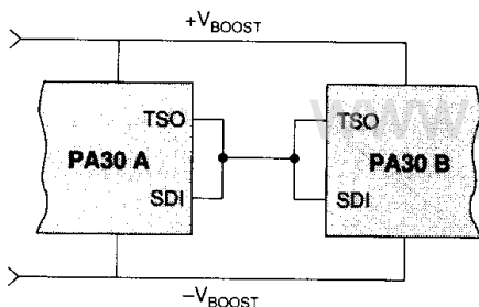
FIGURE 7. SIMPLE TSO/SDI LOOP
