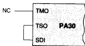
FIGURE 8. SIMPLE TSO/SDI LOOP
