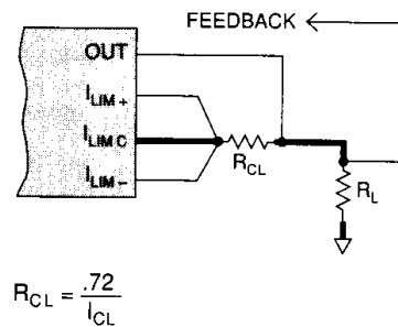
FIGURE 1. I_{LIMIT} WHERE I_{CL+} = I_{CL-}
