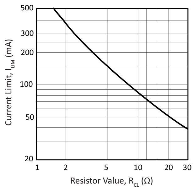
Figure 14: Current Limit
