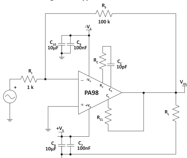
Figure 1: Typical Connections
