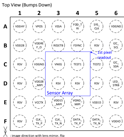
Figure 6. PAC7640LT CSP Package Overview
