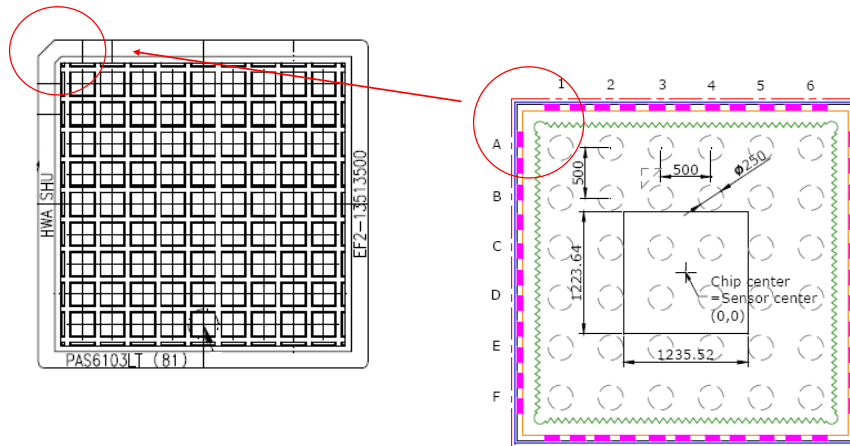
Figure 7. IC Orientation
